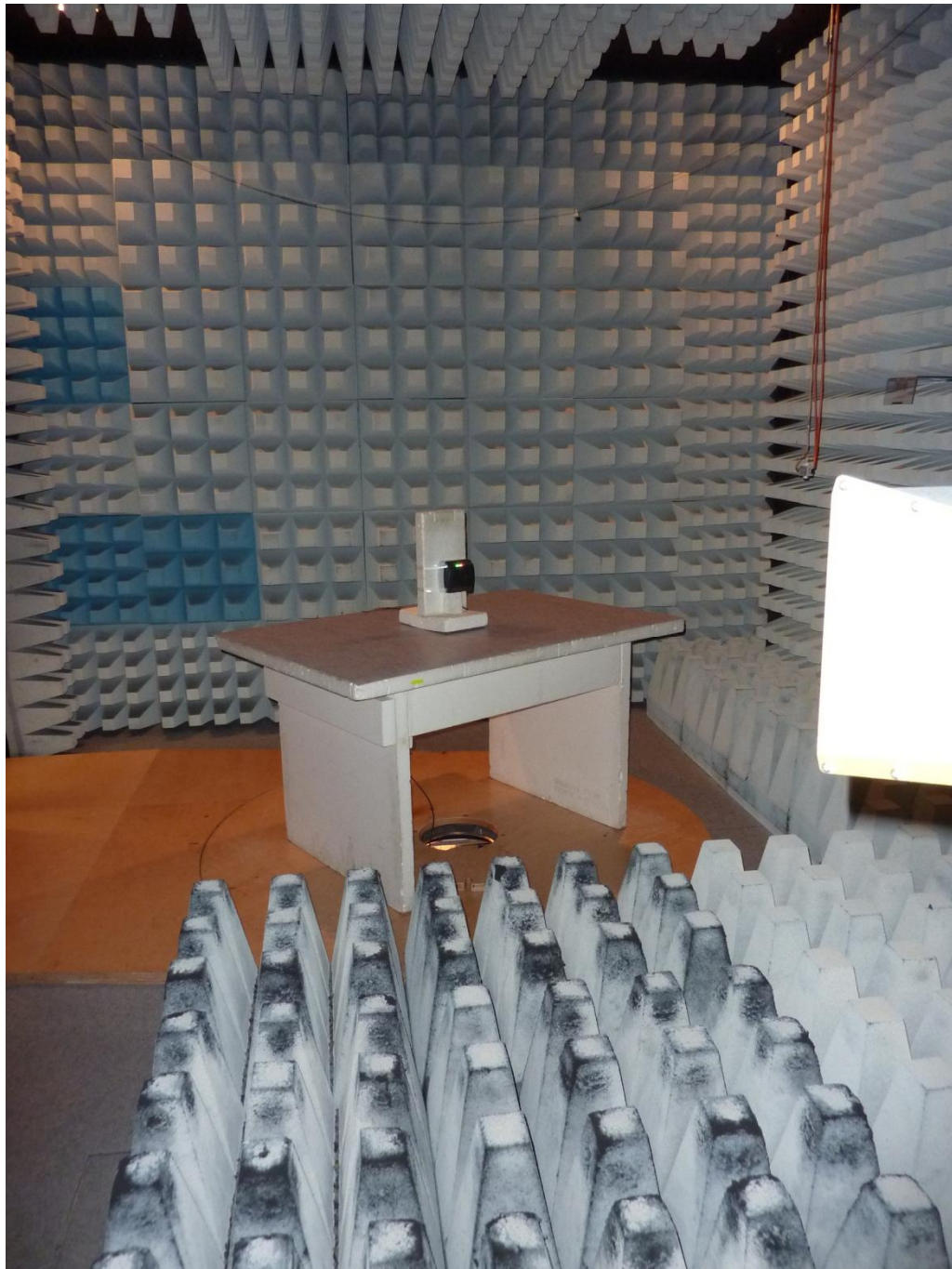
142568_d.JPG: TN902-Q120L130-H1147, test set-up fully anechoic chamber
