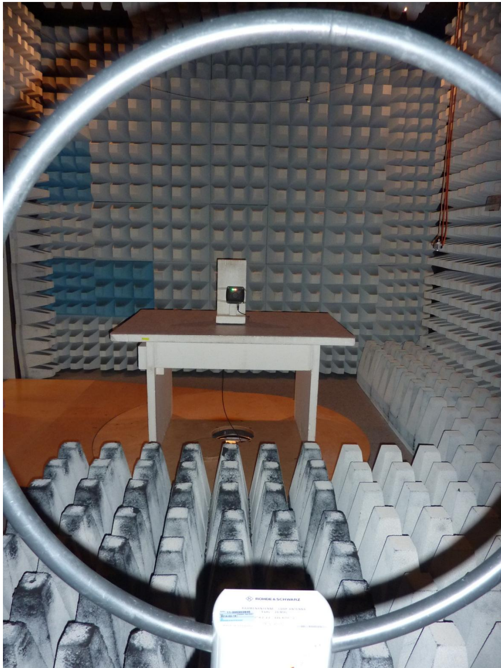
142568_e.JPG: TN902-Q120L130-H1147, test set-up fully anechoic chamber
