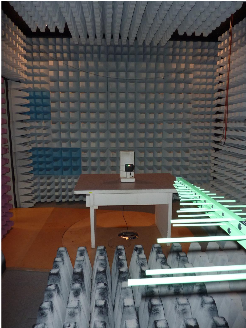
142568_a.JPG: TN902-Q120L130-H1147, test set-up fully anechoic chamber
