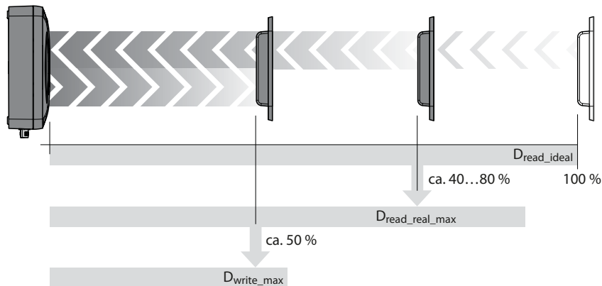
Figure 10: Possible read/write distances
