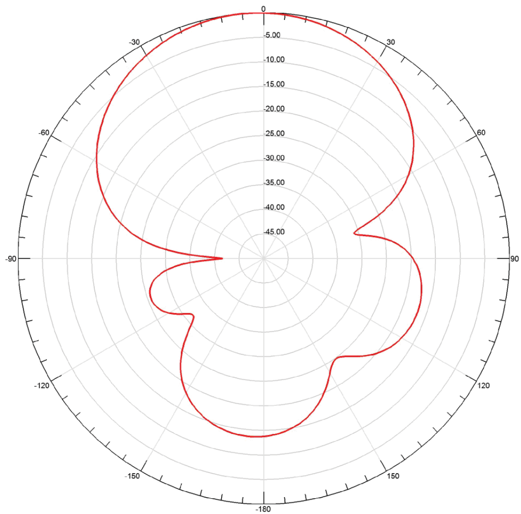
Figure36: Elevation section, horizontal polarization
