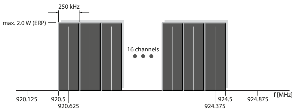
Figure 23: Frequency ranges in China, Frequency hopping procedure
