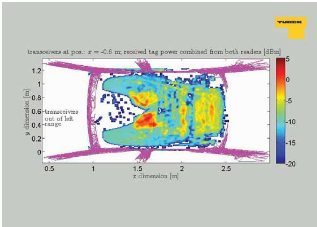
Figure 9: Example of a Ray Tracer field strength simulation
