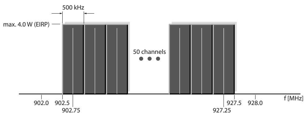
Figure 22: Frequency ranges in the USA, frequen- cy hopping proce- dure
