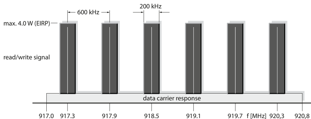
Figure 21: Frequency ranges in Korea, Frequency hopping procedure
