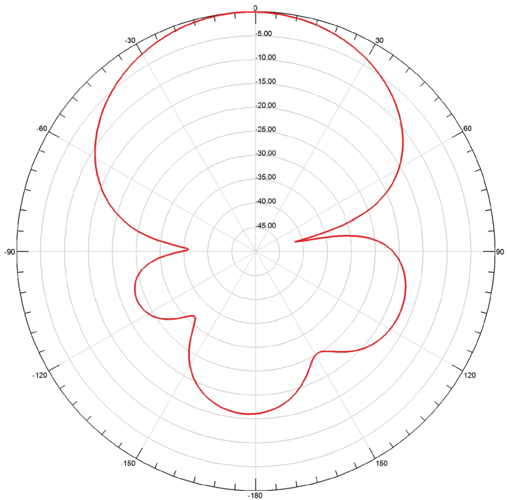
Figure34: Azimuth section, horizontal polarization
