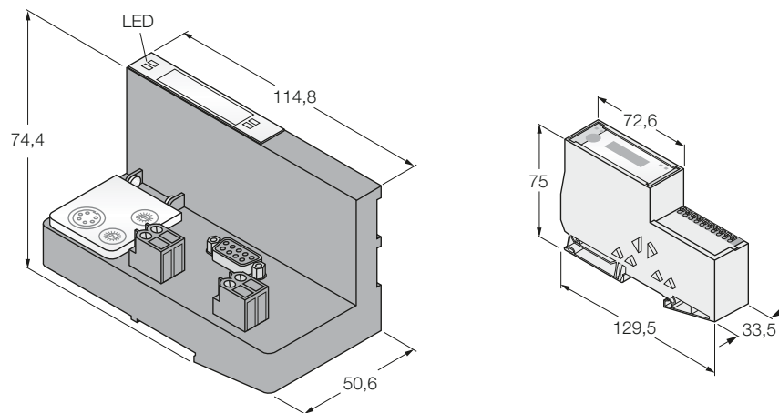
Figure 1: Gateway for BL20 (example PROFIBUS-DP): Standard gateway (left) and ECONOMY gate- way (right)
