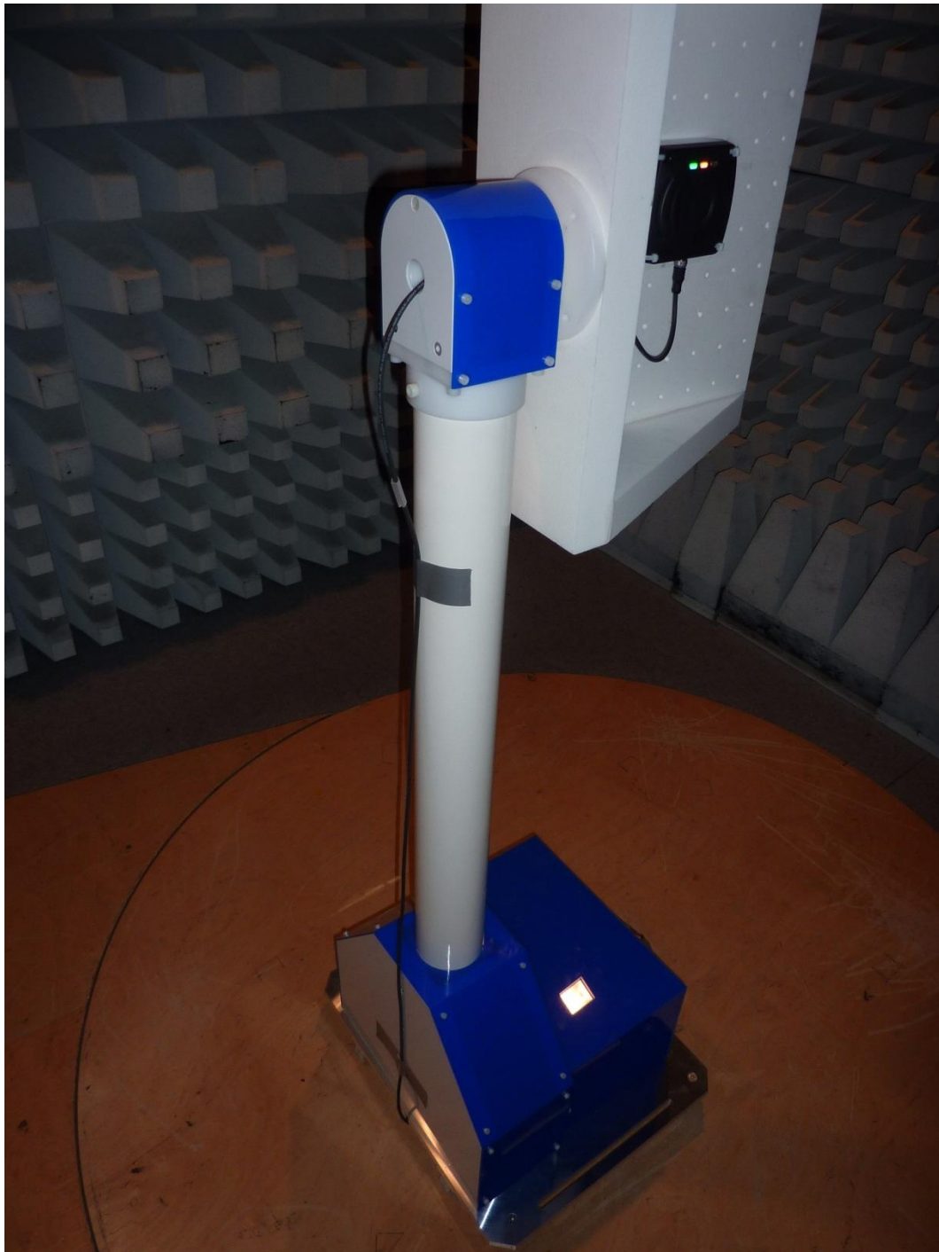
153142_e.JPG: TN902-Q120L130H1147, test set-up fully anechoic chamber
