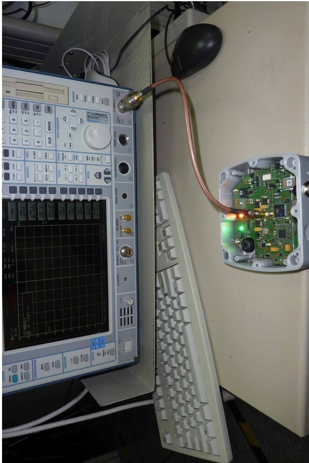
153142_i.JPG: TN902-Q120L130H1147, test set-up conducted measurements
