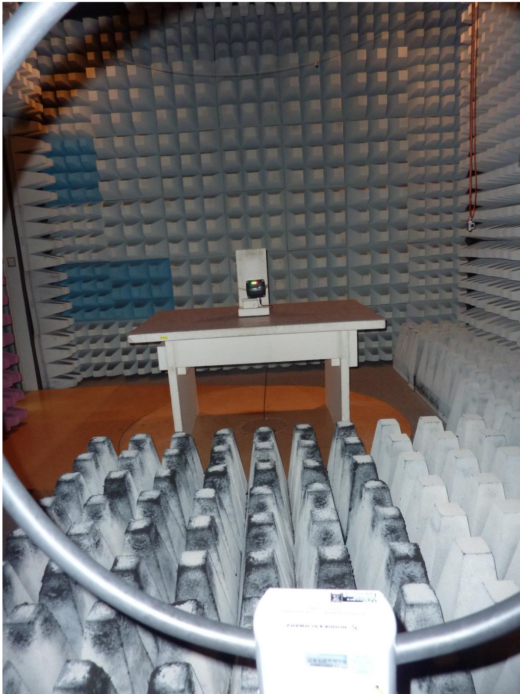
153142_b.JPG: TN902-Q120L130H1147, test setup fully anechoic chamber
