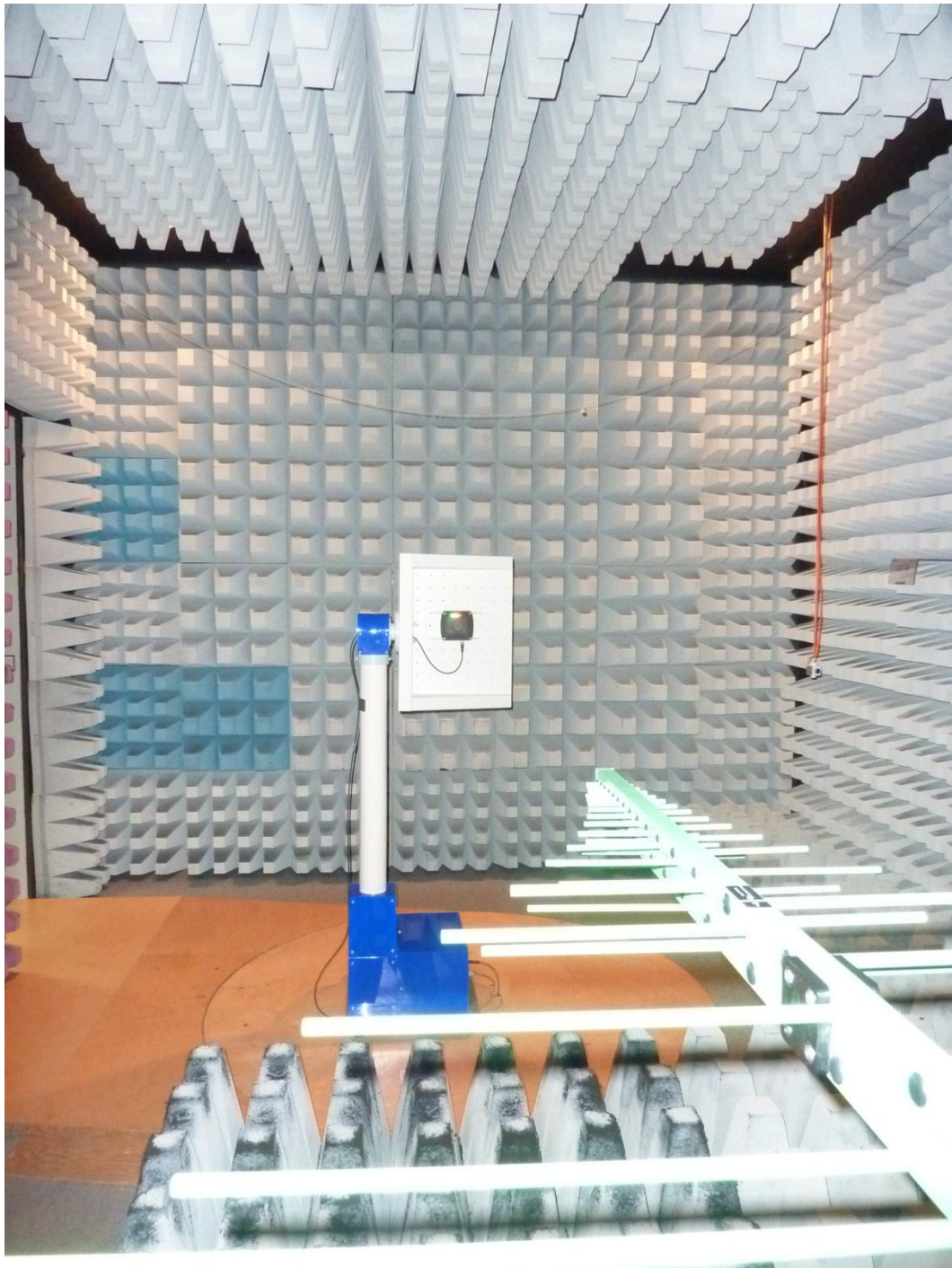
153142_c.JPG: TN902-Q120L130H1147, test set-up fully anechoic chamber
