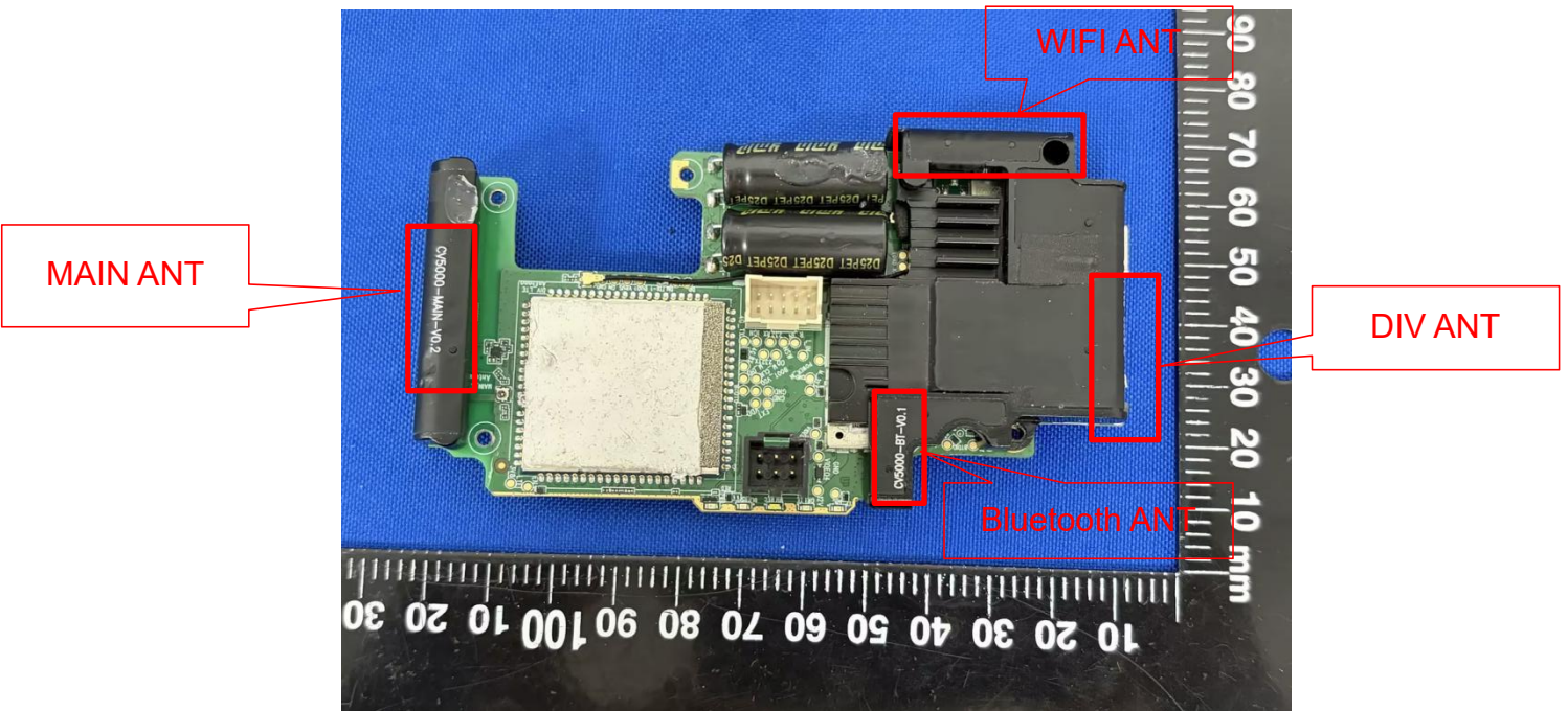
SECONDARY BOARD 1 TOP VIEW (WITH SHIELDING)
