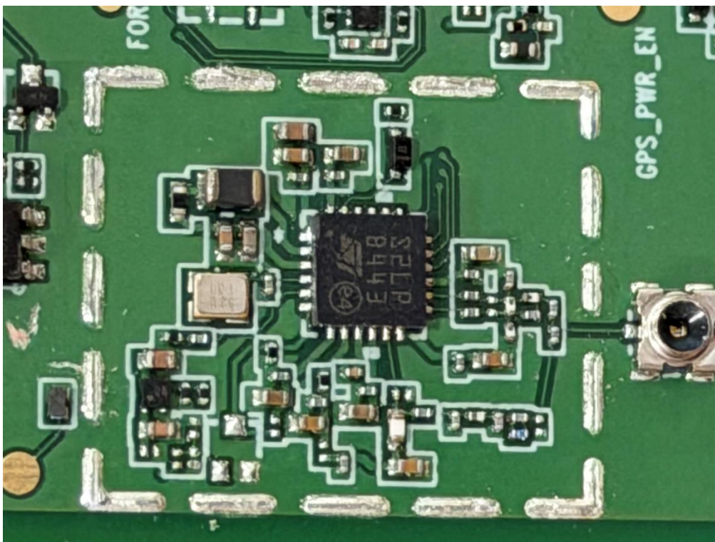
Photo 10: Internal View for 433MHz Chip
