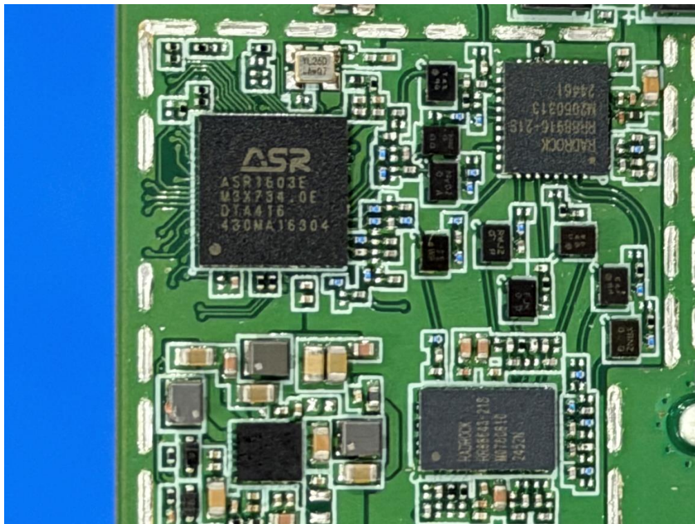
Photo 8: Internal View for 2G/4G Chip
