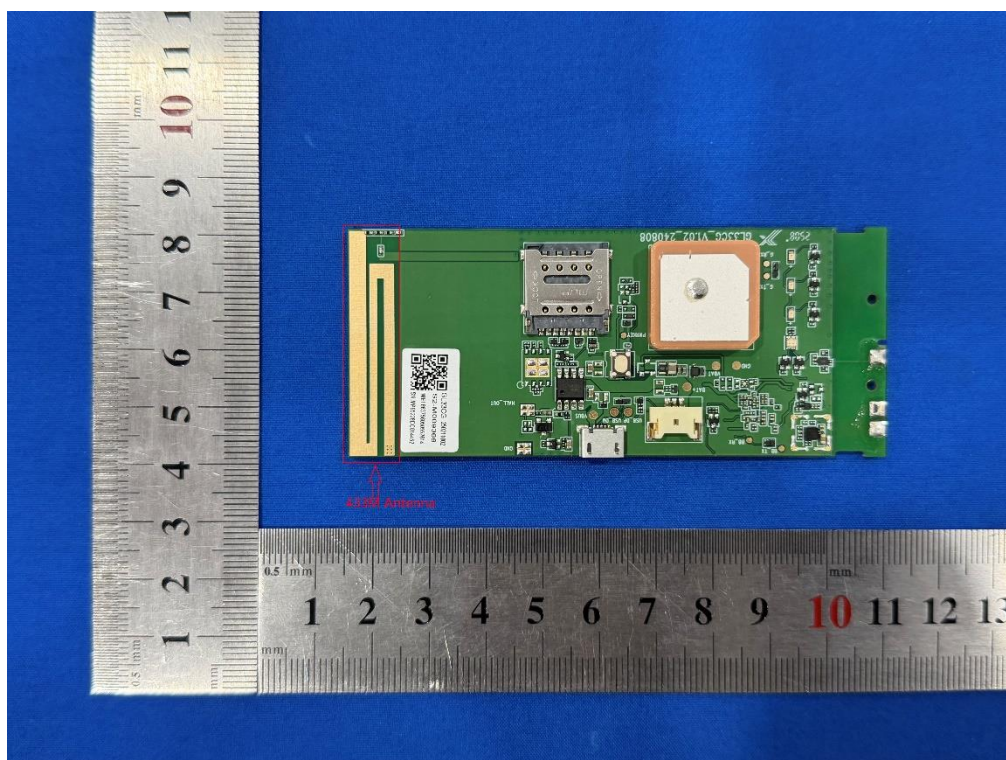
Photo 13: Internal View for 433MHz Antenna
