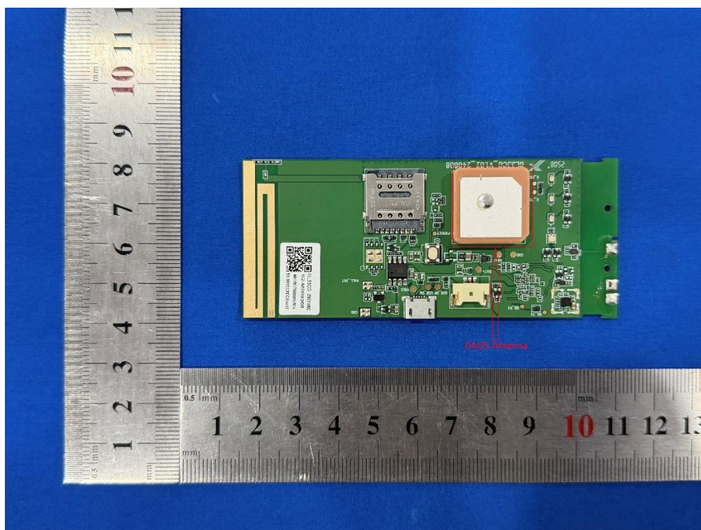
Photo 14: Internal View for GNSS Antenna
