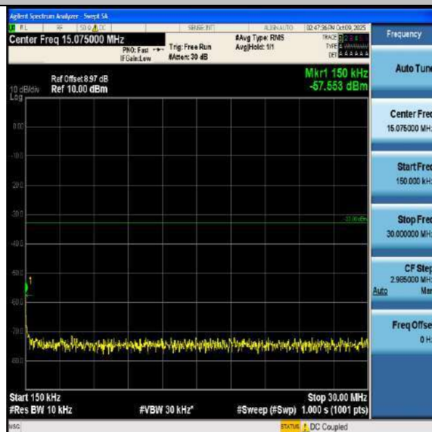
Band2-5MHz-QPSK-19175-1RB#0-0.15~30-PASS
