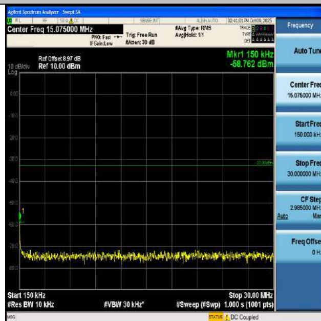
Band2-5MHz-QPSK-18625-1RB#0-0.15~30-PASS
