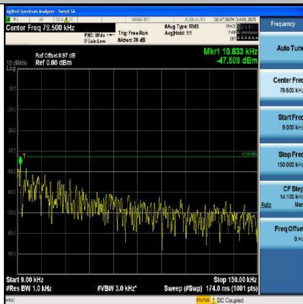
Band2-5MHz-QPSK-19175-1RB#0-0.009~0.15-PASS
