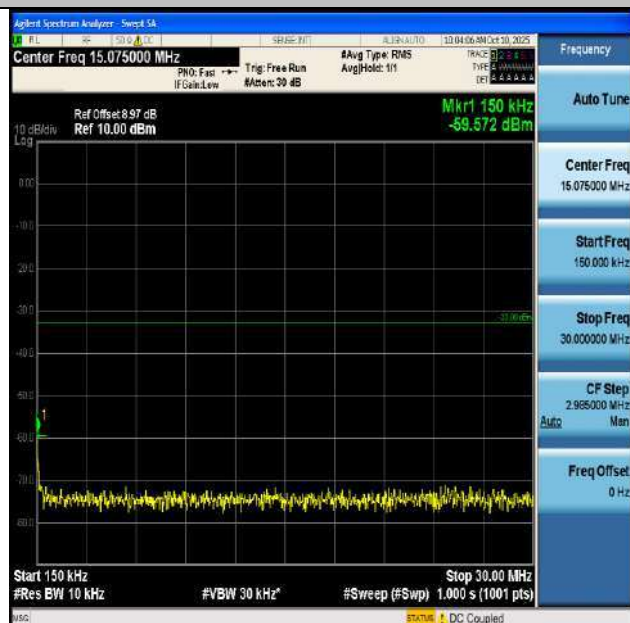
Band2-10MHz-QPSK-18900-1RB#0-0.15~30-PASS
