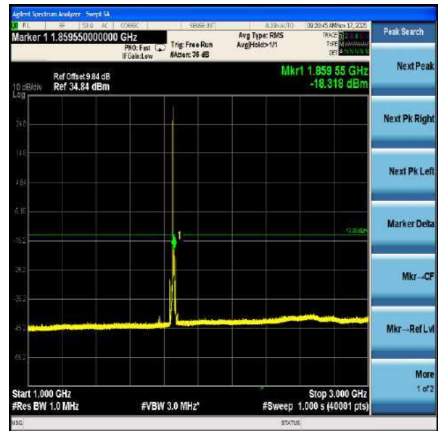
Band2-10MHz-QPSK-18650-1RB#0-1000~3000-PASS
