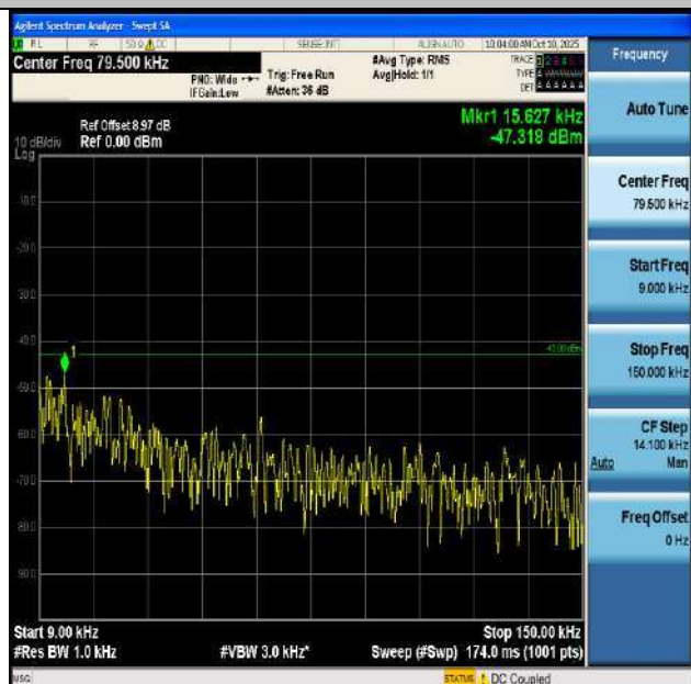
Band2-10MHz-QPSK-18900-1RB#0-0.009~0.15-PASS
