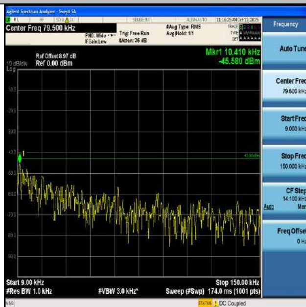
Band2-15MHz-QPSK-18900-1RB#0-0.009~0.15-PASS
