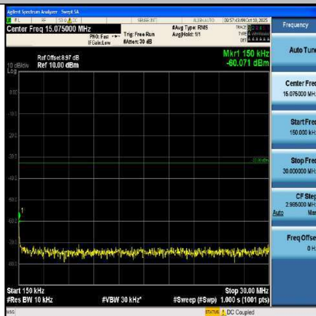
Band2-10MHz-QPSK-18650-1RB#0-0.15~30-PASS
