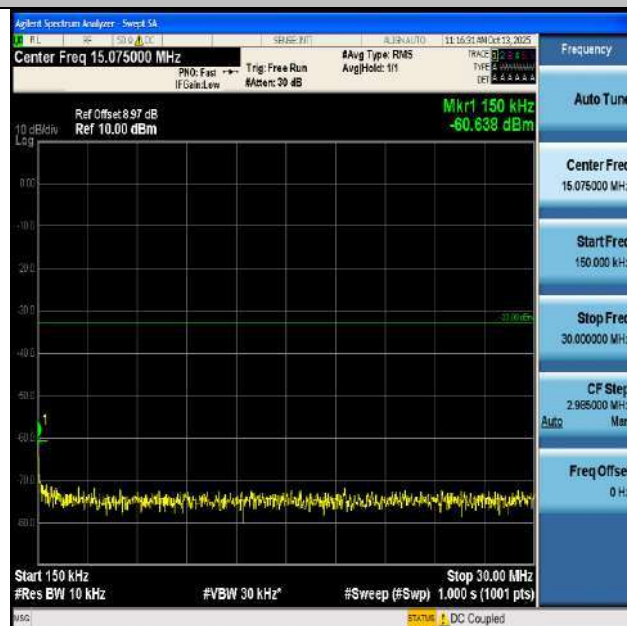
Band2-15MHz-QPSK-18900-1RB#0-0.15~30-PASS
