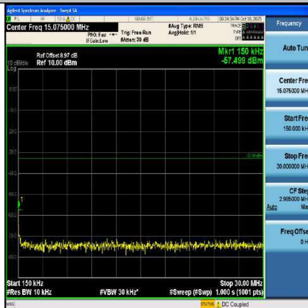
Band2-20MHz-QPSK-18700-1RB#0-0.15~30-PASS
