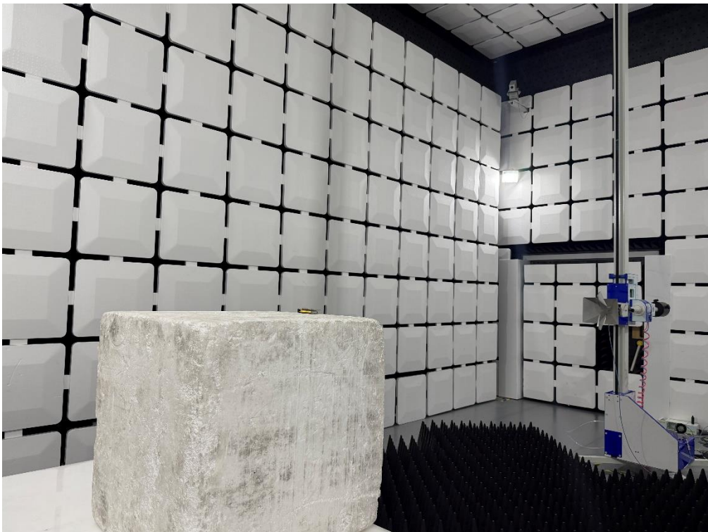
Description: 433M Radiated Emission Test Setup for Above 1GHz
