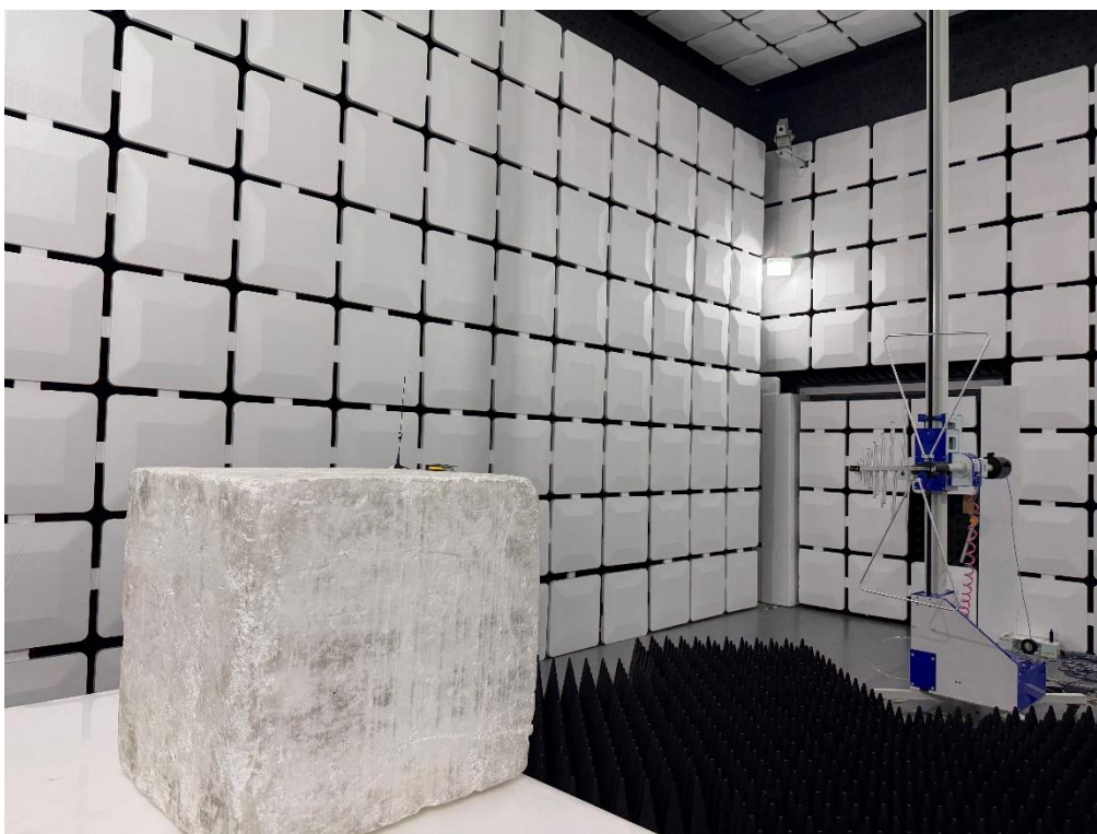
Description: 2G/4G Radiated Emission Test Setup for Below 1GHz
