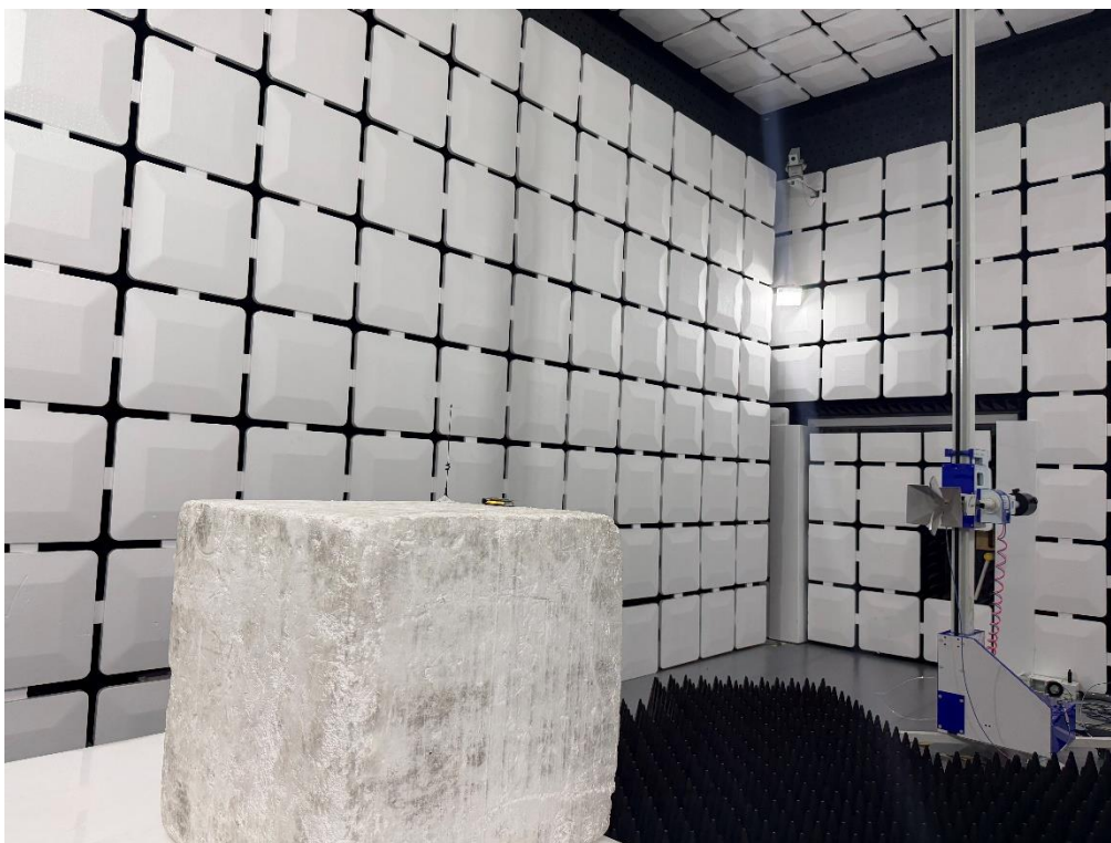
Description: 2G/4G Radiated Emission Test Setup for Above 1GHz
