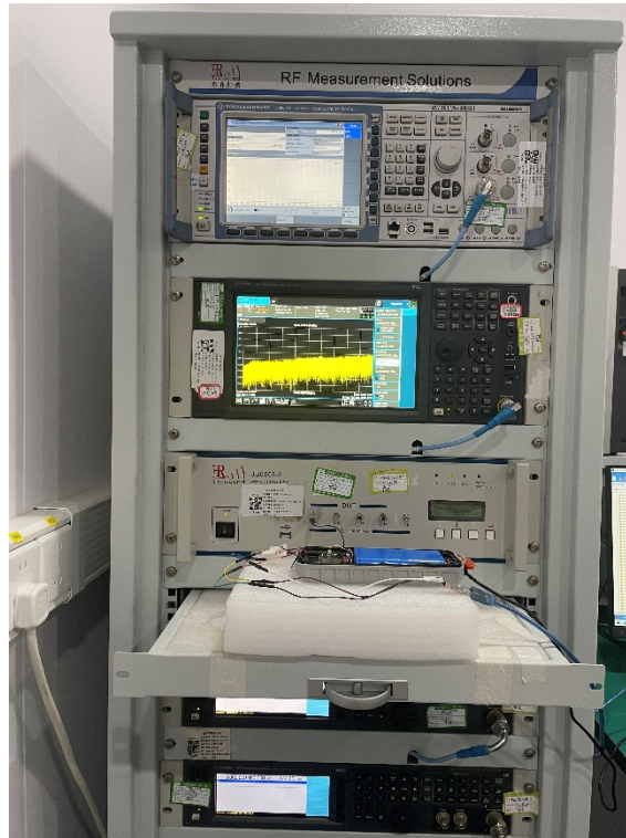
Description: Conducted Test Setup
