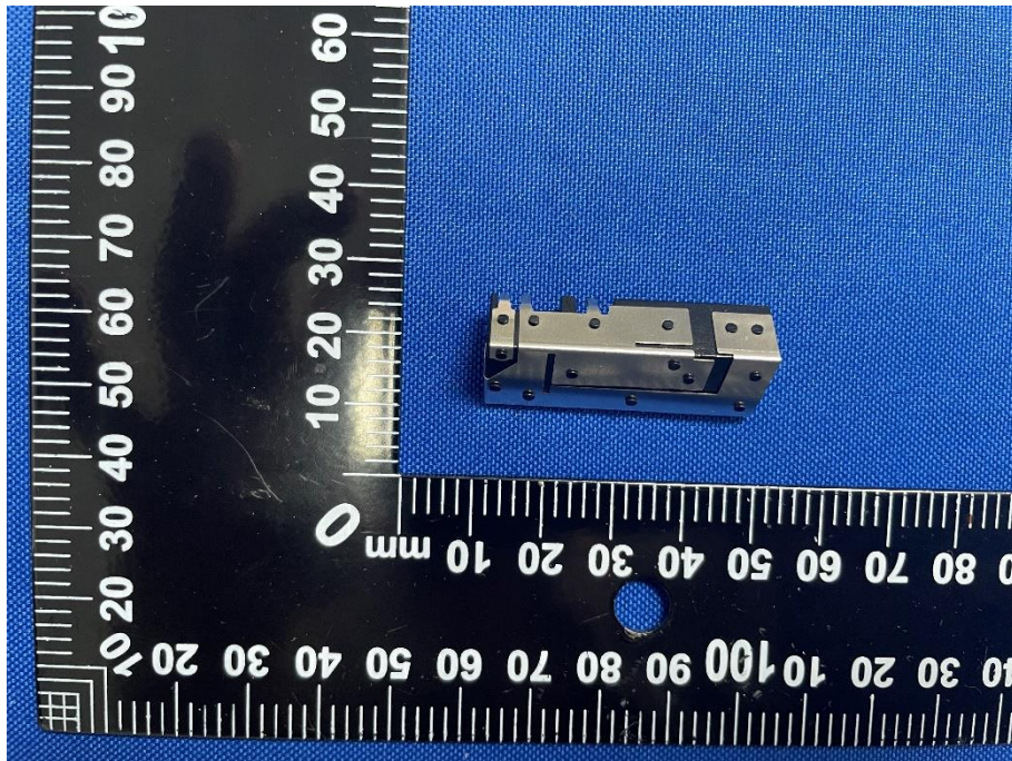
WWAN ANTENNA TOP VIEW
