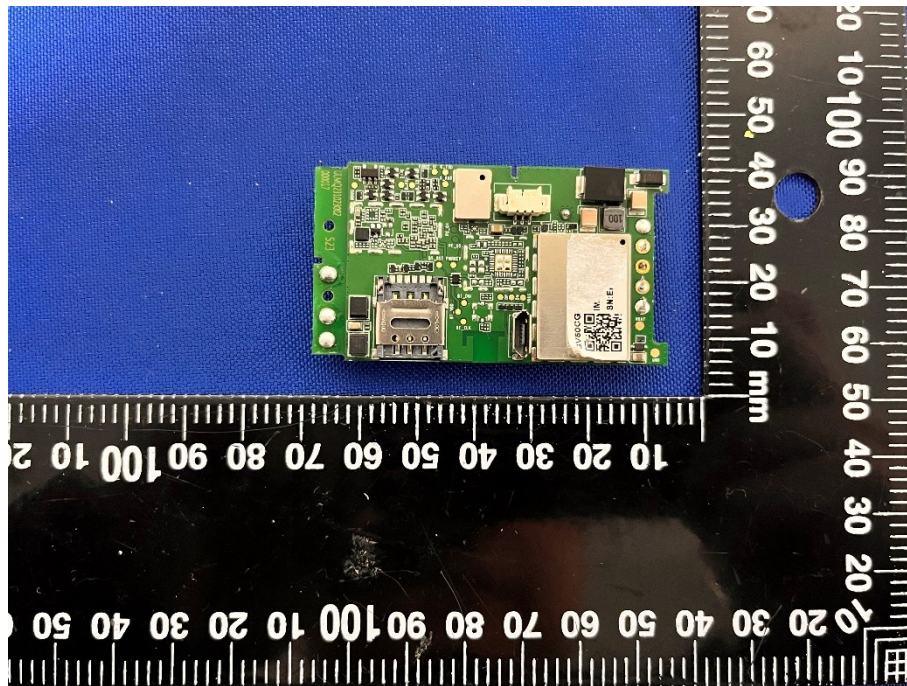
BOTTOM VIEW OF MAINBOARD (WITH SHIELD COVER)
