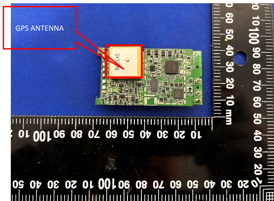
TOP VIEW OF MAINBOARD (WITHOUT SHIELD COVER)
