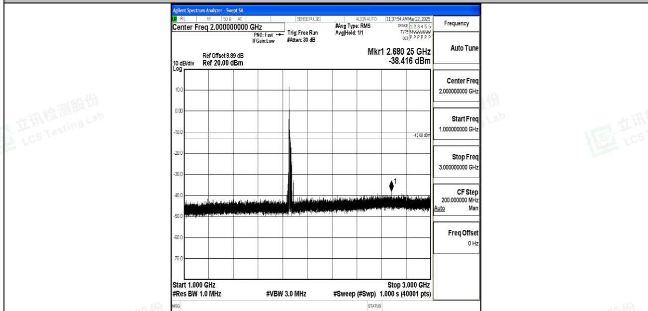
Band2_20MHz_16QAM_18700_1RB#0_1000~3000_1000~3000
