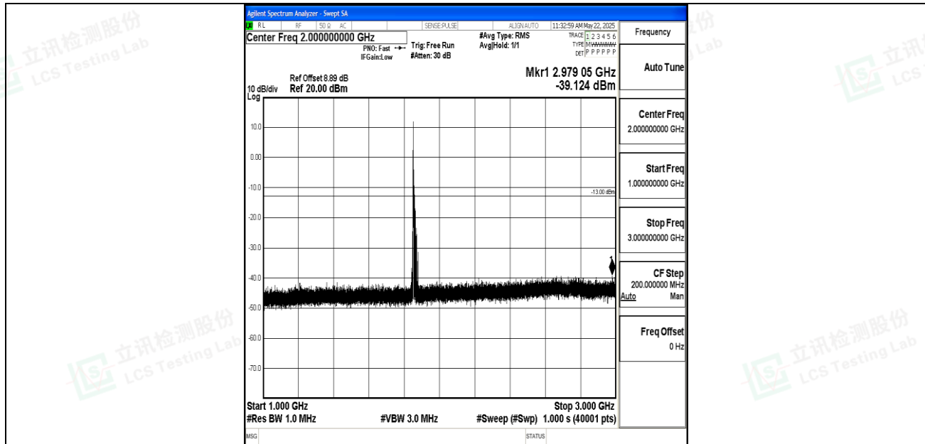
Band2_15MHz_QPSK_18675_1RB#0_1000~3000_1000~3000
