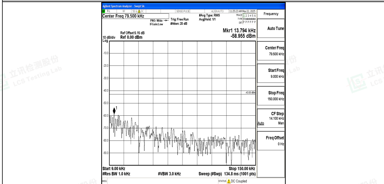
Band2_5MHz_QPSK_18900_1RB#0_0.009~0.15_0.009~0.15
