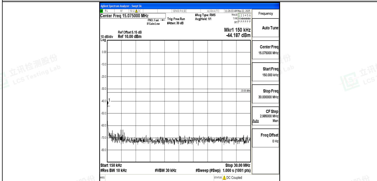
Band2_5MHz_16QAM_18900_1RB#0_0.15~30_0.15~30
