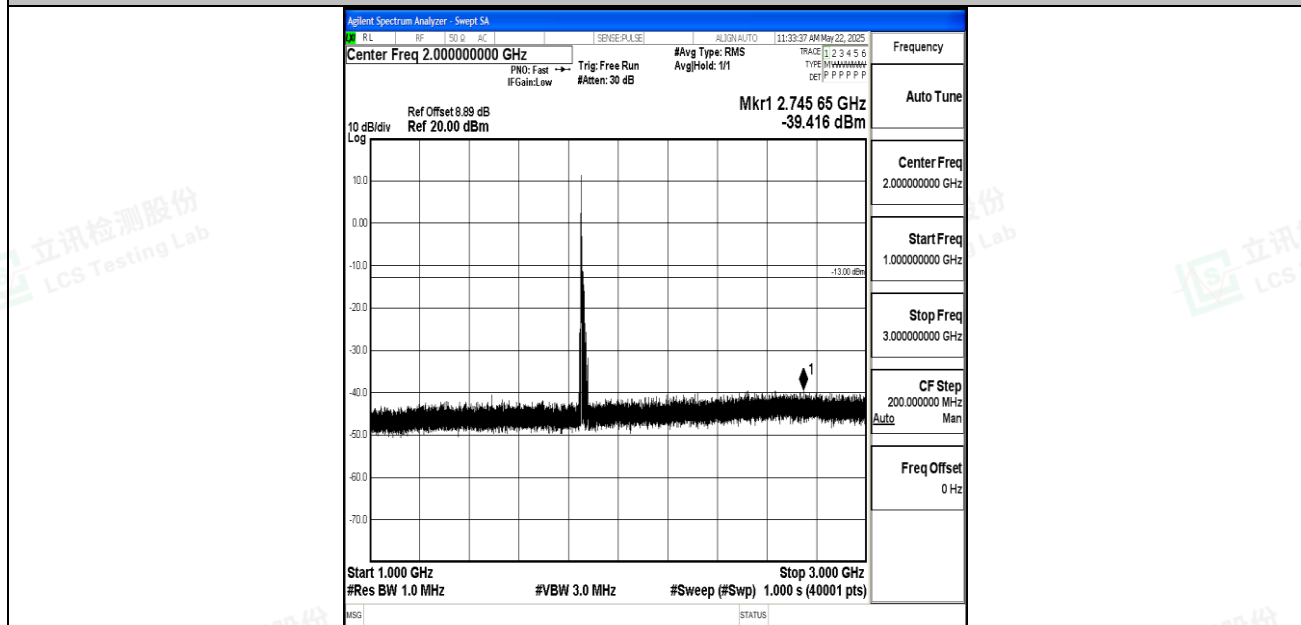
Band2_15MHz_16QAM_18675_1RB#0_1000~3000_1000~3000
