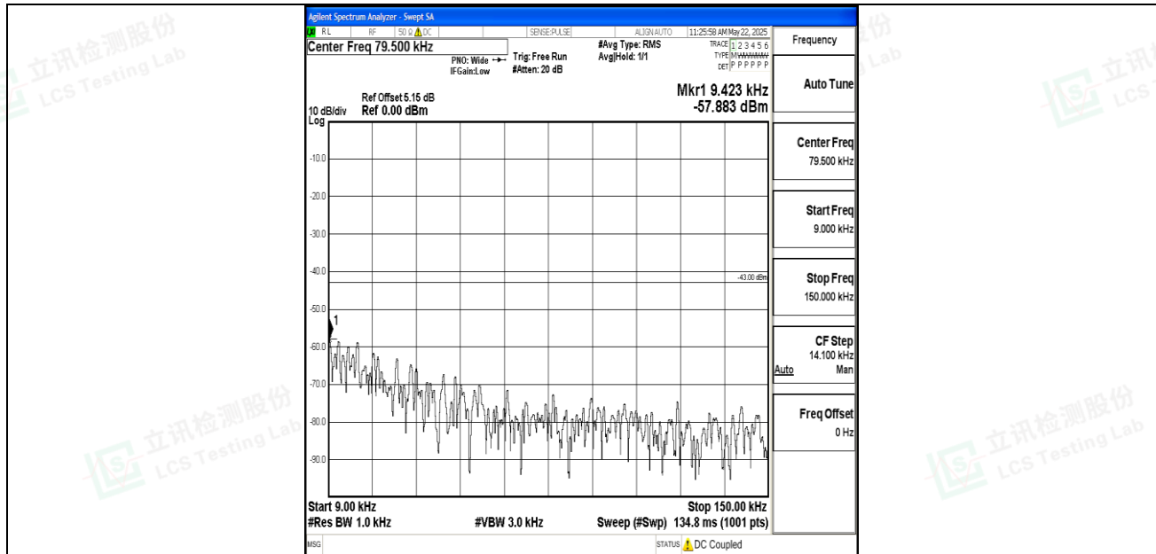
Band2_5MHz_16QAM_18900_1RB#0_0.009~0.15_0.009~0.15
