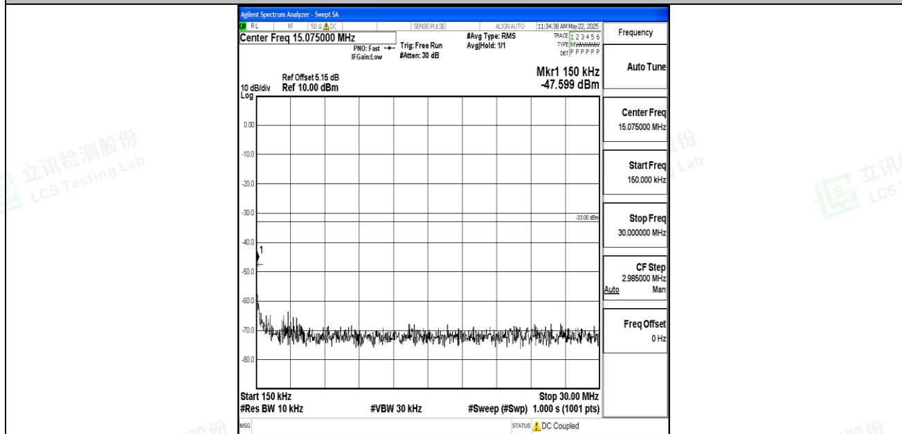
Band2_15MHz_16QAM_18900_1RB#0_0.15~30_0.15~30
