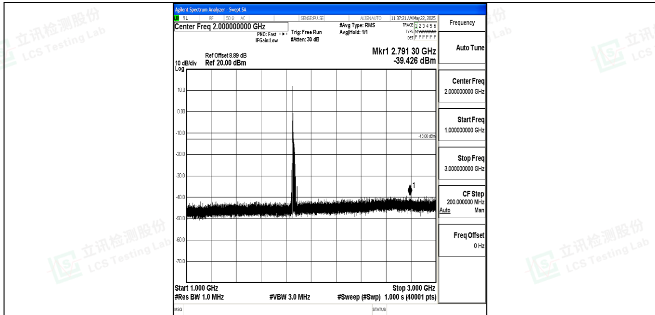
Band2_20MHz_QPSK_18700_1RB#0_1000~3000_1000~3000
