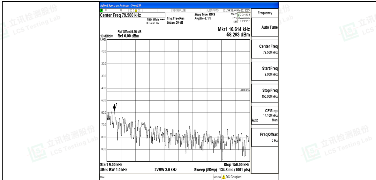
Band2_15MHz_16QAM_18900_1RB#0_0.009~0.15_0.009~0.15
