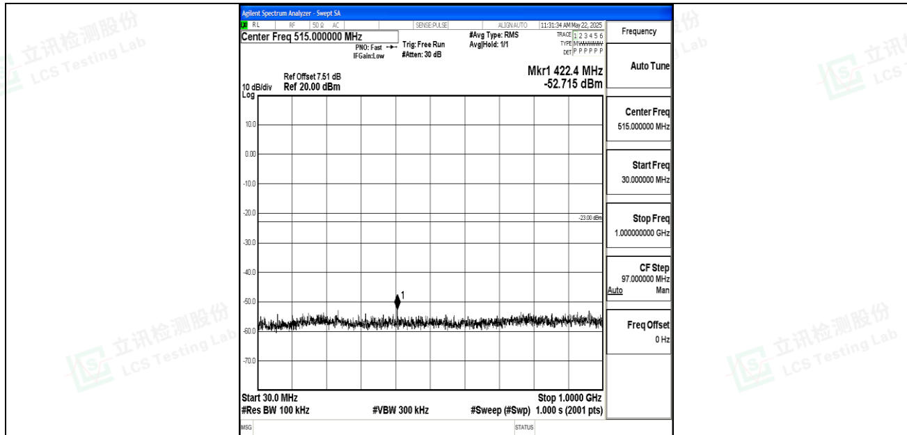
Band2_10MHz_16QAM_19150_1RB#0_30~1000_30~1000
