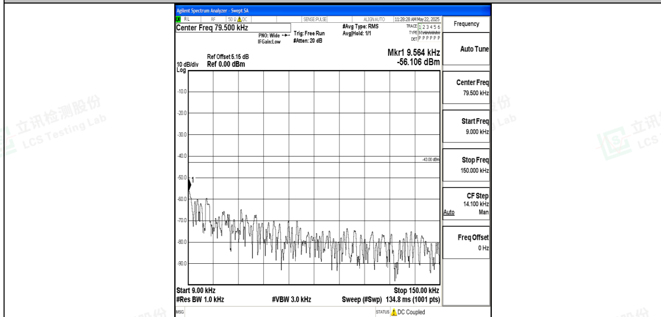
Band2_10MHz_QPSK_18650_1RB#0_0.009~0.15_0.009~0.15
