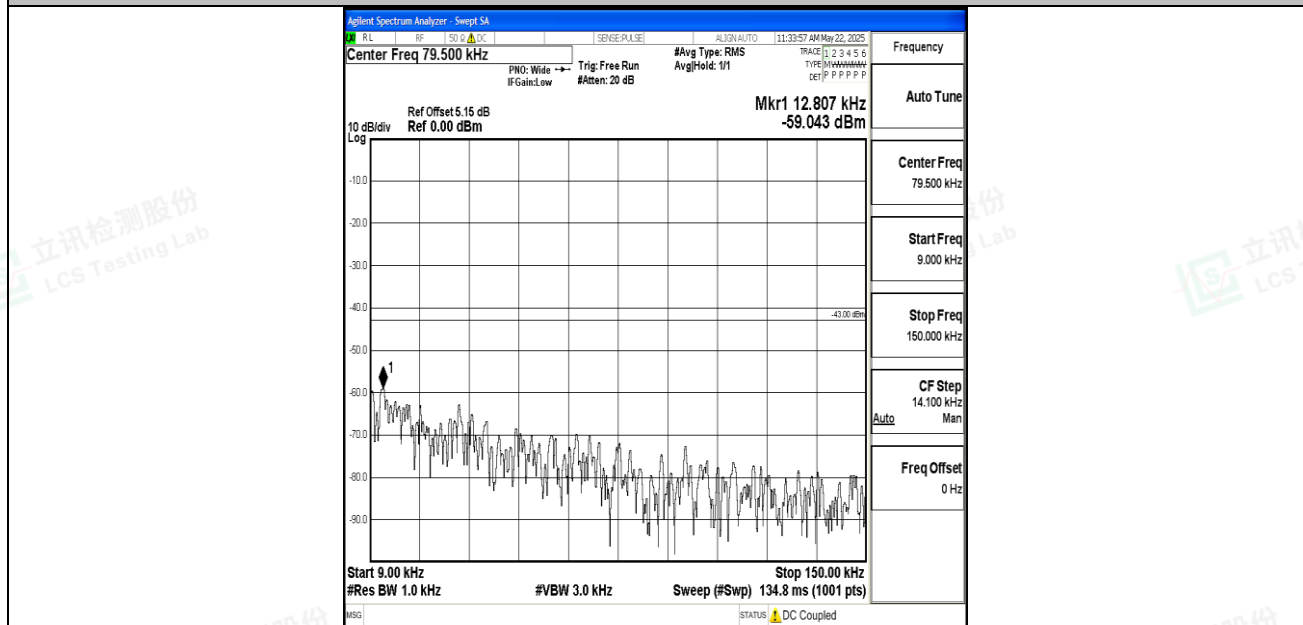
Band2_15MHz_QPSK_18900_1RB#0_0.009~0.15_0.009~0.15
