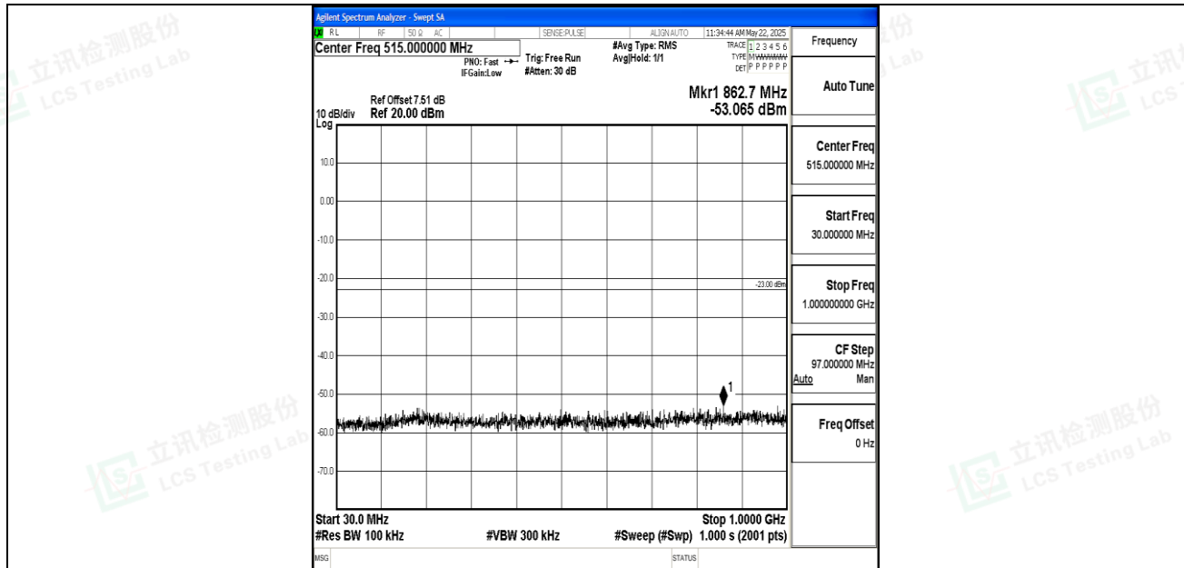
Band2_15MHz_16QAM_18900_1RB#0_30~1000_30~1000
