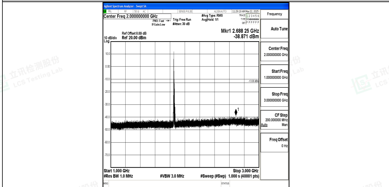
Band2_10MHz_16QAM_18650_1RB#0_1000~3000_1000~3000
