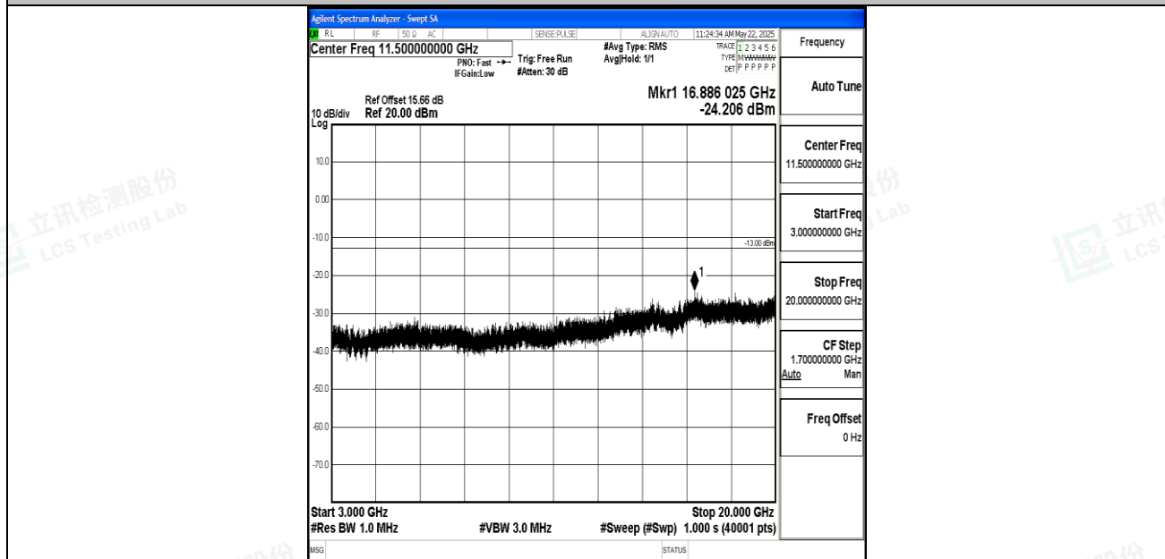
Band2_5MHz_QPSK_18625_1RB#0_3000~20000_3000~20000
