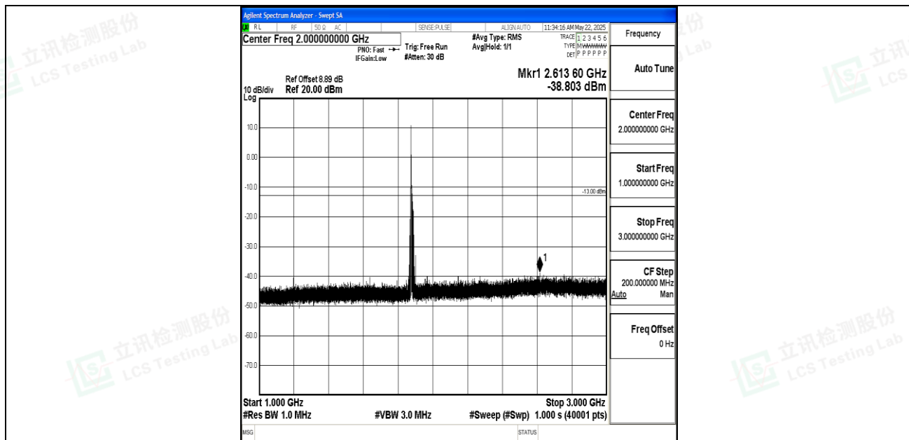
Band2_15MHz_QPSK_18900_1RB#0_1000~3000_1000~3000
