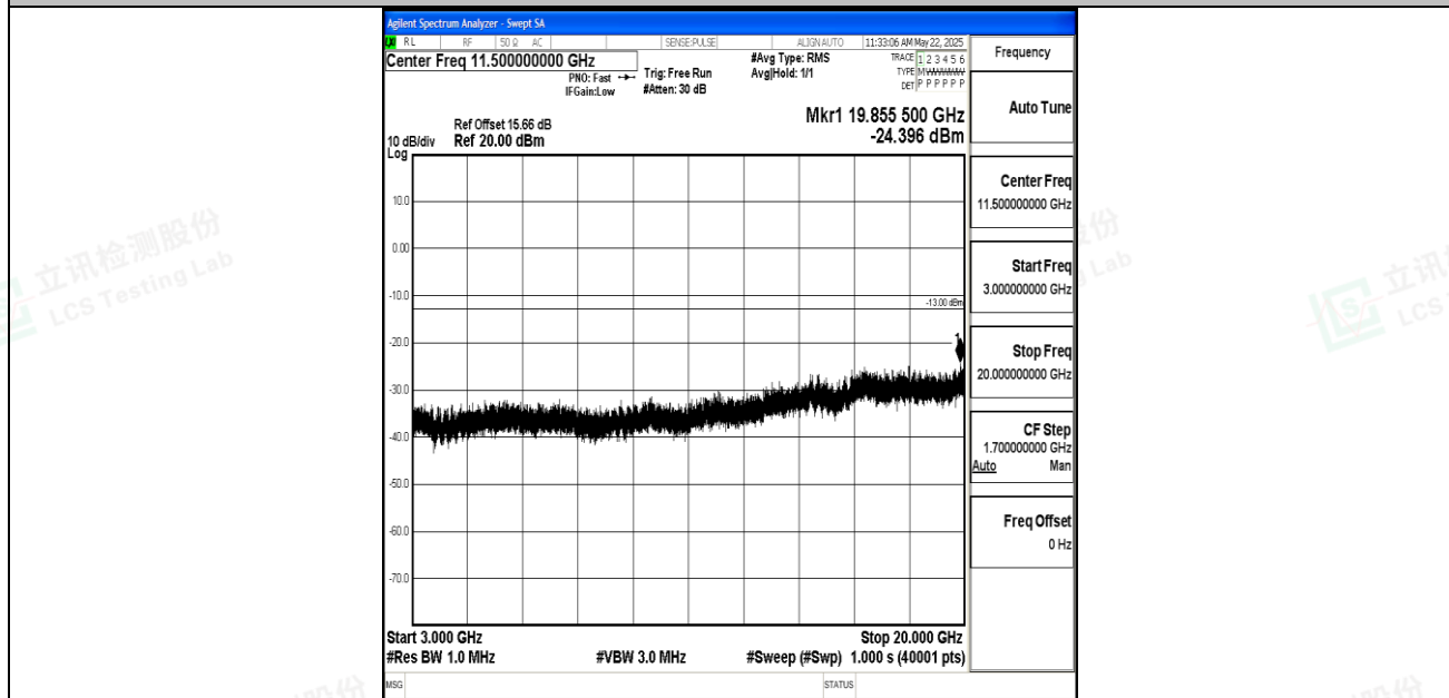
Band2_15MHz_QPSK_18675_1RB#0_3000~20000_3000~20000
