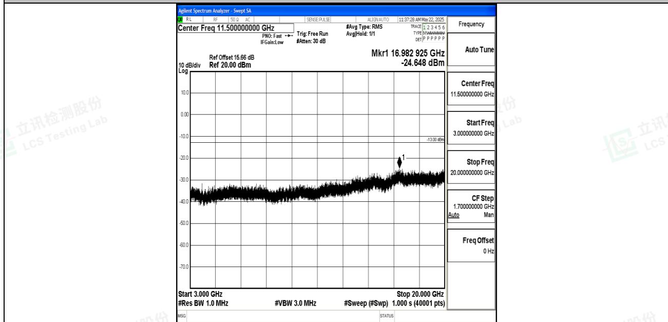
Band2_20MHz_QPSK_18700_1RB#0_3000~20000_3000~20000
