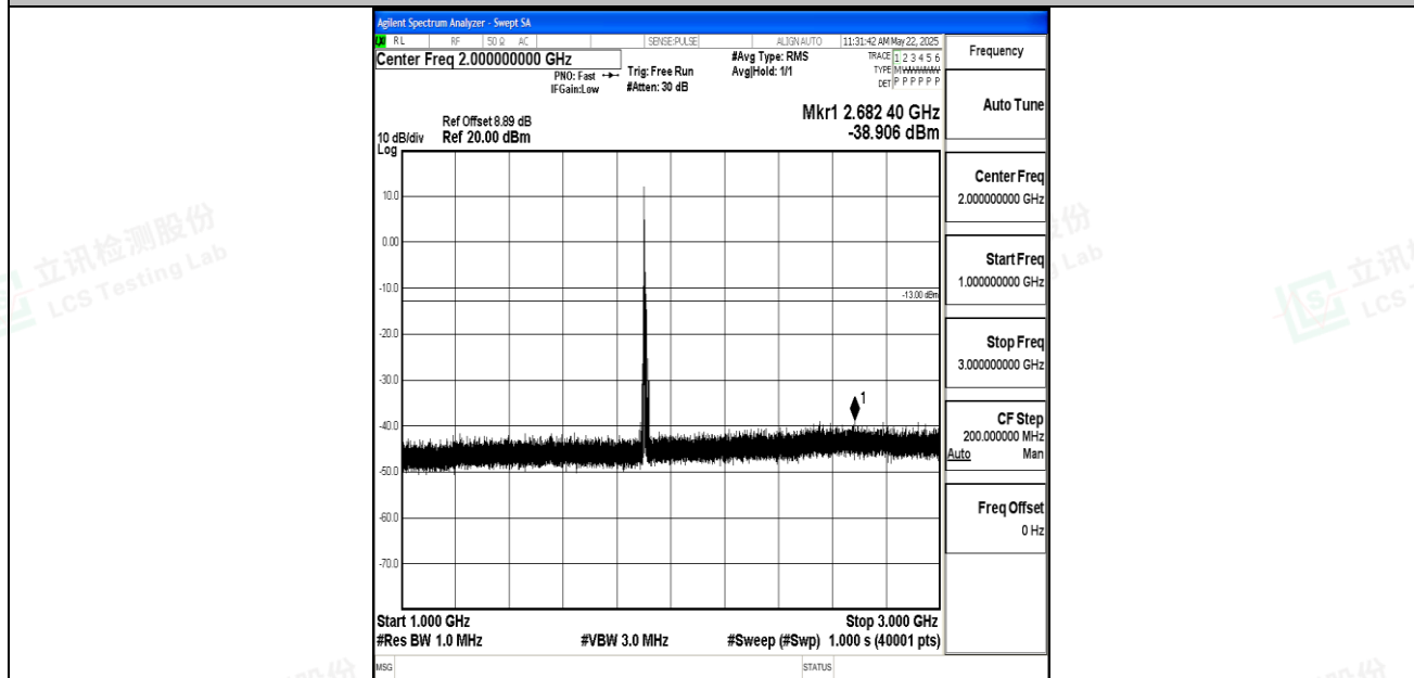
Band2_10MHz_16QAM_19150_1RB#0_1000~3000_1000~3000
