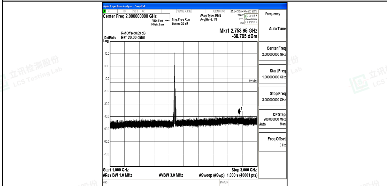
Band2_15MHz_16QAM_18900_1RB#0_1000~3000_1000~3000
