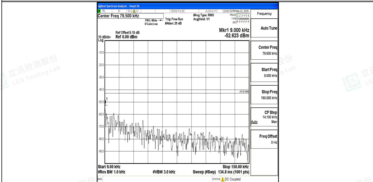
Band4_15MHz_QPSK_20175_1RB#0_0.009~0.15_0.009~0.15
