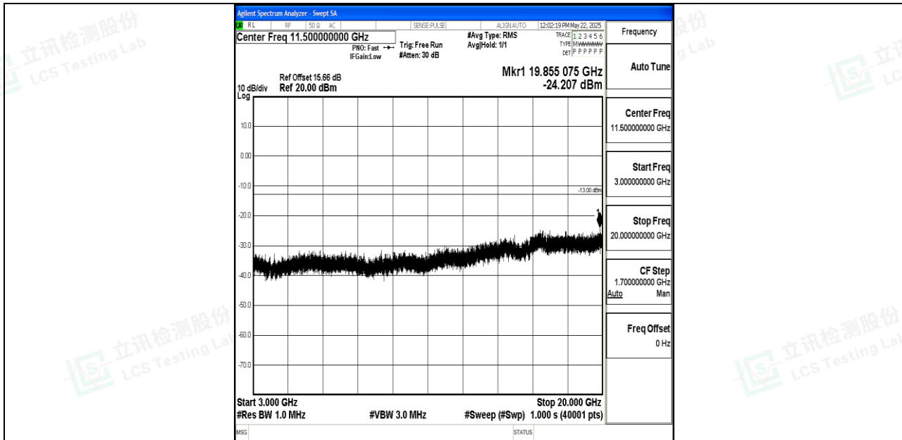
Band4_15MHz_16QAM_20025_1RB#0_3000~20000_3000~20000
