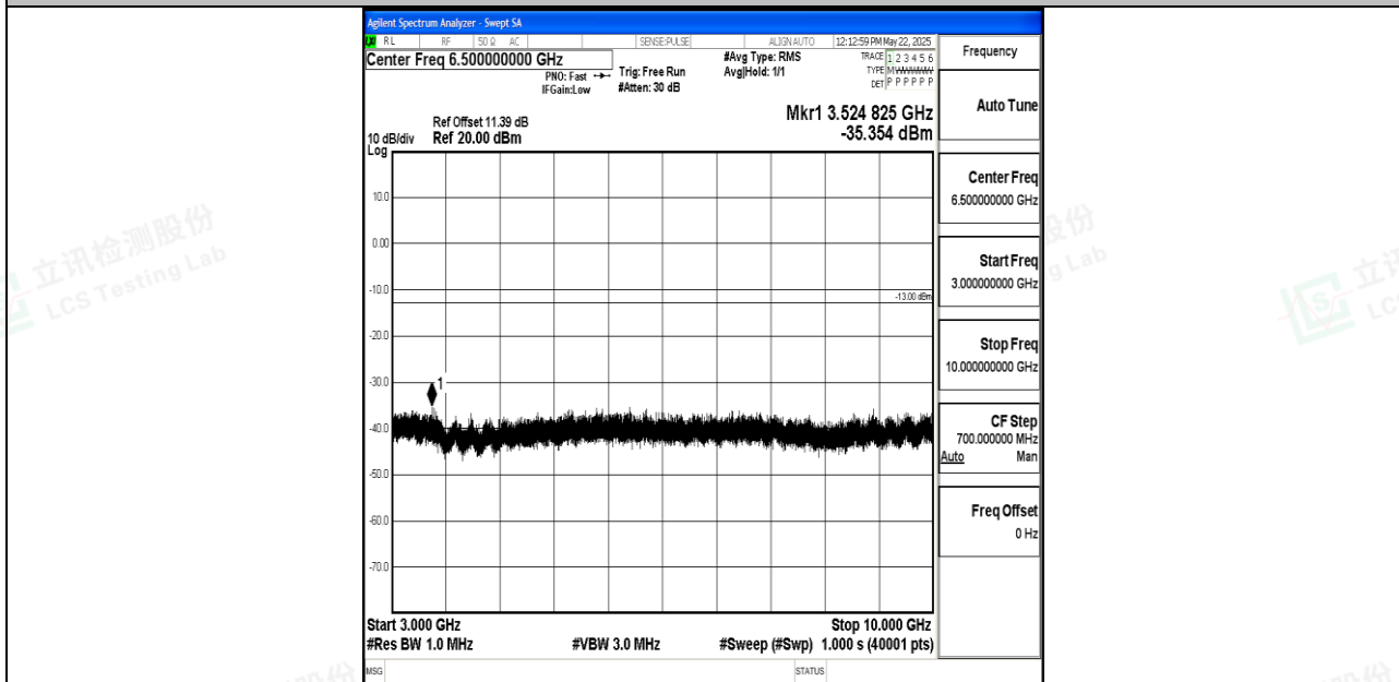
Band5_1.4MHz_16QAM_20407_1RB#0_3000~10000_3000~10000
