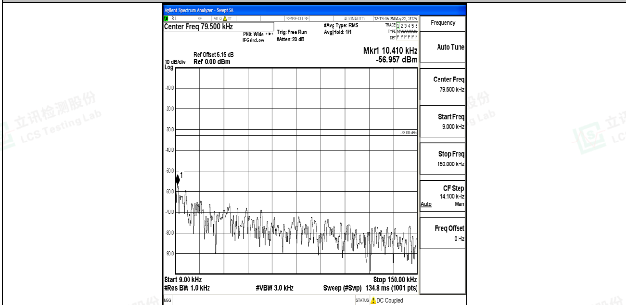
Band5_1.4MHz_16QAM_20525_1RB#0_0.009~0.15_0.009~0.15
