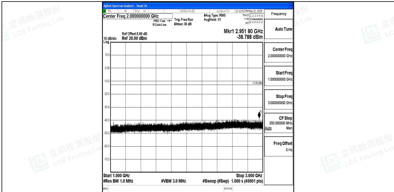
Band5_1.4MHz_16QAM_20407_1RB#0_1000~3000_1000~3000
