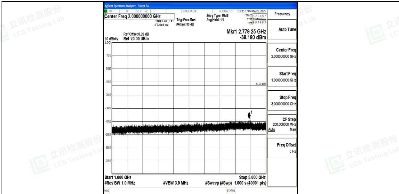
Band5_1.4MHz_16QAM_20643_1RB#0_1000~3000_1000~3000
