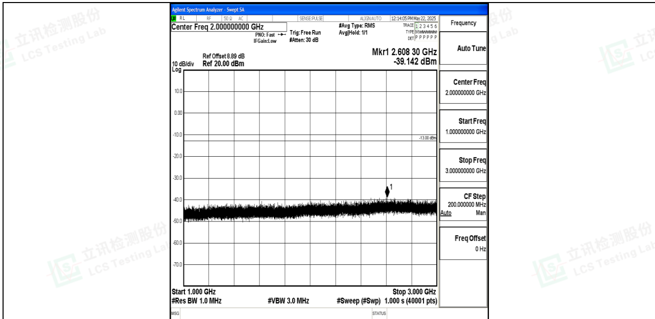
Band5_1.4MHz_16QAM_20525_1RB#0_1000~3000_1000~3000
