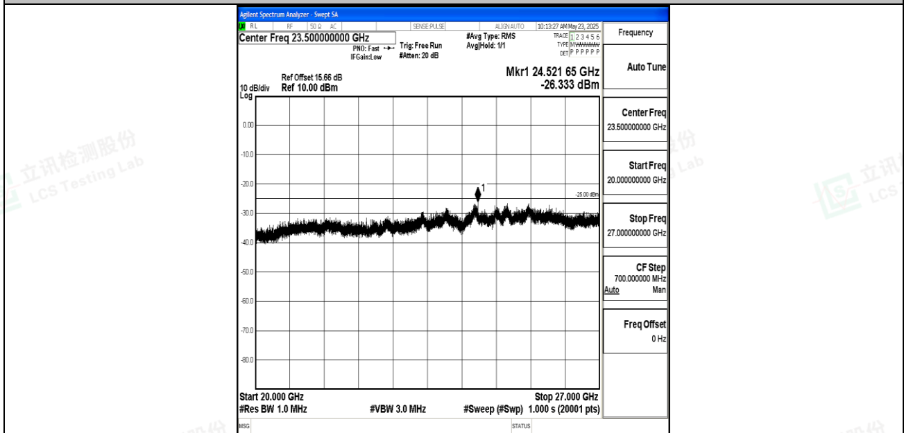
Band7_20MHz_16QAM_20850_1RB#0_20000~27000_20000~27000
