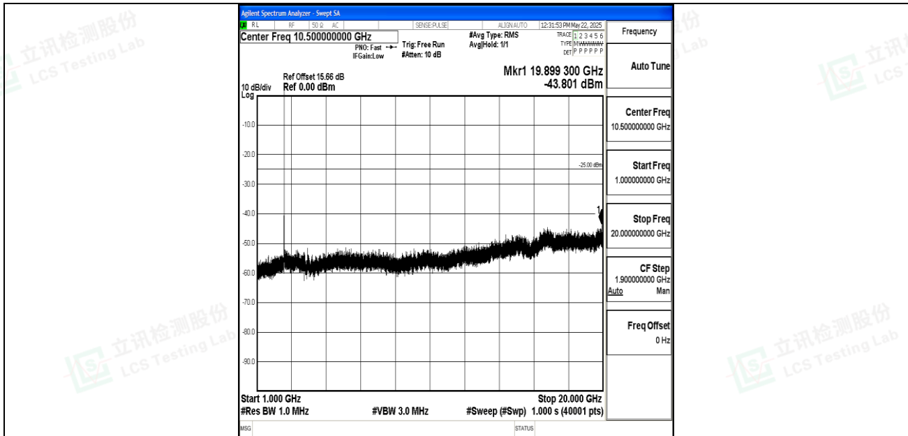
Band7_5MHz_16QAM_20775_1RB#0_1000~20000_1000~20000
