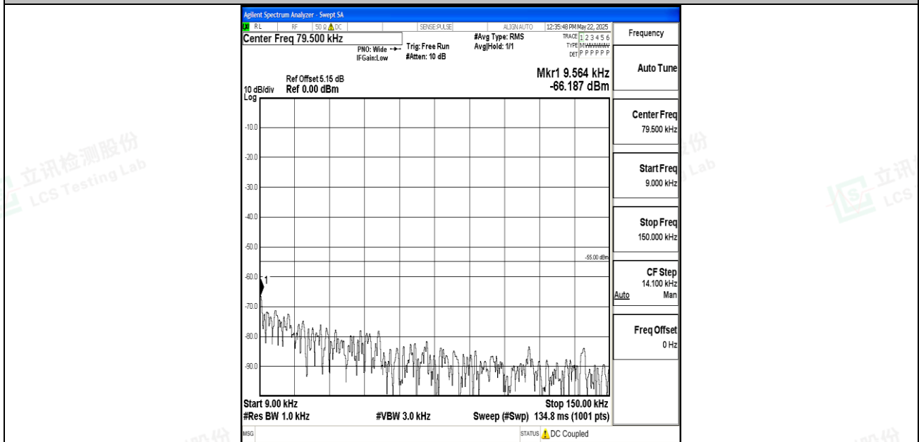
Band7_10MHz_16QAM_20800_1RB#0_0.009~0.15_0.009~0.15
