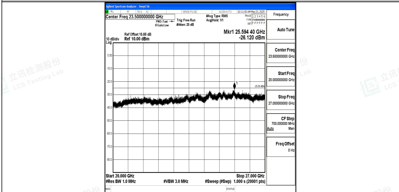
Band7_15MHz_16QAM_21100_1RB#0_20000~27000_20000~27000
