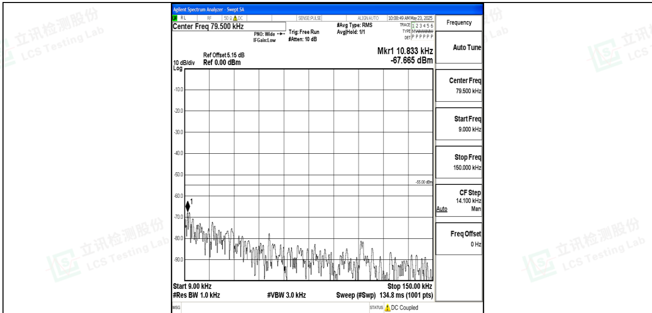
Band7_15MHz_QPSK_20825_1RB#0_0.009~0.15_0.009~0.15
