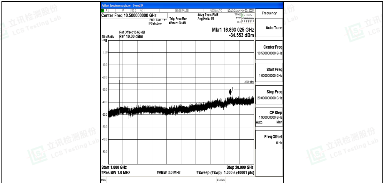
Band7_20MHz_16QAM_20850_1RB#0_1000~20000_1000~20000
