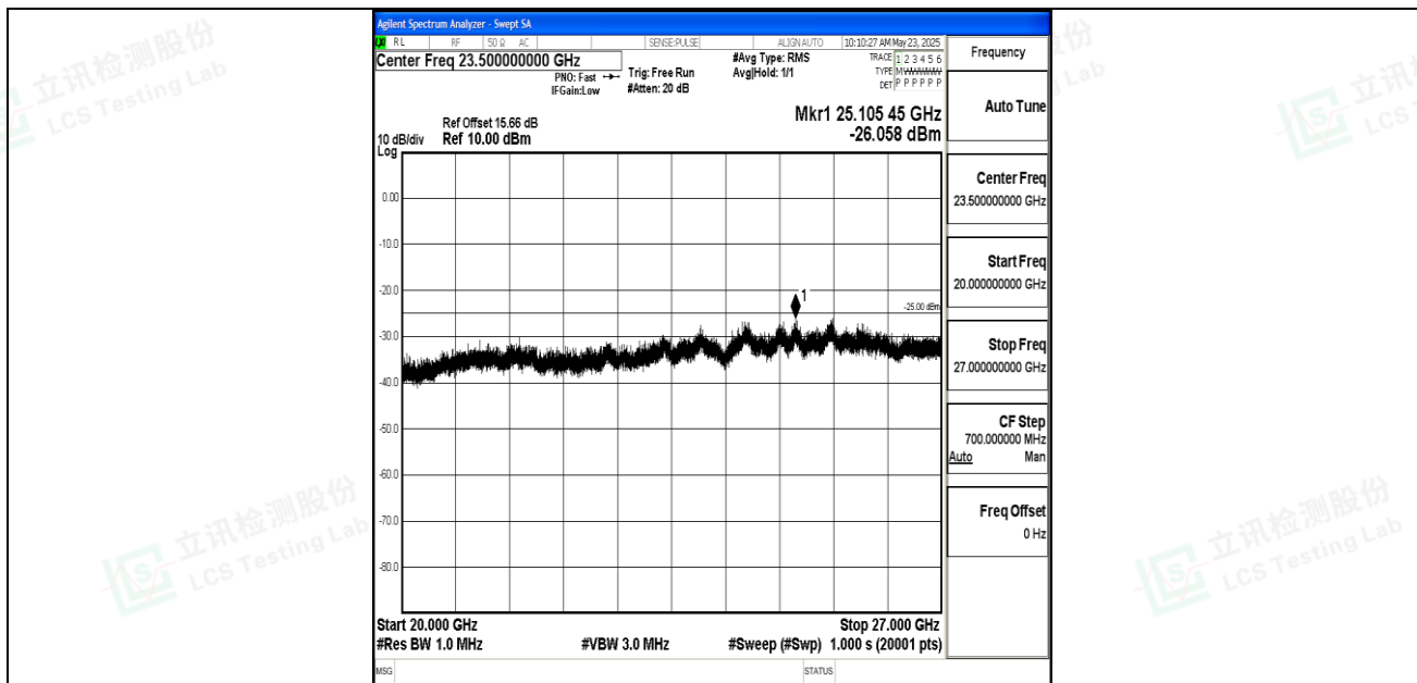
Band7_15MHz_QPSK_21100_1RB#0_20000~27000_20000~27000
