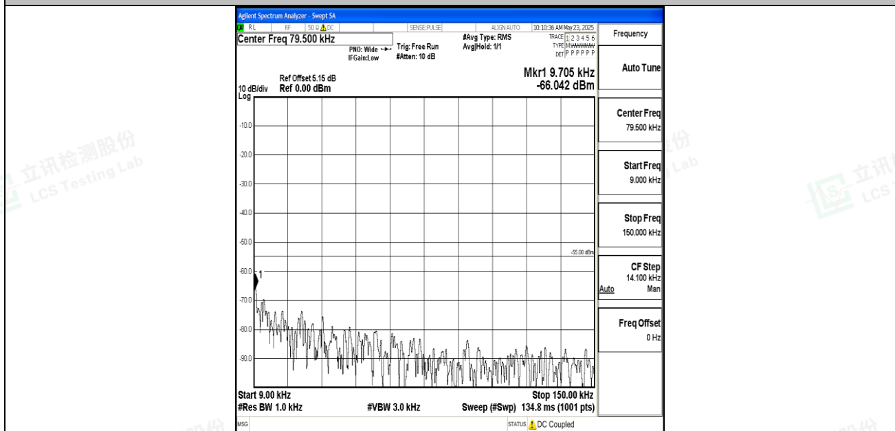
Band7_15MHz_16QAM_21100_1RB#0_0.009~0.15_0.009~0.15
