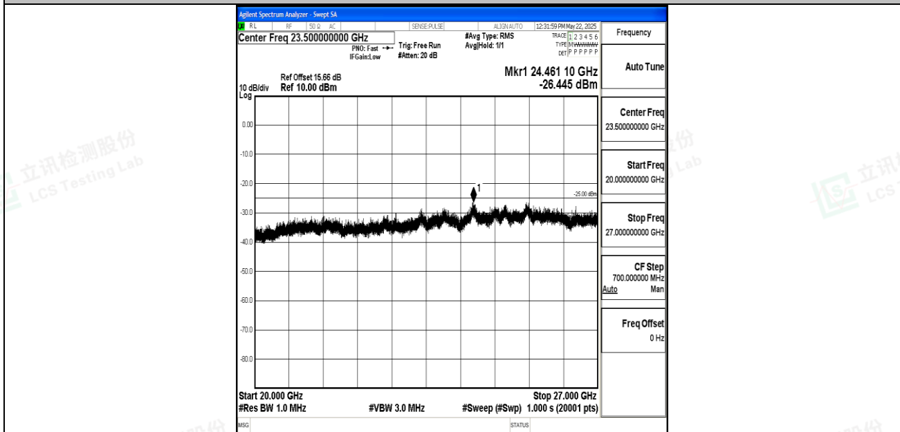
Band7_5MHz_16QAM_20775_1RB#0_20000~27000_20000~27000
