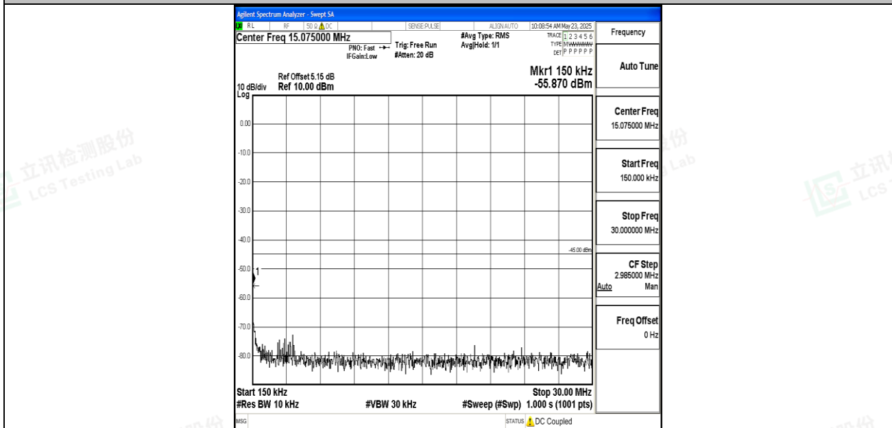
Band7_15MHz_QPSK_20825_1RB#0_0.15~30_0.15~30
