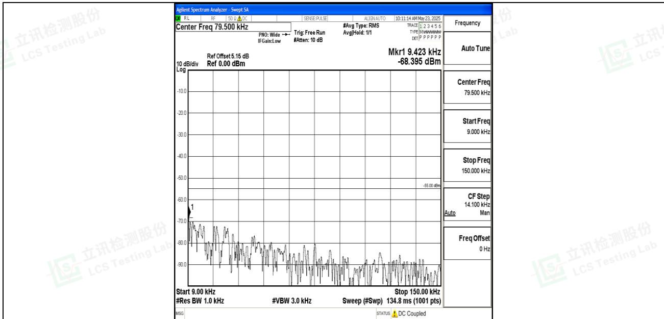
Band7_15MHz_QPSK_21375_1RB#0_0.009~0.15_0.009~0.15
