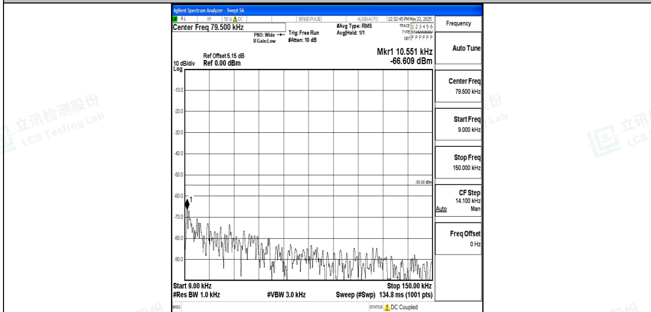
Band7_5MHz_16QAM_21100_1RB#0_0.009~0.15_0.009~0.15
