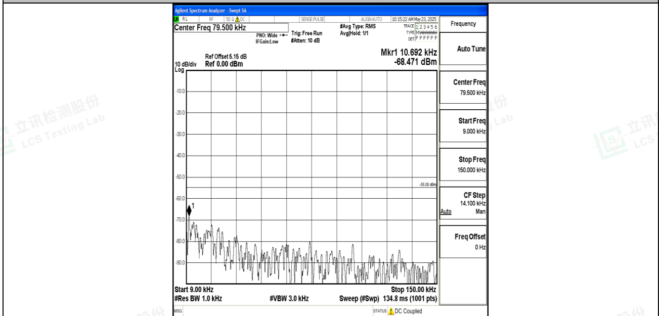
Band7_20MHz_16QAM_21350_1RB#0_0.009~0.15_0.009~0.15
