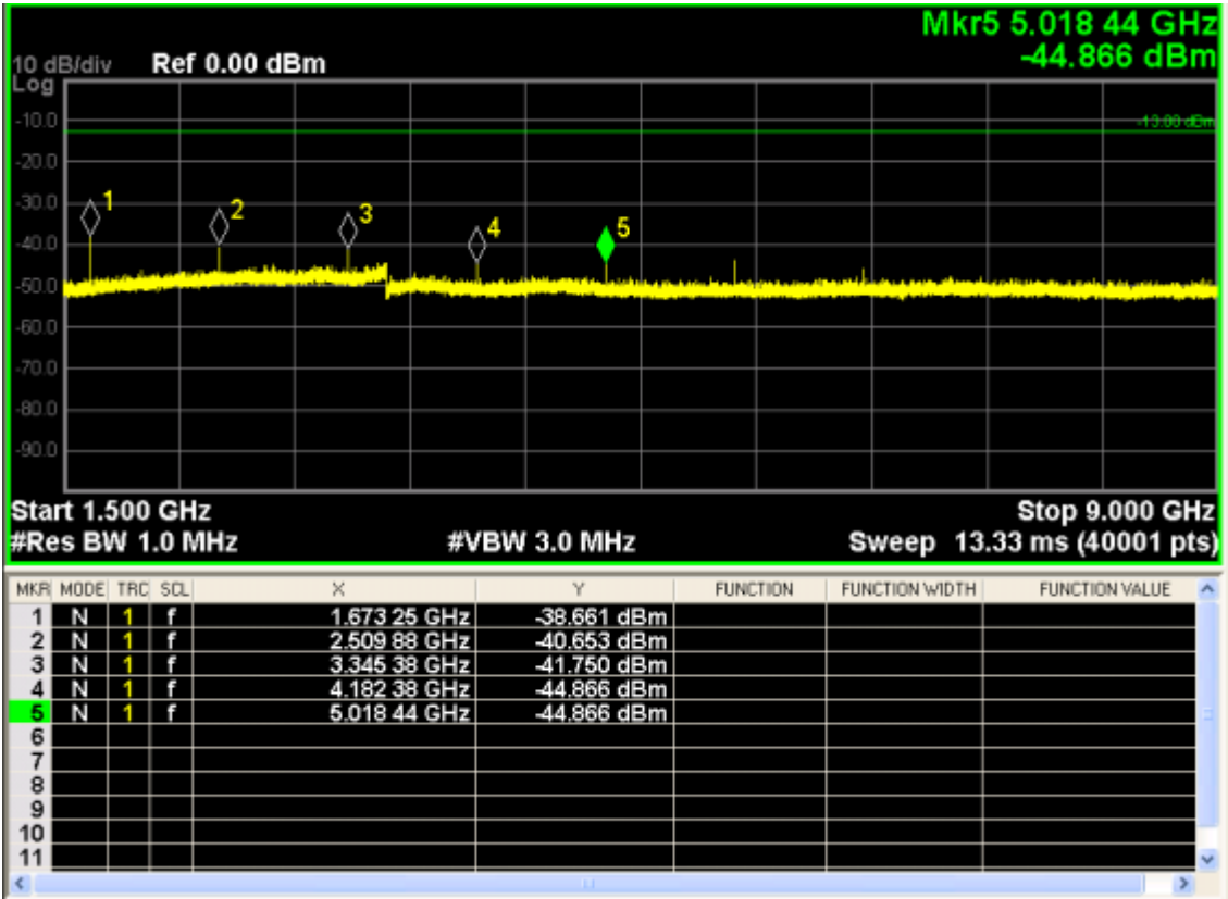
GSM850 (GPRS 1 Tx Slot), Channel 189
