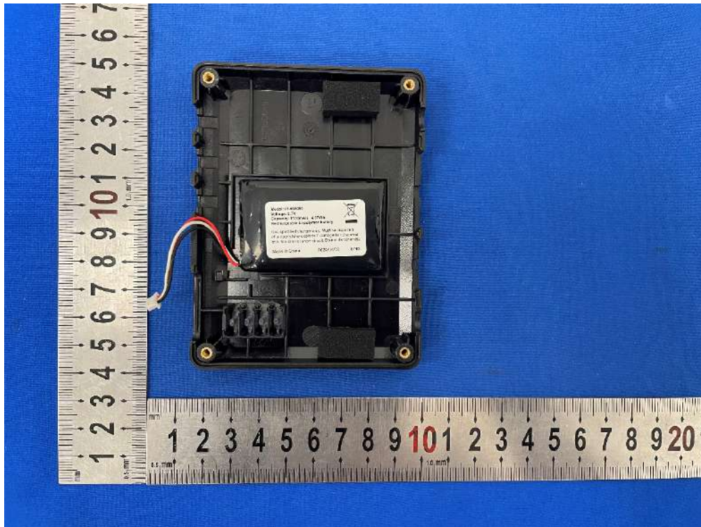
Photo 2: Internal View for Battery
