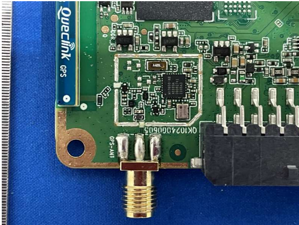
Photo 11: Internal View for GNSS chip
