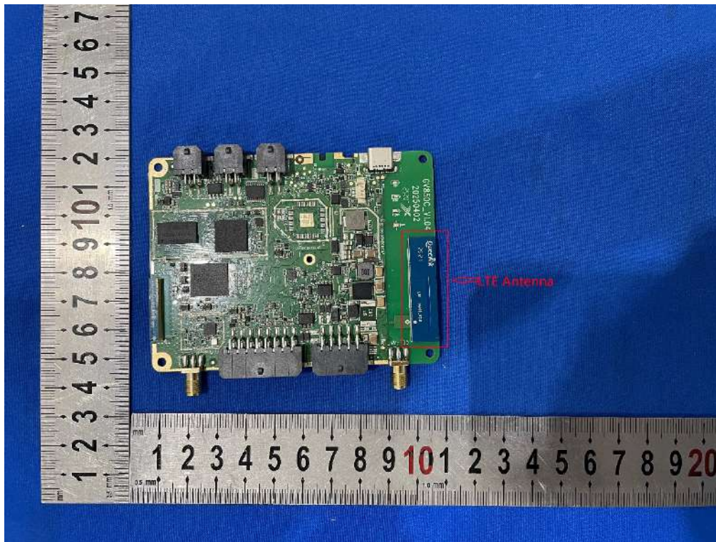
Photo 15: Internal View for LTE Antenna (QA100_V3.0_MIRROR)
