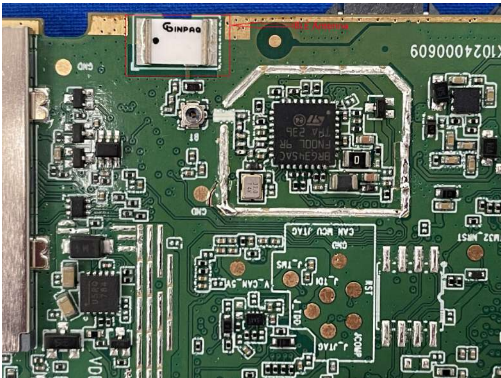
Photo 14: Internal View for BLE Antenna
