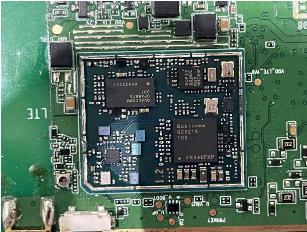
Photo 9: Internal View for LTE Chip
