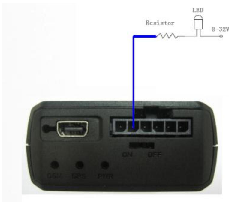
Figure 13. Typical Connection with LED
