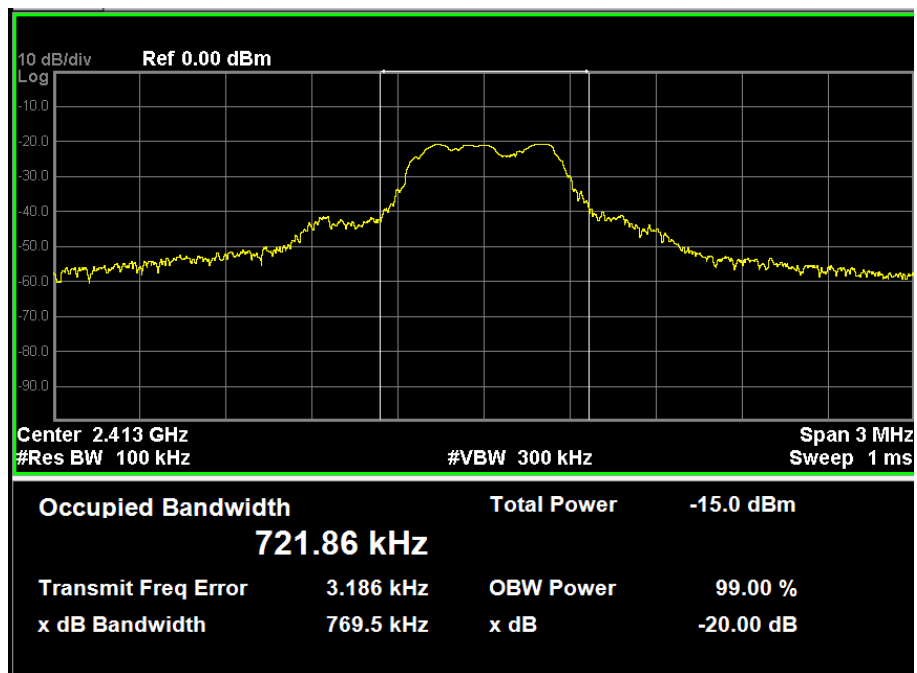
Mid Channel – Bandwidth 770 kHz
