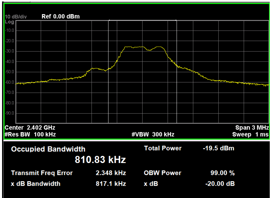
Low Channel – Bandwidth 817 kHz
