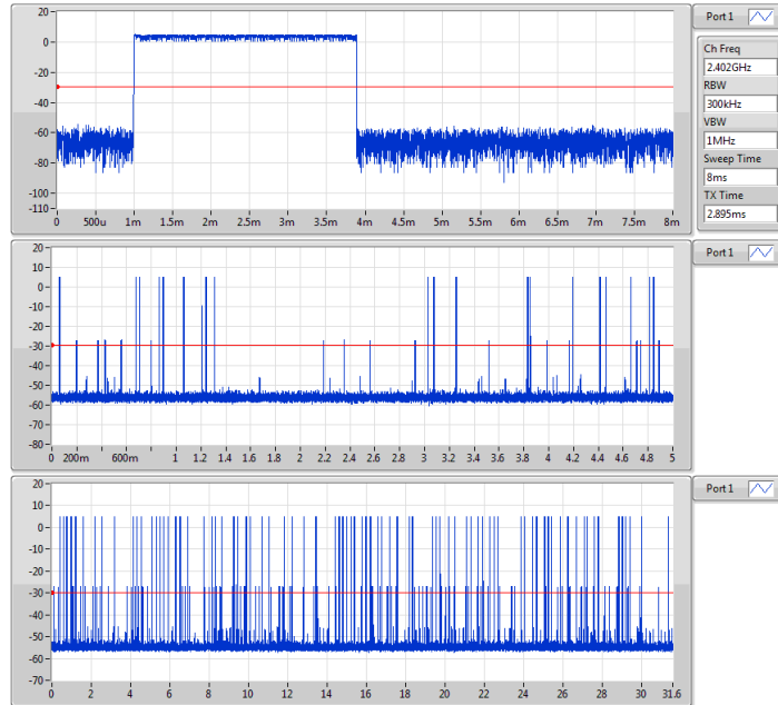
BT-BR(1Mbps) 2402MHz
