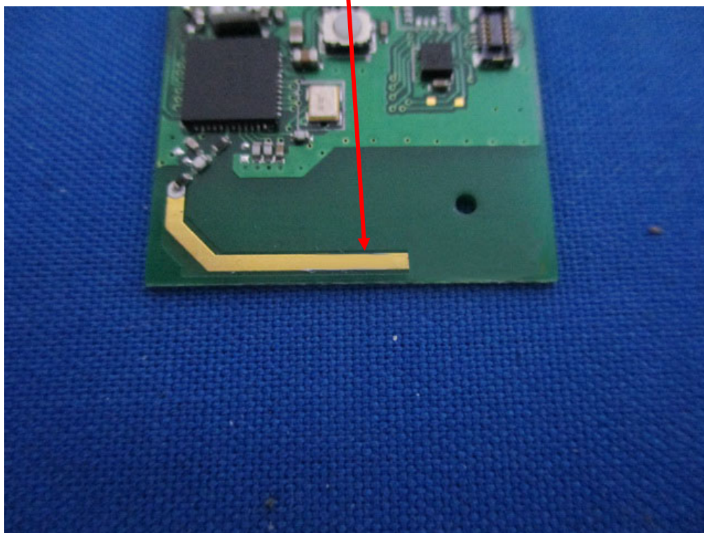
BLE&ANT+ Antenna
