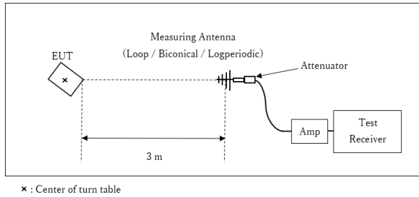
Figure 2: Test Setup
