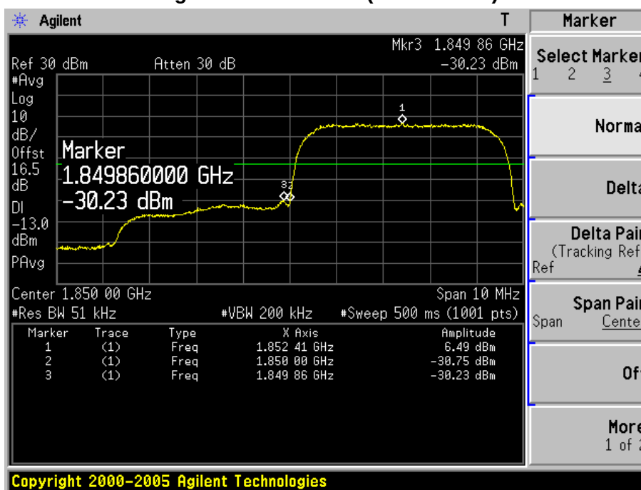
Figure Channel 9262 (1852.40MHz)
