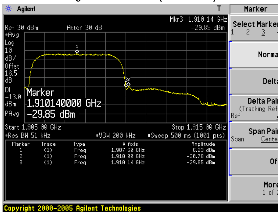
Figure Channel 9538 (1907.60MHz)
