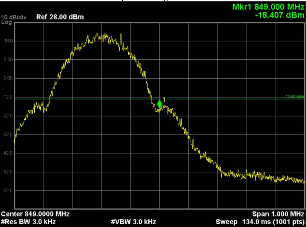
GSM850 (GSM Link), Channel 251
