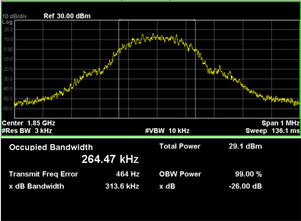
GSM1900 (GPRS Link), Channel 512
