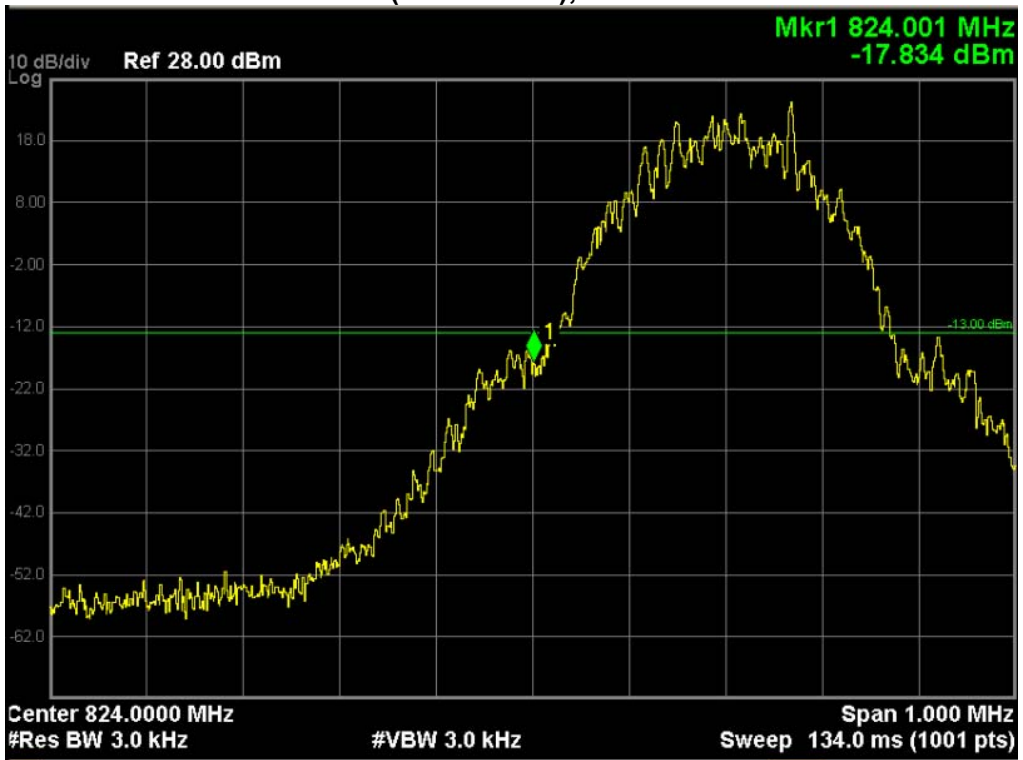
GSM850 (GPRS Link), Channel 128
