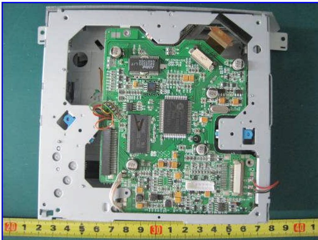
Front View of DVD PCB Board
