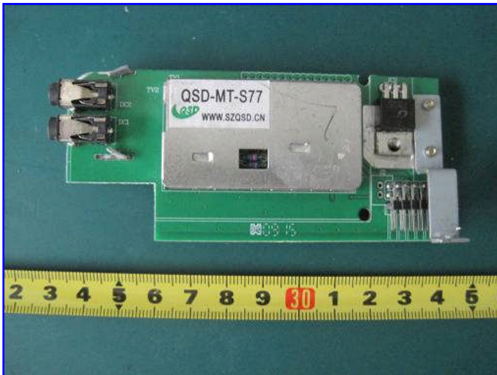
Front View of TV Module PCB
