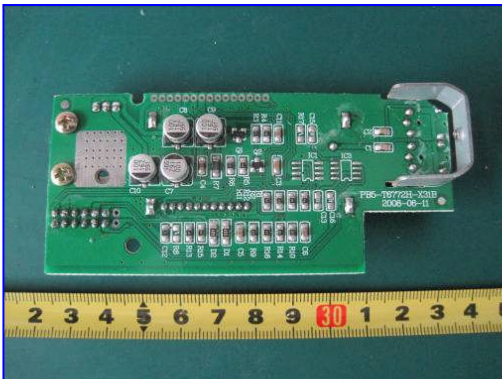
Rear View of TV Module PCB
