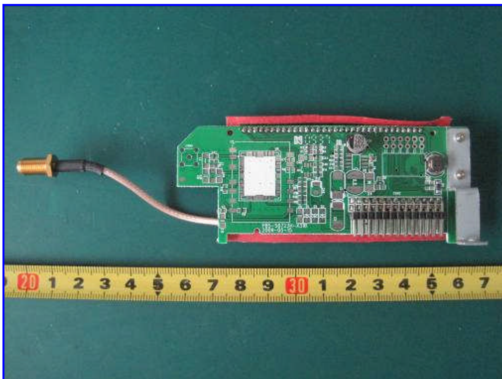
Rear View of GSM module PCB
