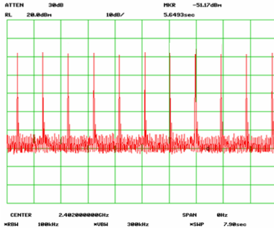
Low Channel (Sweep in 7.9sec)
