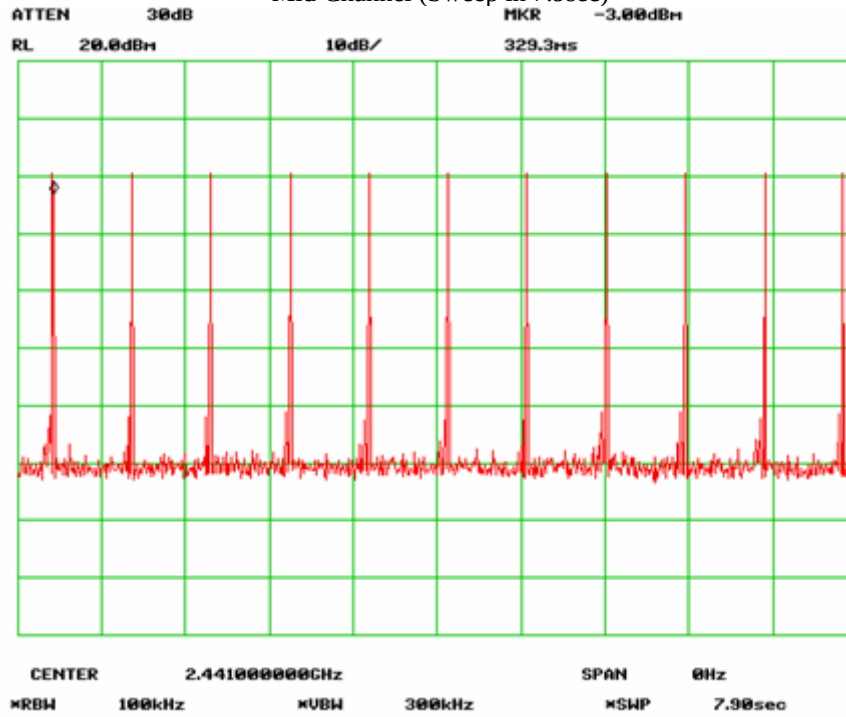
Mid Channel (Sweep in 7.9sec)
