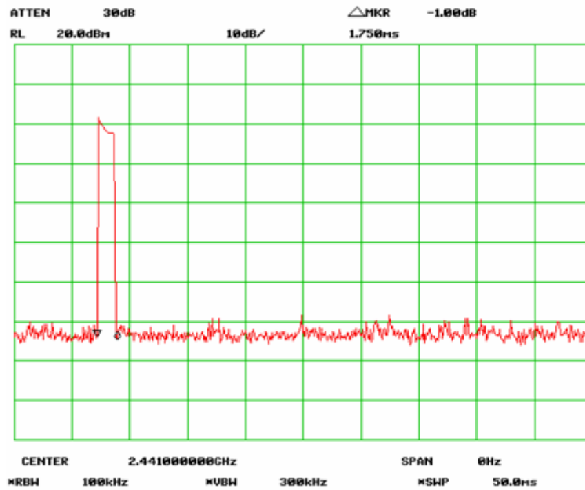
Mid Channel (Sweep in 50msec)
