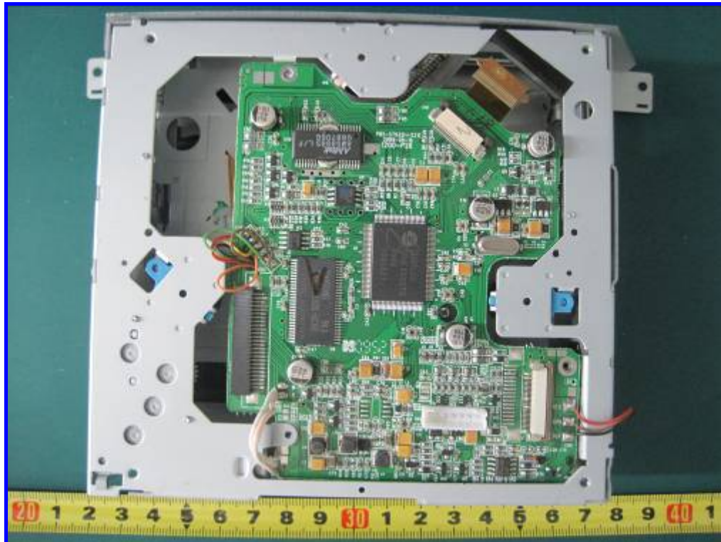
Front View of DVD PCB Board
