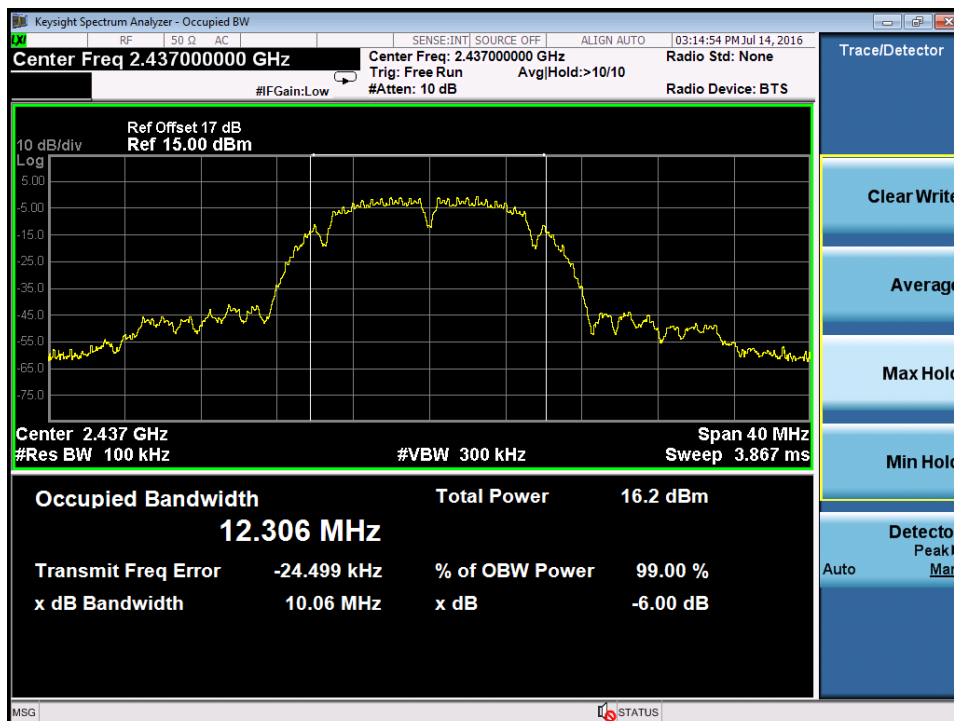
Figure 2: 6dB Bandwidth, Ant 0, 11b, 2437MHz
