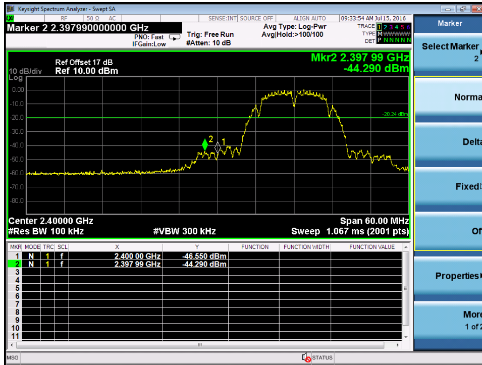
Figure 61: Conducted Bandedge, Ant 0, 11b, 2412MHz
