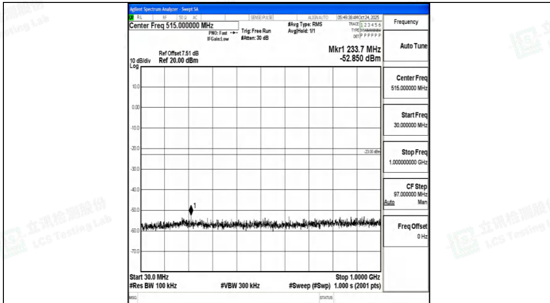
Band2_15MHz_QPSK_18675_1RB#0_30~1000_30~1000
