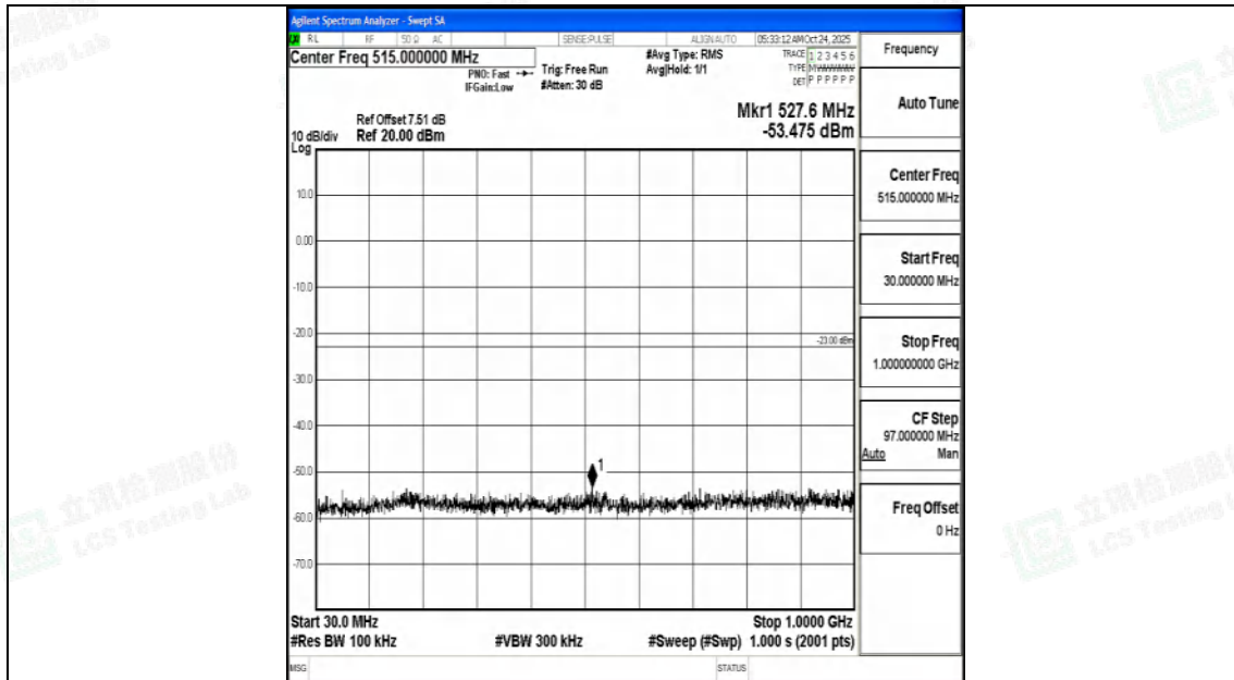
Band2_10MHz_QPSK_18900_1RB#0_30~1000_30~1000
