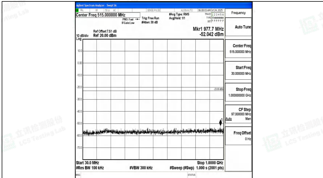
Band2_20MHz_QPSK_18900_1RB#0_30~1000_30~1000
