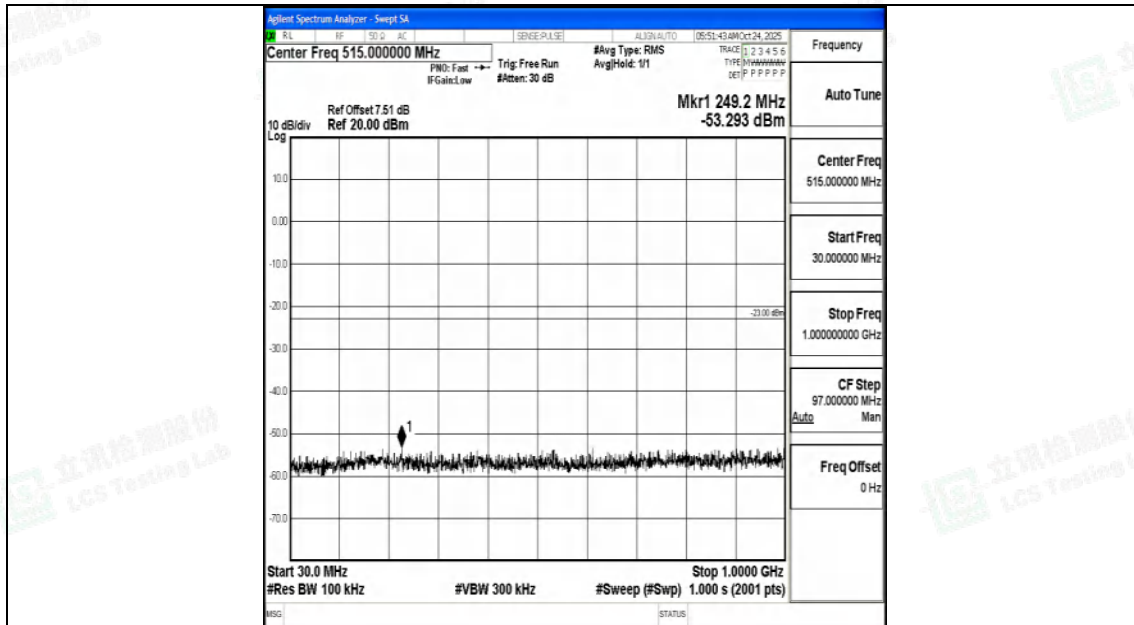
Band2_15MHz_QPSK_19125_1RB#0_30~1000_30~1000
