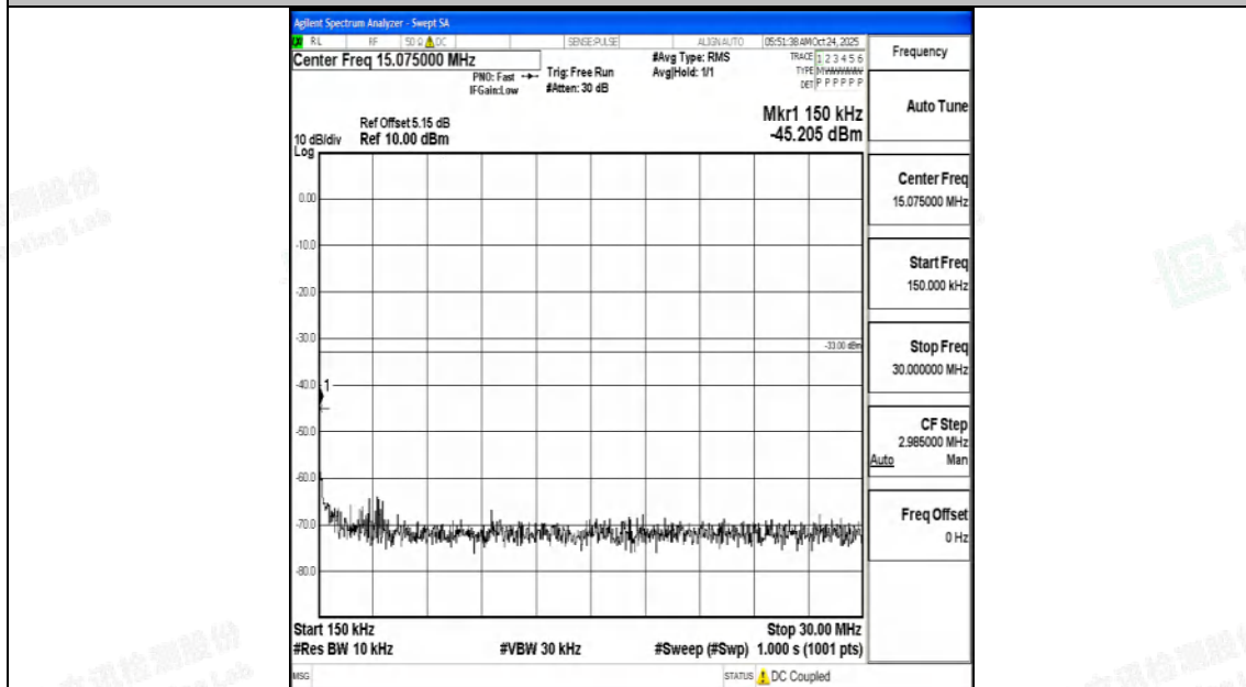
Band2_15MHz_QPSK_19125_1RB#0_0.15~30_0.15~30
