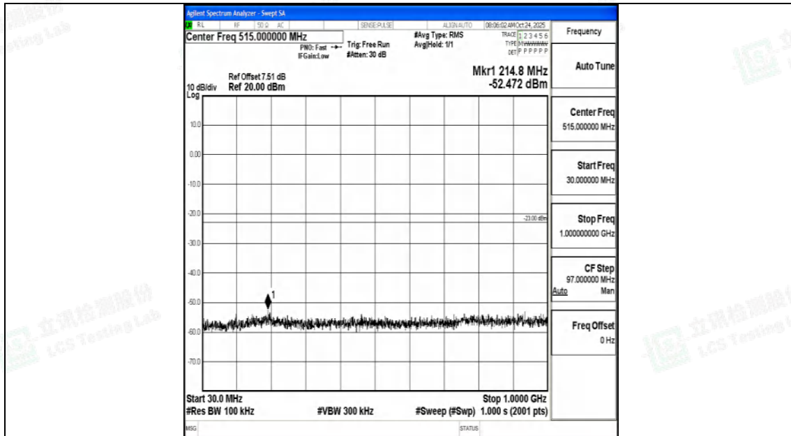
Band4_20MHz_QPSK_20300_1RB#0_30~1000_30~1000
