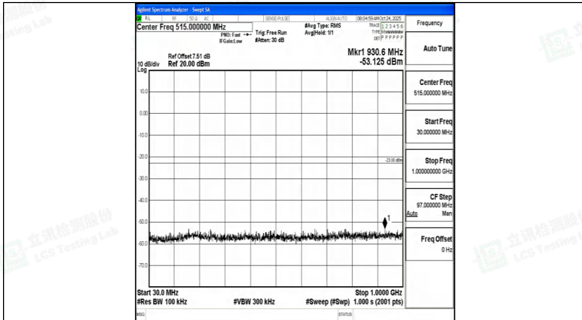
Band4_20MHz_QPSK_20175_1RB#0_30~1000_30~1000
