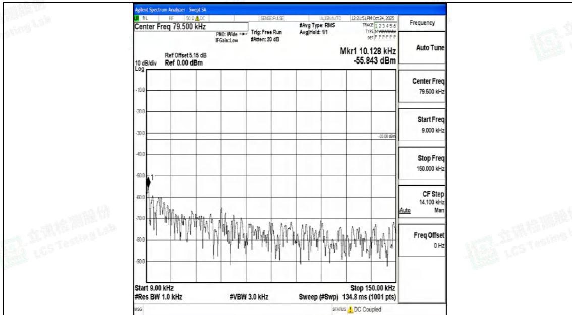
Band12_10MHz_QPSK_23095_1RB#0_0.009~0.15_0.009~0.15
