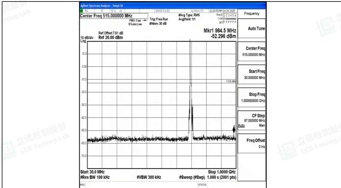
Band12_10MHz_QPSK_23060_1RB#0_30~1000_30~1000
