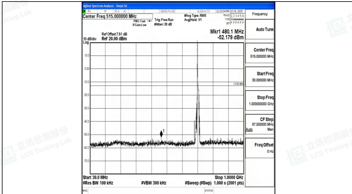
Band12_10MHz_QPSK_23130_1RB#0_30~1000_30~1000
