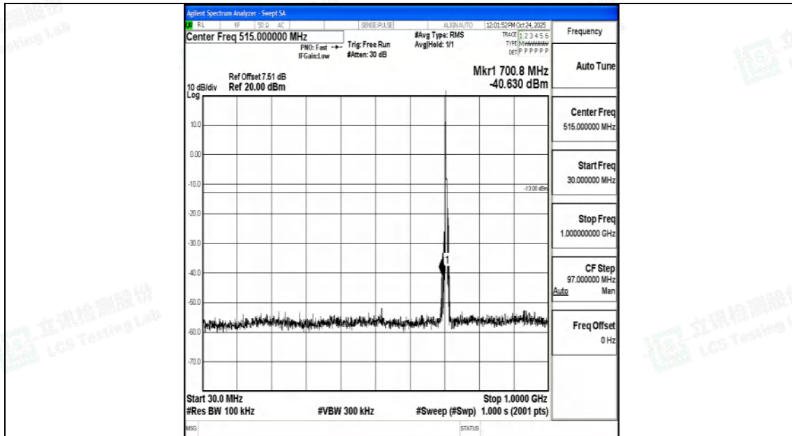
Band12_5MHz_QPSK_23155_1RB#0_30~1000_30~1000
