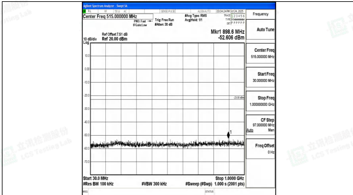
Band25_10MHz_QPSK_26365_1RB#0_30~1000_30~1000
