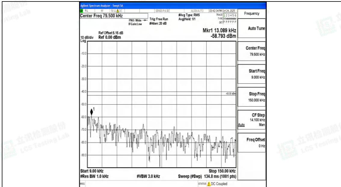
Band25_20MHz_QPSK_26140_1RB#0_0.009~0.15_0.009~0.15
