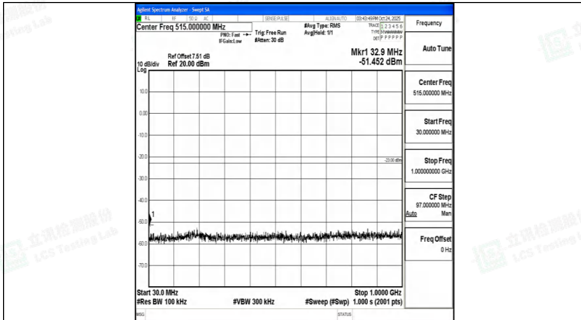
Band25_20MHz_QPSK_26365_1RB#0_30~1000_30~1000
