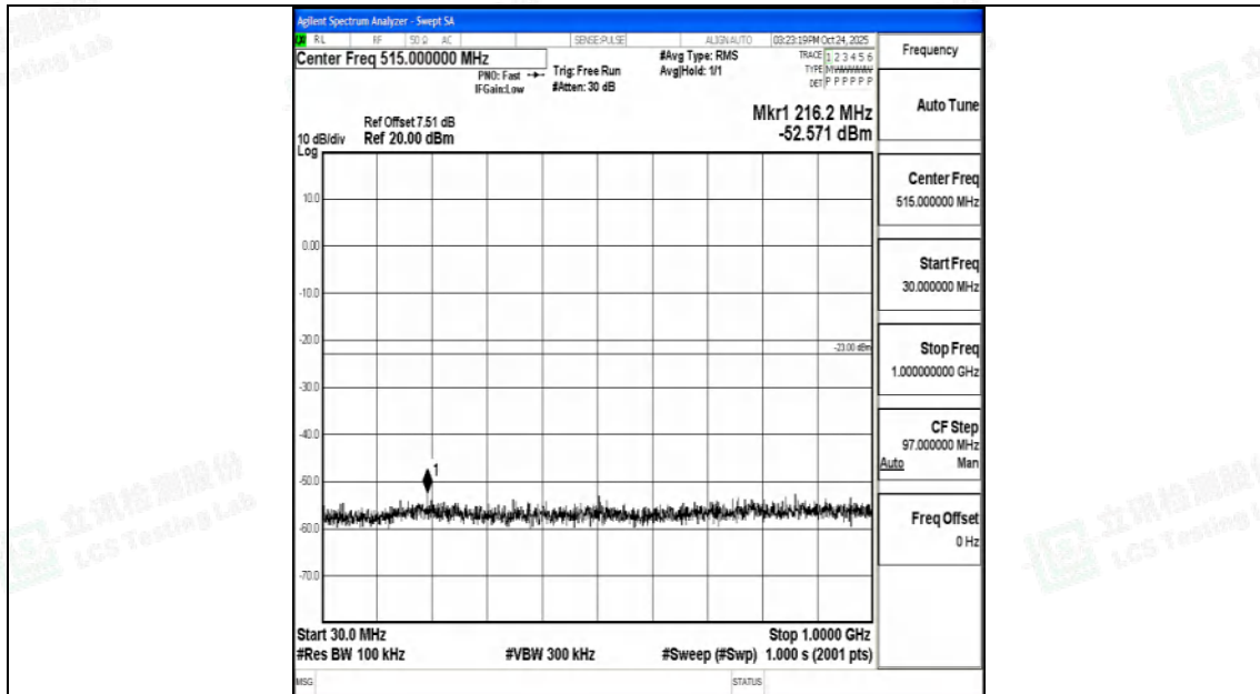
Band25_15MHz_QPSK_26115_1RB#0_30~1000_30~1000
