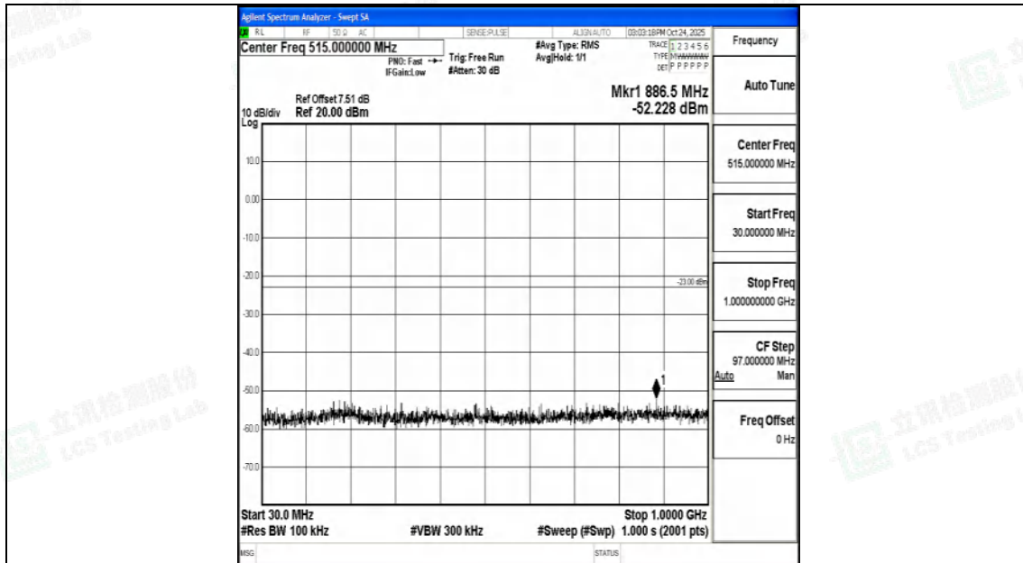
Band25_10MHz_QPSK_26090_1RB#0_30~1000_30~1000
