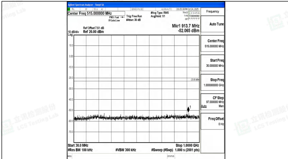
Band25_15MHz_QPSK_26615_1RB#0_30~1000_30~1000
