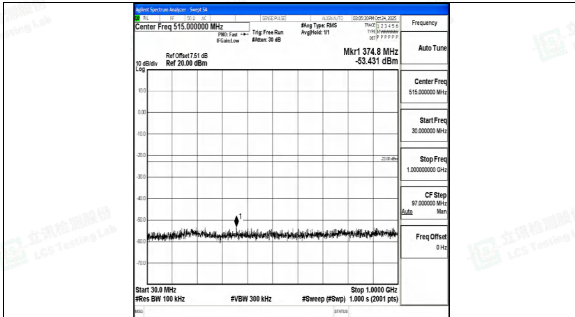
Band25_10MHz_QPSK_26640_1RB#0_30~1000_30~1000
