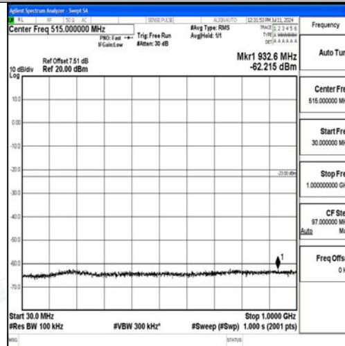
Band2_15MHz_QPSK_19125_1RB#0_30~1000_30~1000
