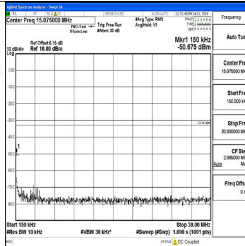
Band2_15MHz_QPSK_19125_1RB#0_0.15~30_0.15~30
