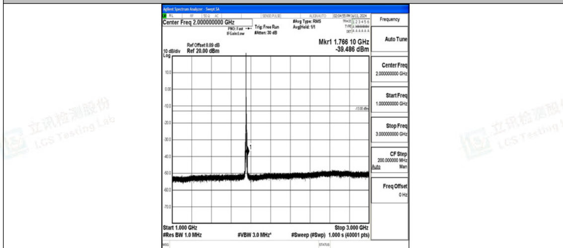
Band4_5MHz_QPSK_20375_1RB#0_1000~3000_1000~3000
