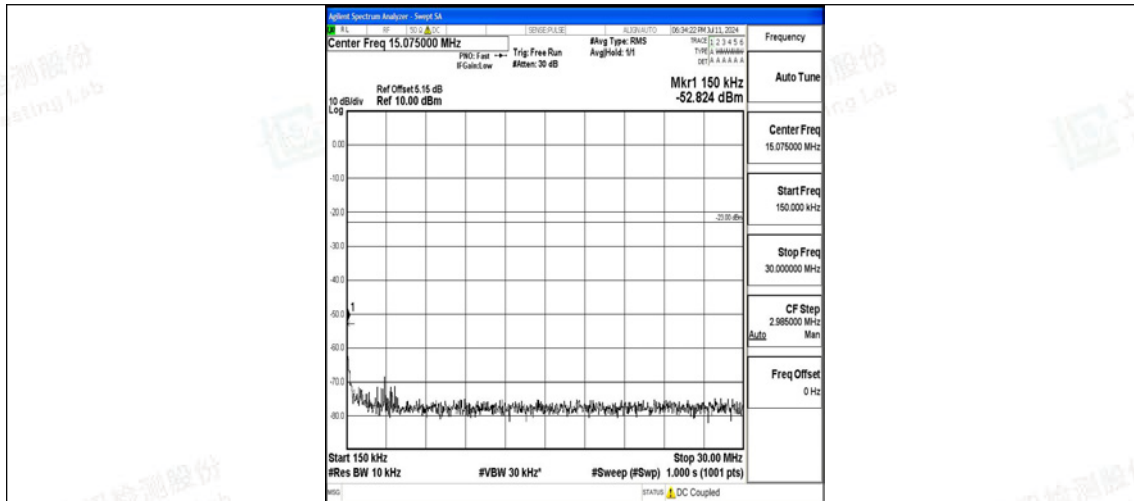
Band12_1.4MHz_QPSK_23173_1RB#0_0.15~30_0.15~30
