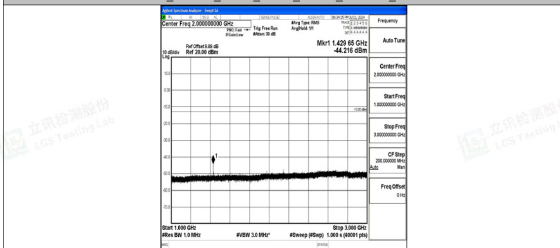
Band12_1.4MHz_QPSK_23173_1RB#0_1000~3000_1000~3000
