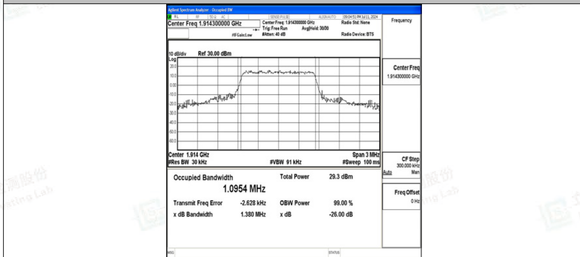
Band25-1.4MHz-QPSK-26683-6RB#0-PASS
