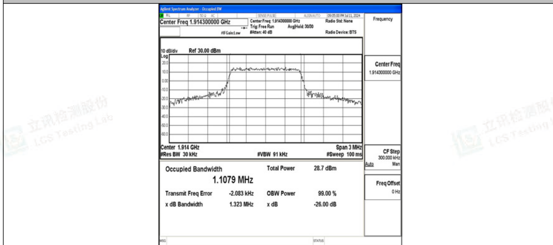
Band25-1.4MHz-16QAM-26683-6RB#0-PASS
