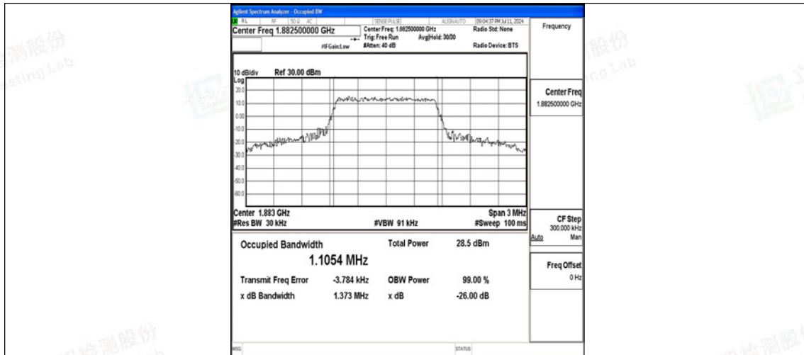
Band25-1.4MHz-16QAM-26365-6RB#0-PASS
