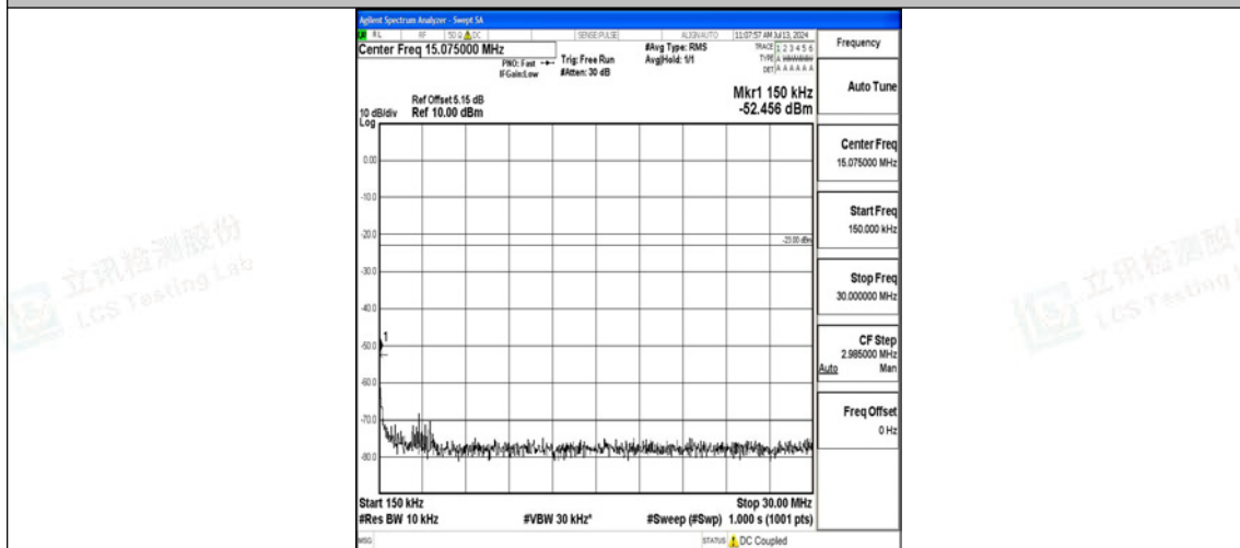
Band26_15MHz_QPSK_26915_1RB#0_0.15~30_0.15~30
