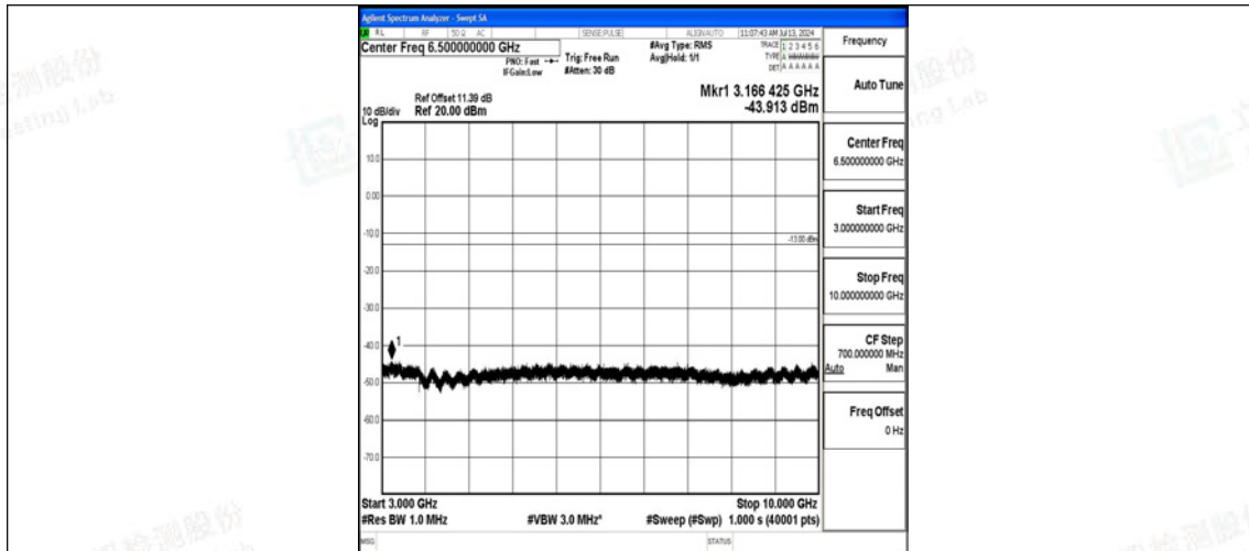
Band26_15MHz_16QAM_26865_1RB#0_3000~10000_3000~10000
