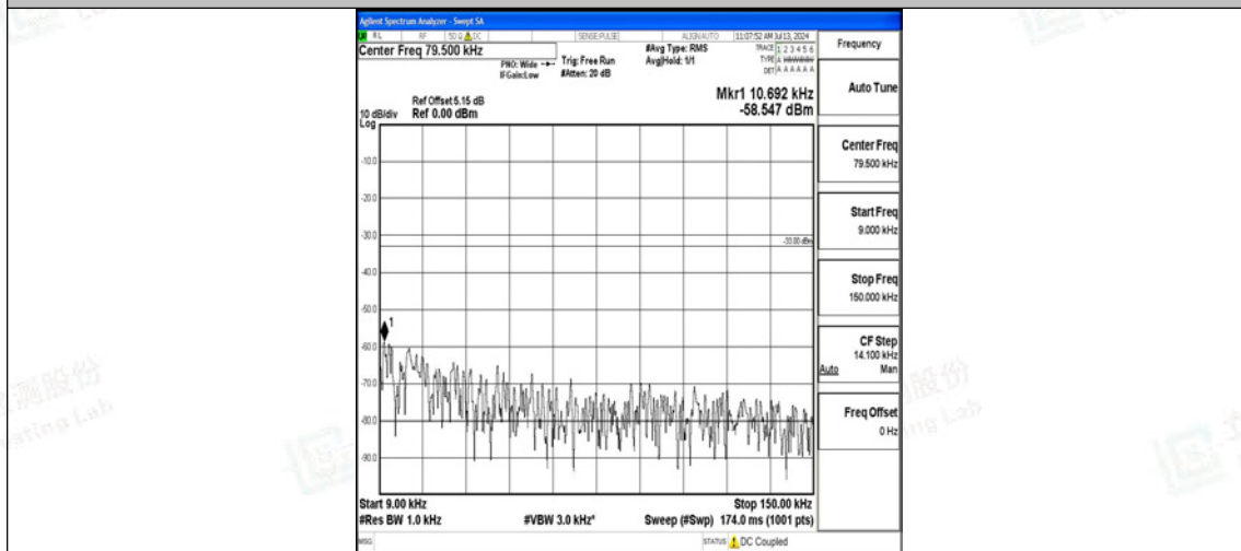
Band26_15MHz_QPSK_26915_1RB#0_0.009~0.15_0.009~0.15
