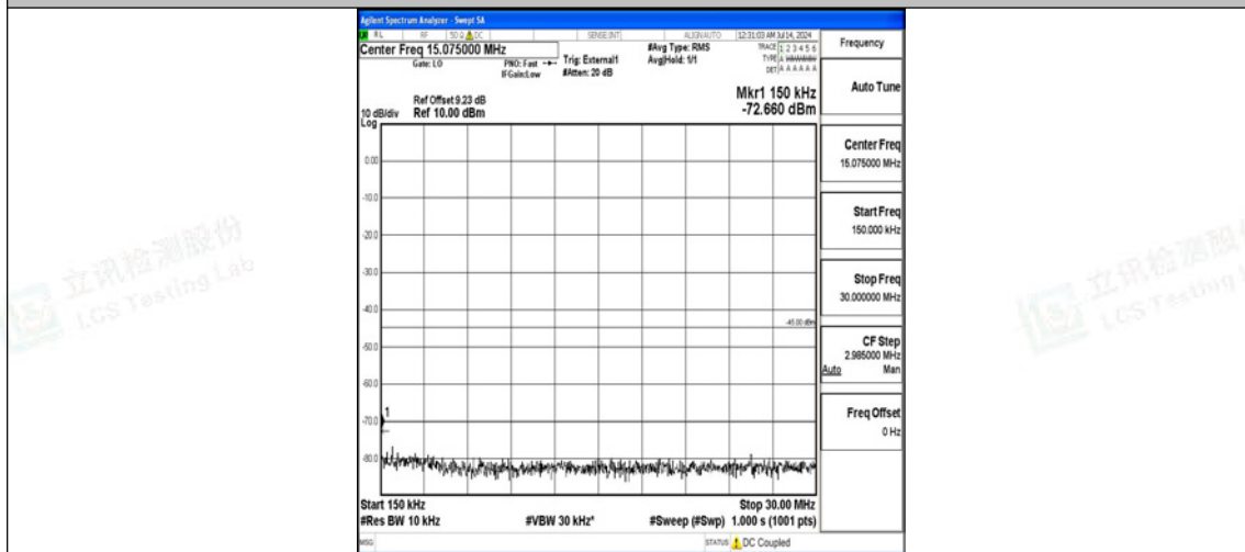
Band38-5MHz-QPSK-38000-25RB#0-0.15~30-PASS
