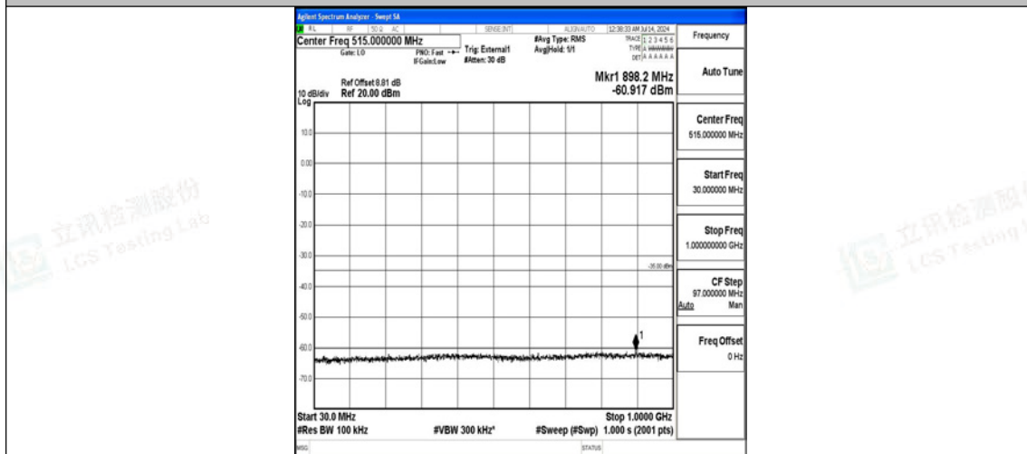
Band38-5MHz-16QAM-38225-25RB#0-30~1000-PASS
