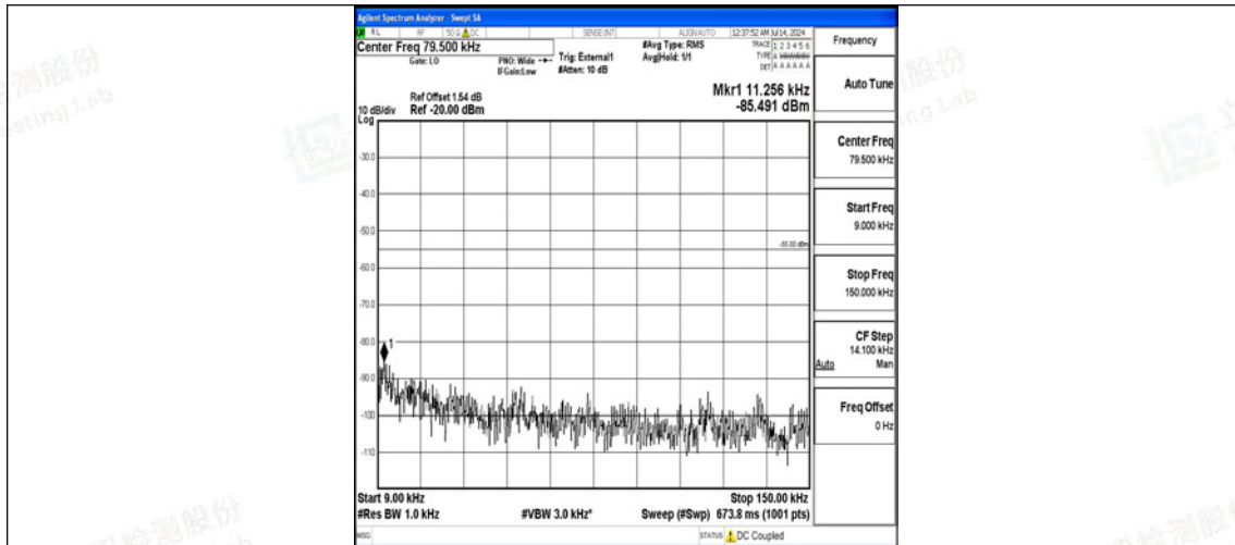
Band38-5MHz-16QAM-38225-25RB#0-0.009~0.15-PASS
