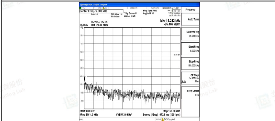
Band38-5MHz-16QAM-38000-25RB#0-0.009~0.15-PASS
