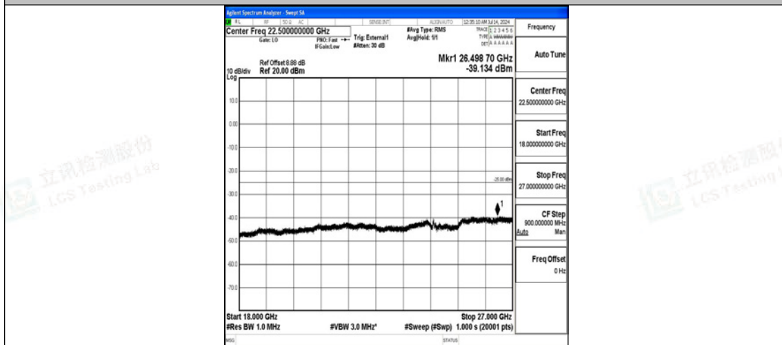
Band38-5MHz-16QAM-38000-25RB#0-18000~27000-PASS
