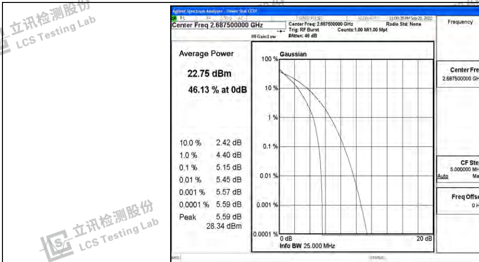
Band41-5MHz-16QAM-39675-25RB#0
