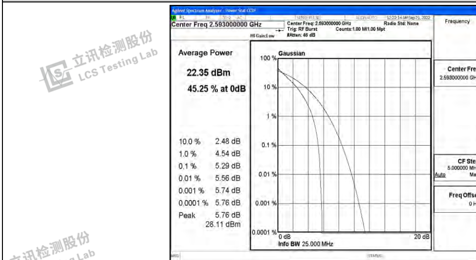
Band41-15MHz-QPSK-41515-75RB#0
