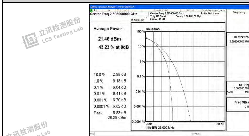
Band41-15MHz-16QAM-41515-75RB#0
