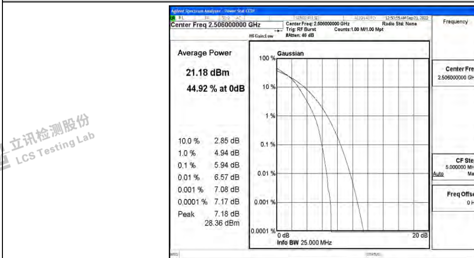
Band41-20MHz-16QAM-40620-100RB#0
