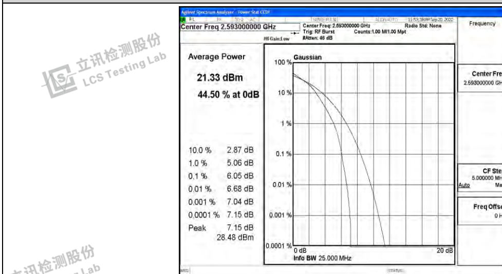
Band41-10MHz-16QAM-41540-50RB#0
