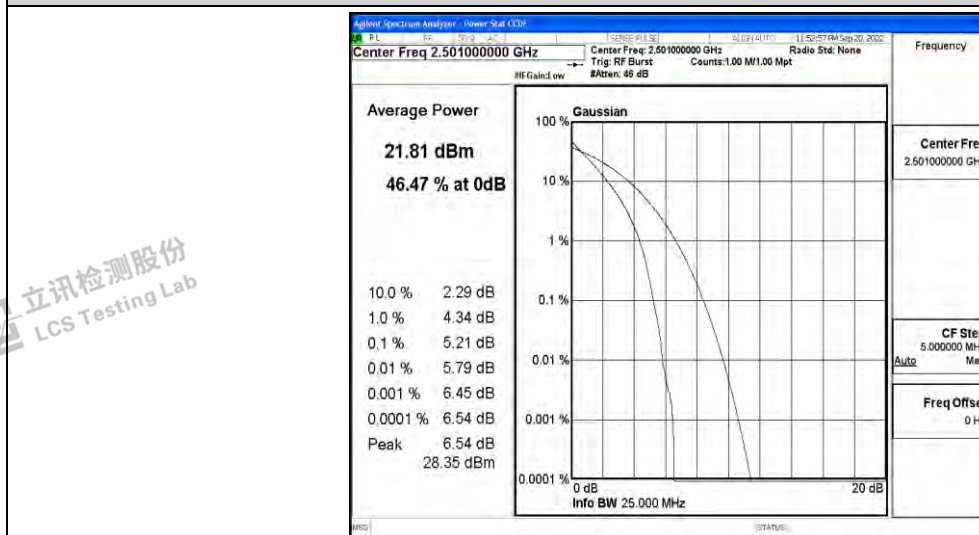
Band41-10MHz-QPSK-40620-50RB#0
