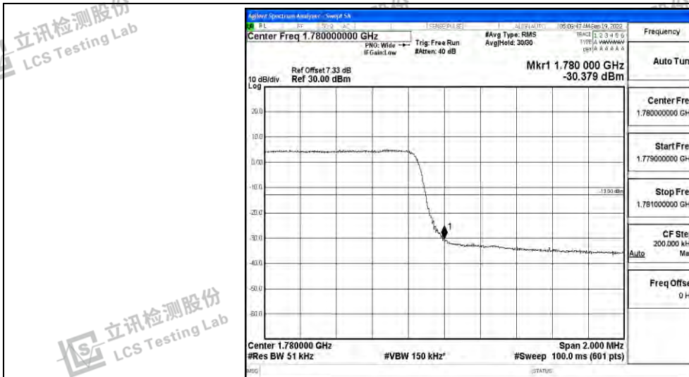
Band66-3MHz-16QAM-131987-15RB#0
