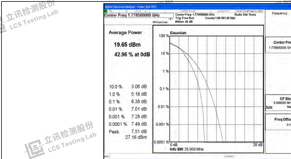
Band66-5MHz-QPSK-131997-25RB#0
