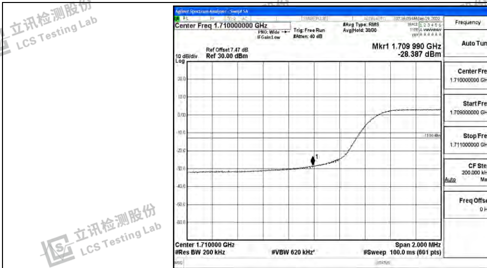
Band66-10MHz-16QAM-132622-50RB#0
