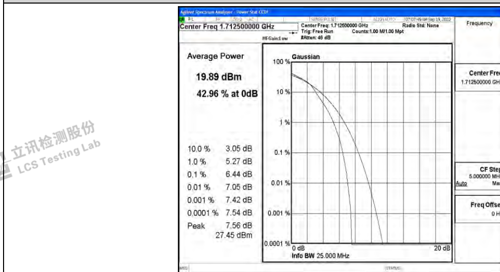
Band66-5MHz-16QAM-132322-25RB#0
