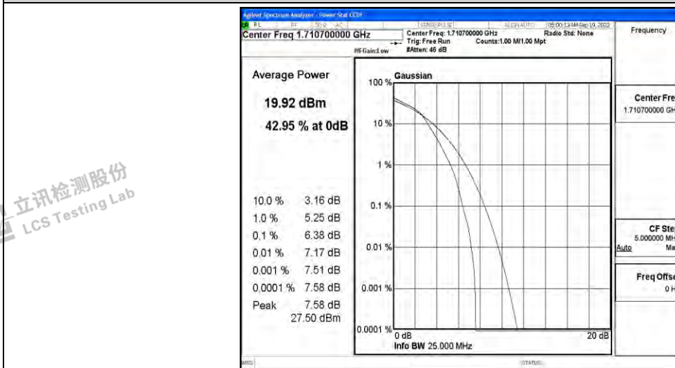
Band66-1.4MHz-16QAM-132322-6RB#0
