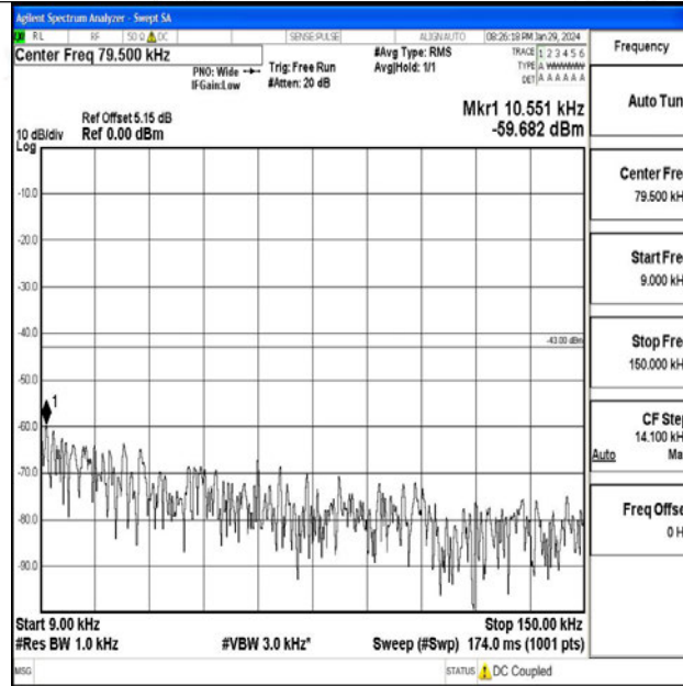
Band4_15MHz_QPSK_20175_1RB#0_0.009~0.15_0.009~0.15
