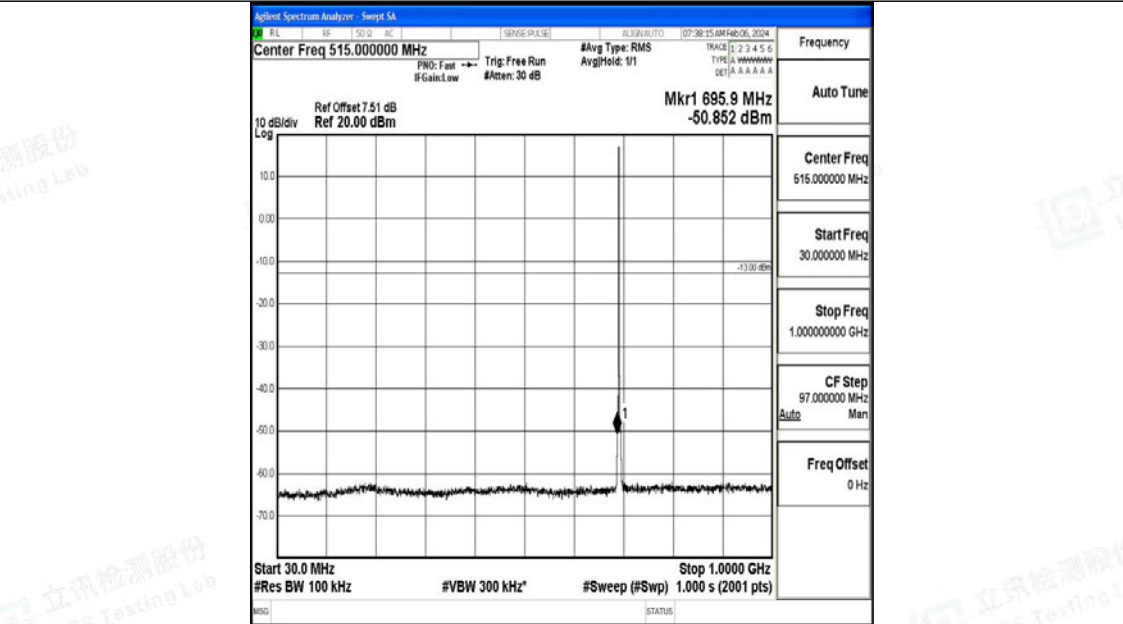
Band12_1.4MHz_QPSK_23017_1RB#0_30~1000_30~1000
