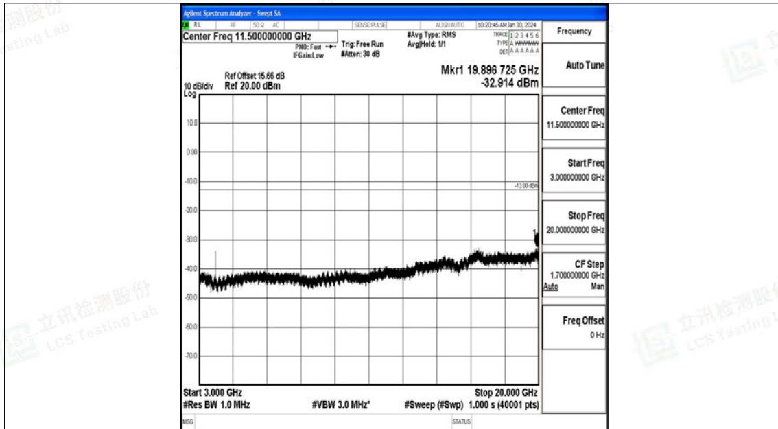
Band25_5MHz_QPSK_26665_1RB#0_3000~20000_3000~20000
