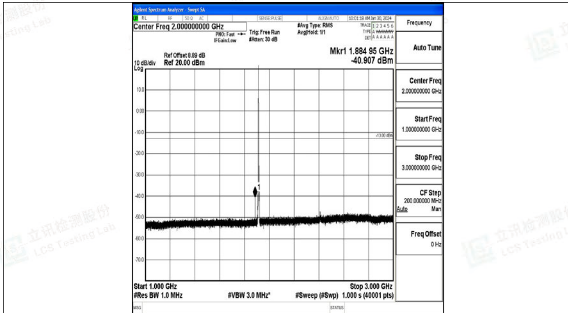
Band25_3MHz_16QAM_26675_1RB#0_1000~3000_1000~3000
