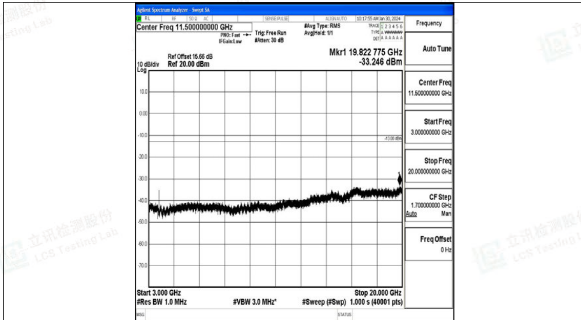
Band25_5MHz_QPSK_26065_1RB#0_3000~20000_3000~20000
