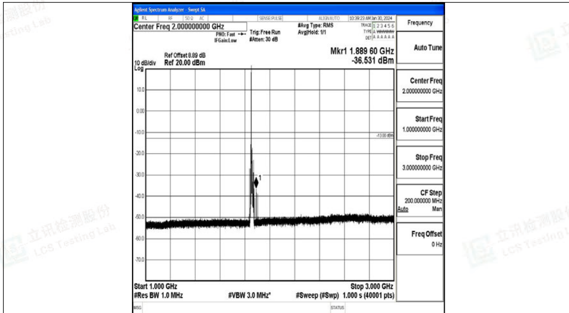
Band25_10MHz_16QAM_26090_1RB#0_1000~3000_1000~3000
