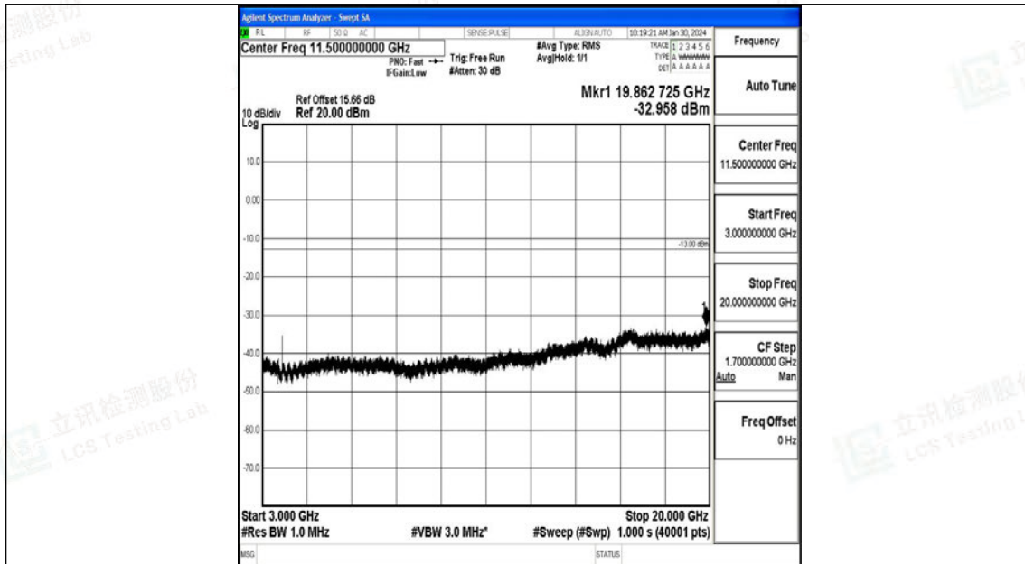
Band25_5MHz_QPSK_26365_1RB#0_3000~20000_3000~20000
