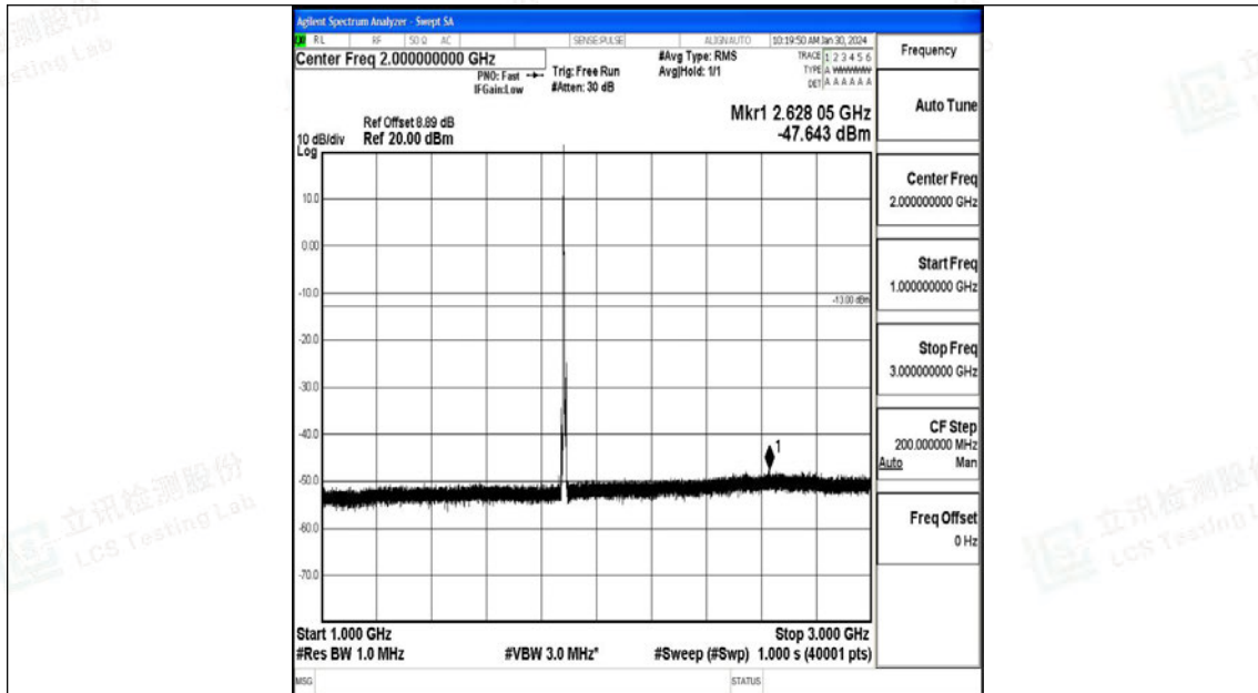
Band25_5MHz_16QAM_26365_1RB#0_1000~3000_1000~3000
