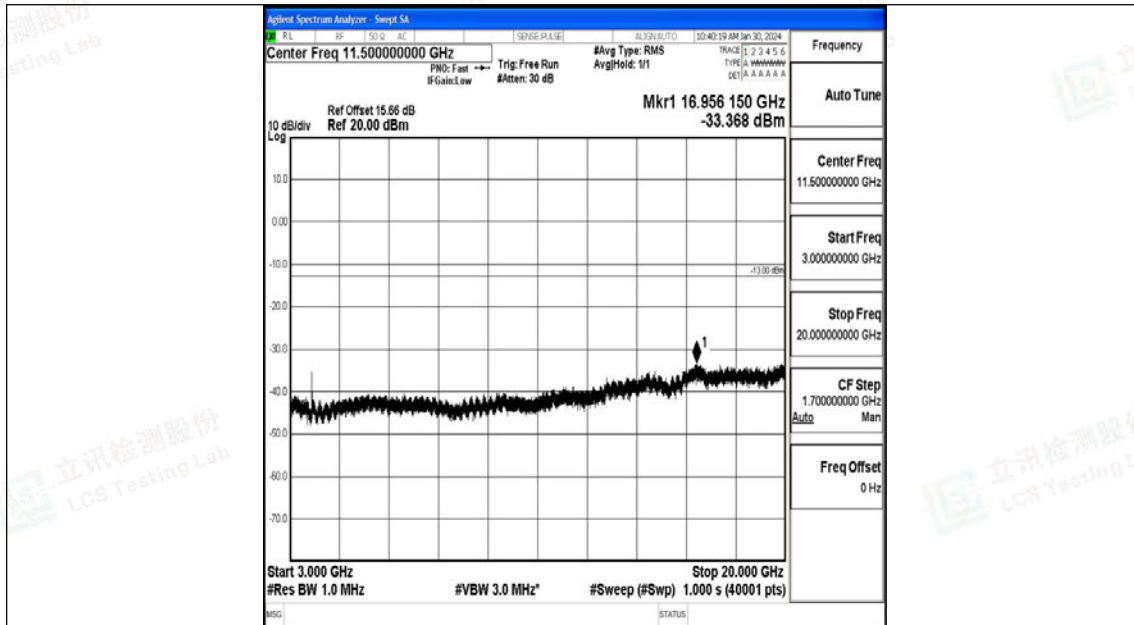
Band25_10MHz_QPSK_26365_1RB#0_3000~20000_3000~20000
