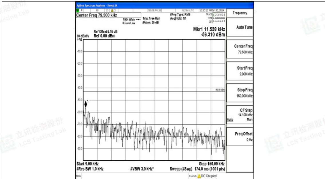
Band25_5MHz_QPSK_26665_1RB#0_0.009~0.15_0.009~0.15
