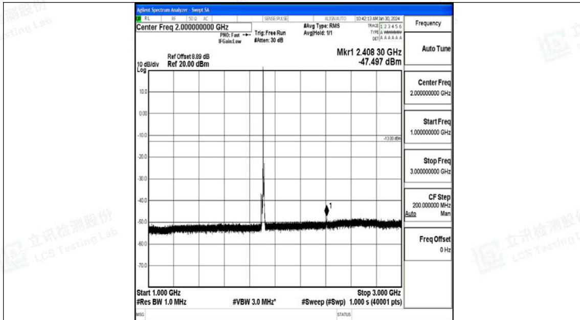
Band25_10MHz_16QAM_26640_1RB#0_1000~3000_1000~3000
