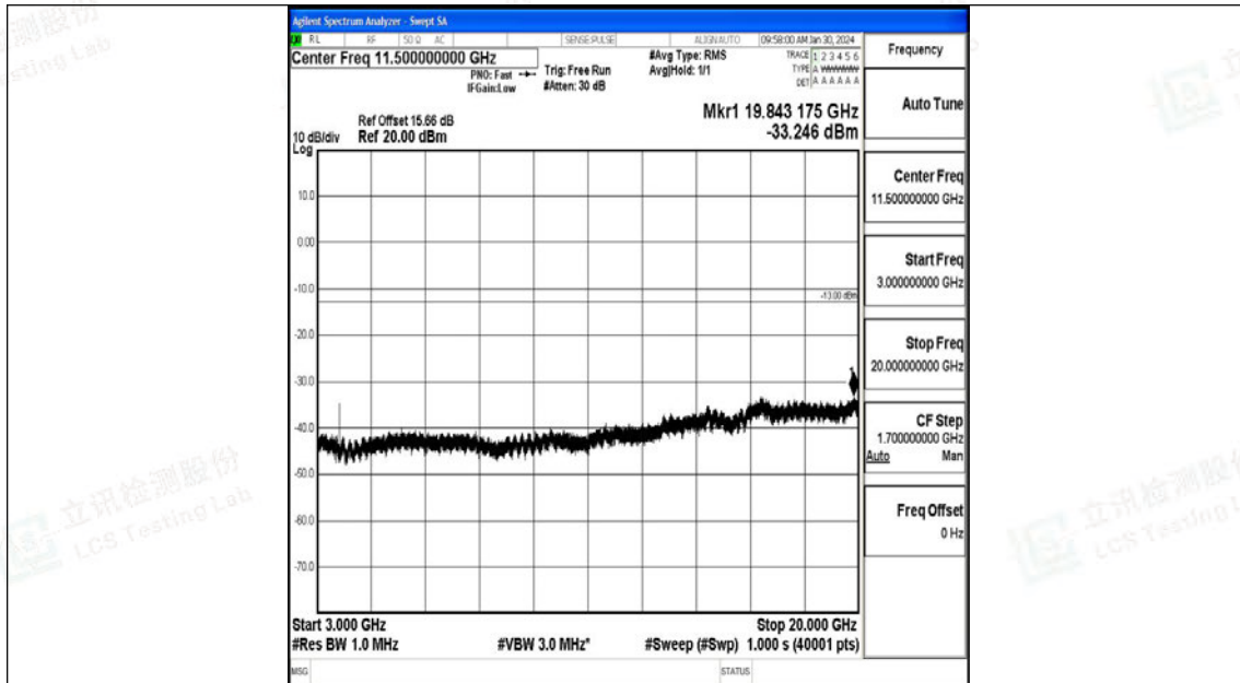
Band25_3MHz_QPSK_26055_1RB#0_3000~20000_3000~20000
