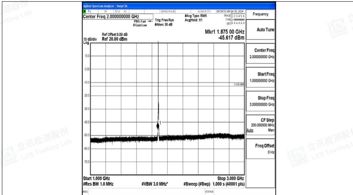
Band25_3MHz_16QAM_26365_1RB#0_1000~3000_1000~3000
