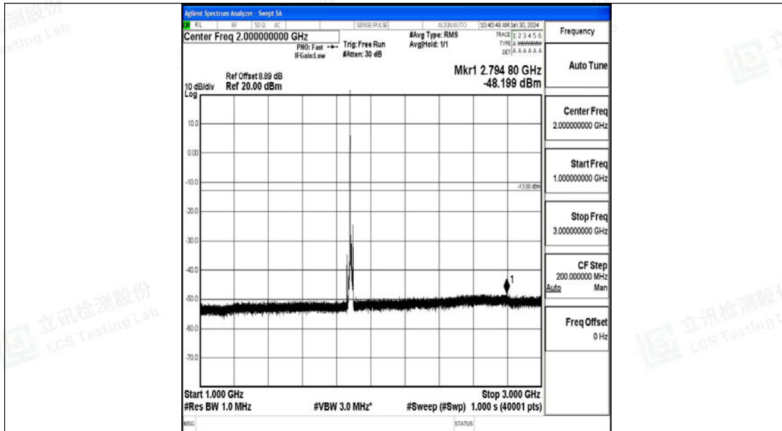
Band25_10MHz_16QAM_26365_1RB#0_1000~3000_1000~3000
