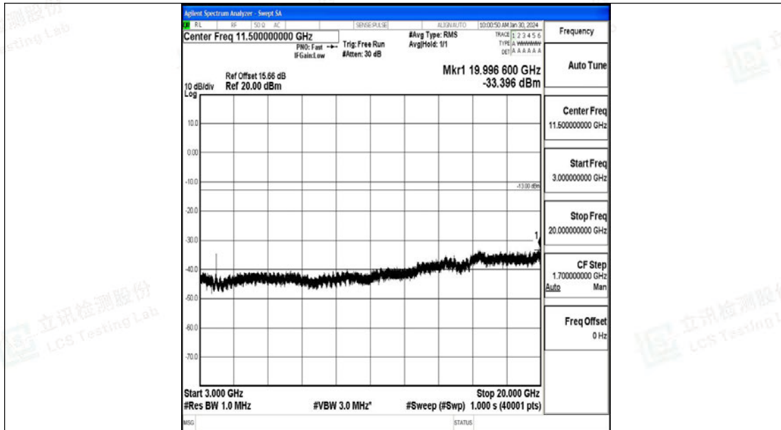
Band25_3MHz_QPSK_26675_1RB#0_3000~20000_3000~20000
