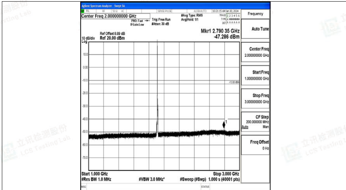
Band25_5MHz_16QAM_26665_1RB#0_1000~3000_1000~3000
