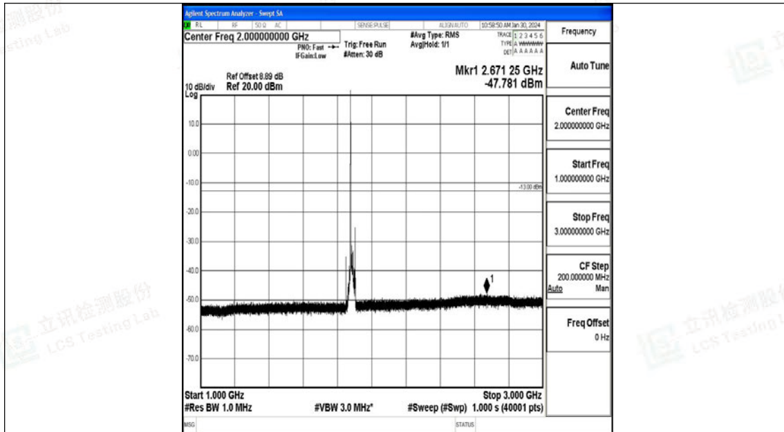
Band25_15MHz_16QAM_26365_1RB#0_1000~3000_1000~3000
