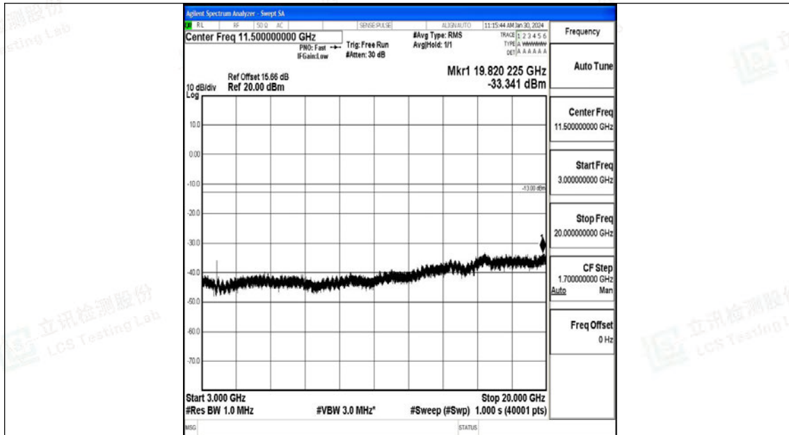
Band25_20MHz_QPSK_26365_1RB#0_3000~20000_3000~20000
