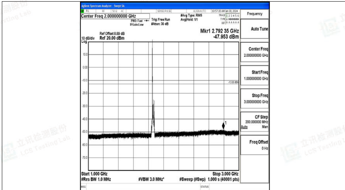
Band25_15MHz_16QAM_26115_1RB#0_1000~3000_1000~3000
