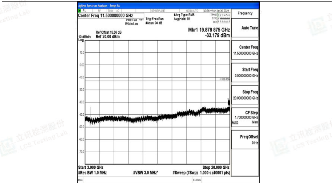
Band25_15MHz_QPSK_26115_1RB#0_3000~20000_3000~20000
