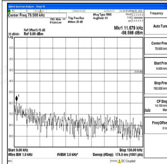
Band26_3MHz_QPSK_27025_1RB#0_0.009~0.15 5_0.009~0.15
