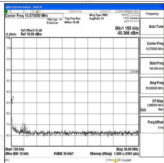
Band26_5MHz_QPSK_27015_1RB#0_0.15~30_0.15~30 15~30
