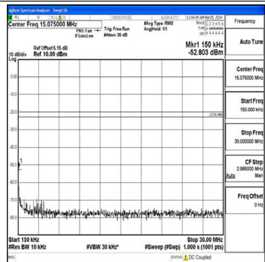
Band26_10MHz_QPSK_26840_1RB#0_0.15~30 0.15~30
