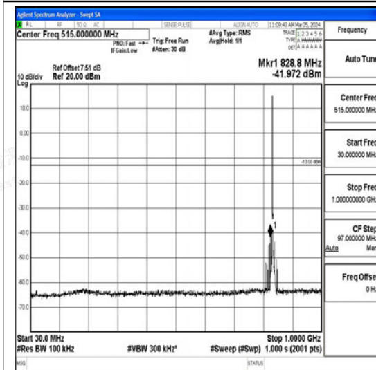
Band26_3MHz_QPSK_26915_1RB#0_30~1000_30~1000
