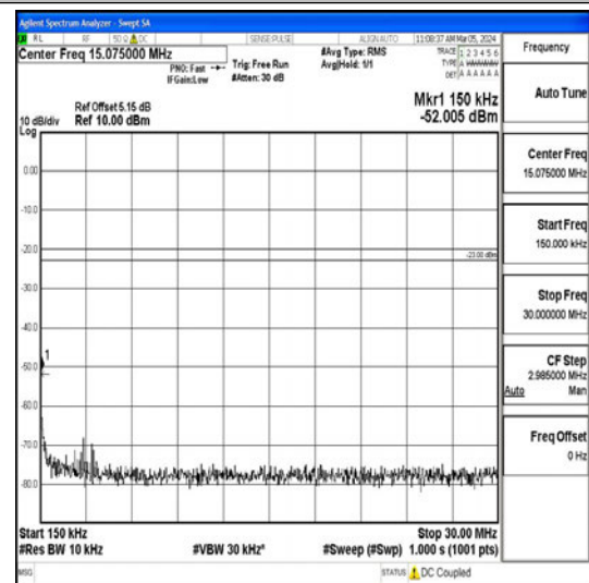
Band26_3MHz_QPSK_26805_1RB#0_0.15~30_0. 15~30
