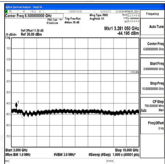
Band26_3MHz_16QAM_26915_1RB#0_3000~10000 00_3000~10000
