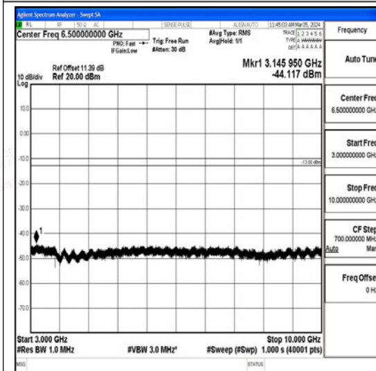
Band26_10MHz_QPSK_26840_1RB#0_3000~10000_000_3000~10000
