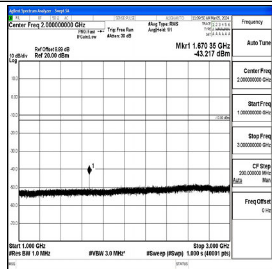
Band26_3MHz_QPSK_26915_1RB#0_1000~3000_1000~3000
