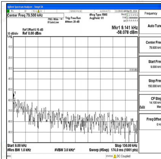
Band26_5MHz_QPSK_27015_1RB#0_0.009~0.15 5_0.009~0.15
