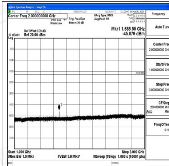
Band26_5MHz_16QAM_27015_1RB#0_1000~3000 00_1000~3000
