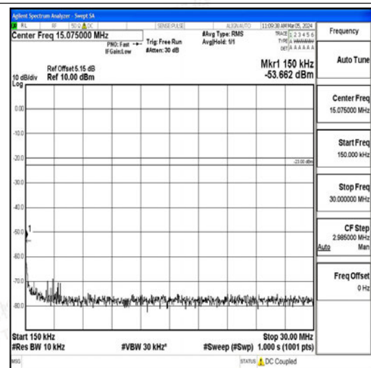
Band26_3MHz_QPSK_26915_1RB#0_0.15~30_0.15~30 15~30
