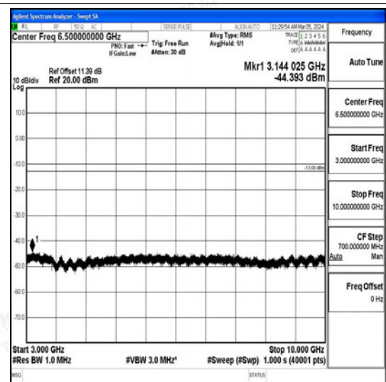
Band26_5MHz_16QAM_27015_1RB#0_3000~10000 00_3000~10000
