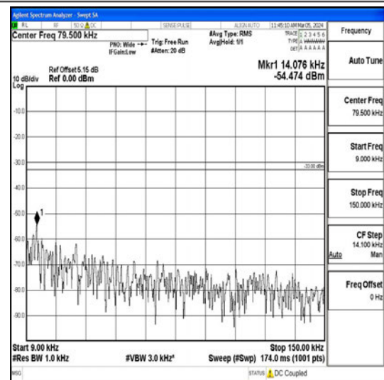
Band26_10MHz_16QAM_26840_1RB#0_0.009~0.15_0.009~0.15
