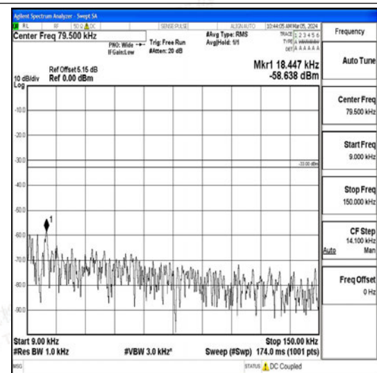
Band26_1.4MHz_16QAM_26797_1RB#0_0.009~0.15_0.009~0.15
