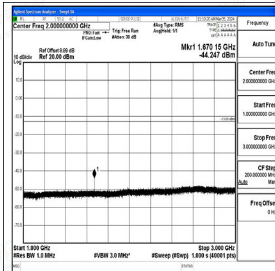
Band26_3MHz_16QAM_26915_1RB#0_1000~3000 00_1000~3000
