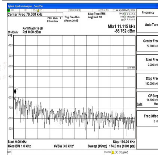
Band26_10MHz_QPSK_26840_1RB#0_0.009~0.15 15_0.009~0.15
