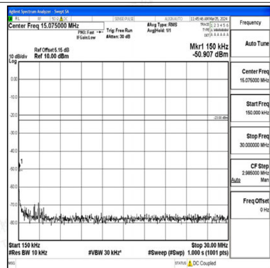
Band26_10MHz_QPSK_26915_1RB#0_0.15~30_0.15~30
