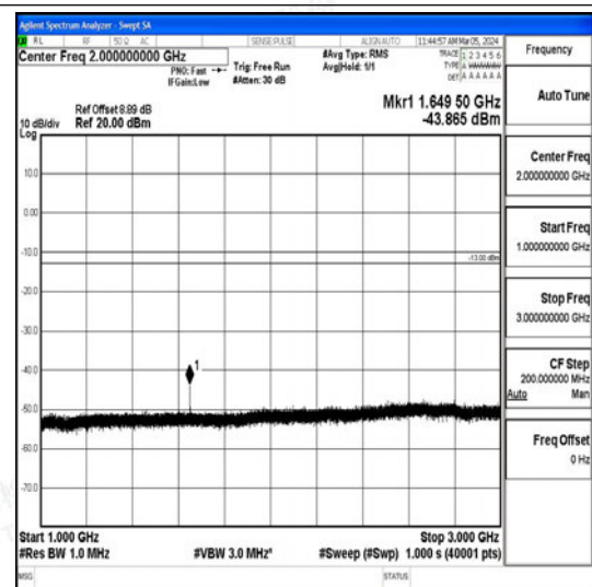
Band26_10MHz_QPSK_26840_1RB#0_1000~3000_0_1000~3000
