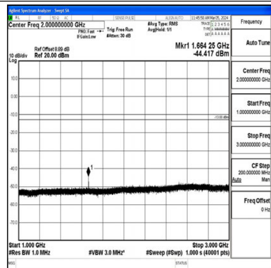
Band26_10MHz_QPSK_26915_1RB#0_1000~3000_0_1000~3000
