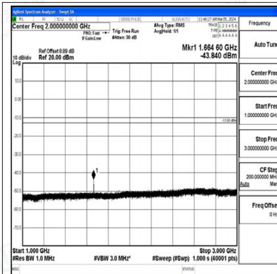
Band26_10MHz_16QAM_26915_1RB#0_1000~3000
