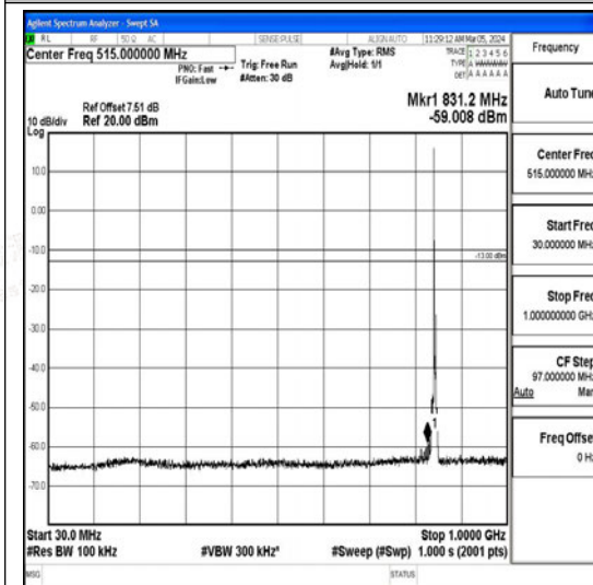
Band26_5MHz_QPSK_27015_1RB#0_30~1000_30~1000
