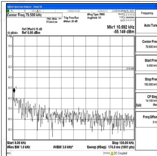
Band26_3MHz_QPSK_26915_1RB#0_0.009~0.15 5_0.009~0.15
