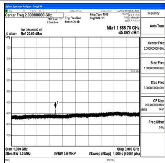
Band26_5MHz_QPSK_27015_1RB#0_1000~3000_1000~3000
