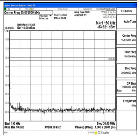
Band26_3MHz_QPSK_27025_1RB#0_0.15~30.0. 15~30
