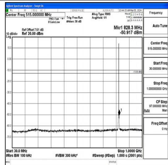
Band26_1.4MHz_16QAM_26797_1RB#0_0_30~1000_0_30~1000
