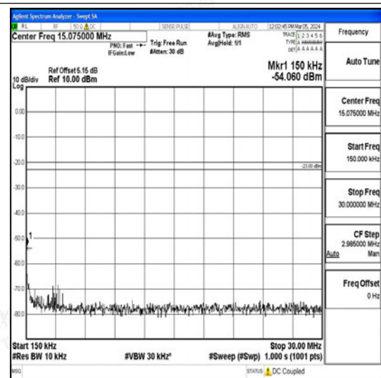
Band26_15MHz_QPSK_26965_1RB#0_0.15~30_0.15~30
