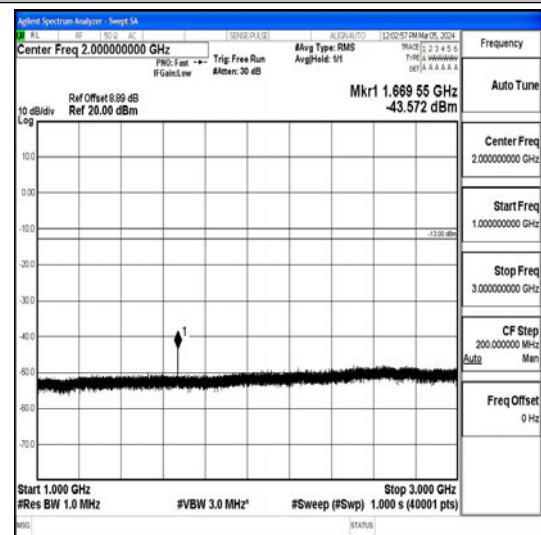
Band26_15MHz_QPSK_26965_1RB#0_1000~3000_0_1000~3000
