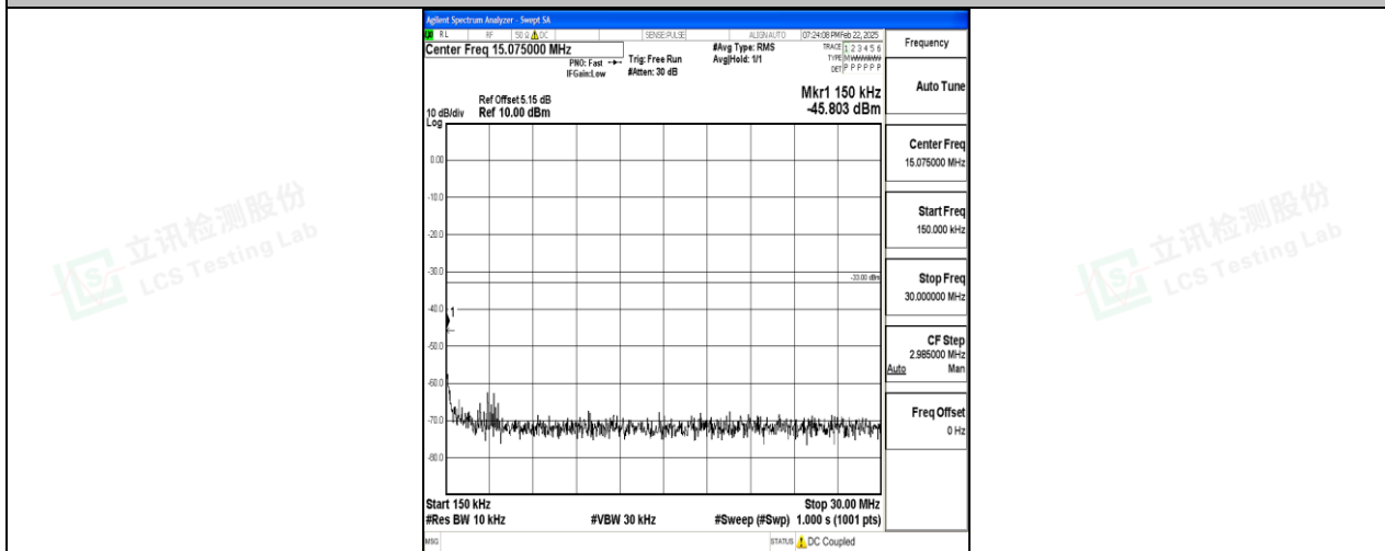
Band2_3MHz_QPSK_19185_1RB#0_0.15~30_0.15~30
