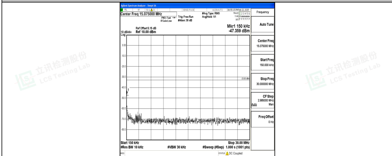
Band2_1.4MHz_16QAM_18607_1RB#0_0.15~30_0.15~30
