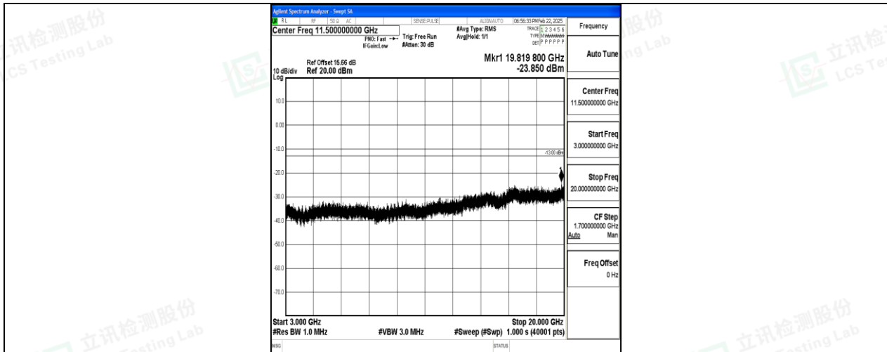
Band2_1.4MHz_16QAM_18900_1RB#0_3000~20000_3000~20000
