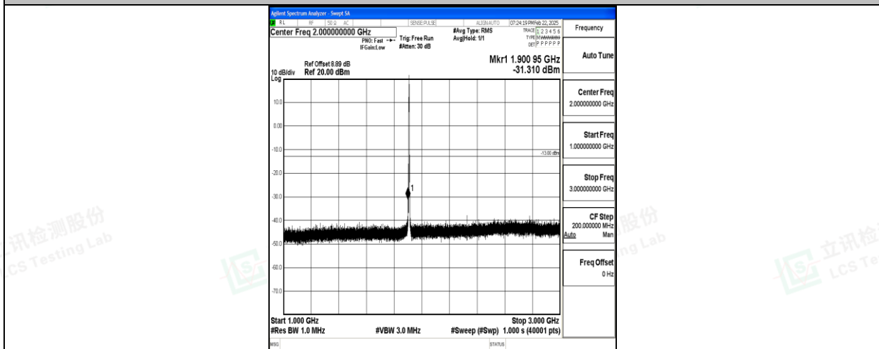
Band2_3MHz_QPSK_19185_1RB#0_1000~3000_1000~3000
