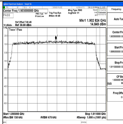
Band2_15MHz_QPSK_19125_75RB#0
