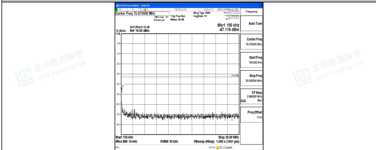
Band2_15MHz_16QAM_18675_1RB#0_0.15~30_0.15~30
