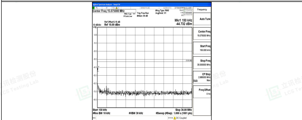
Band2_10MHz_QPSK_18900_1RB#0_0.15~30_0.15~30
