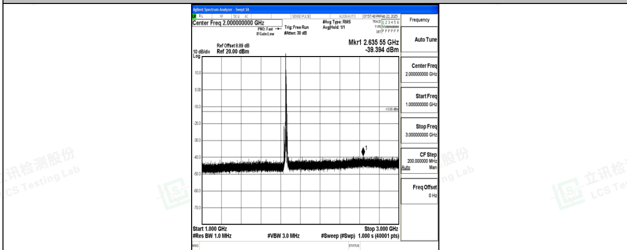
Band2_10MHz_16QAM_18650_1RB#0_1000~3000_1000~3000
