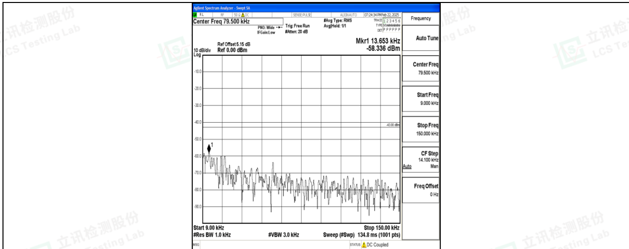
Band2_3MHz_16QAM_19185_1RB#0_0.009~0.15_0.009~0.15
