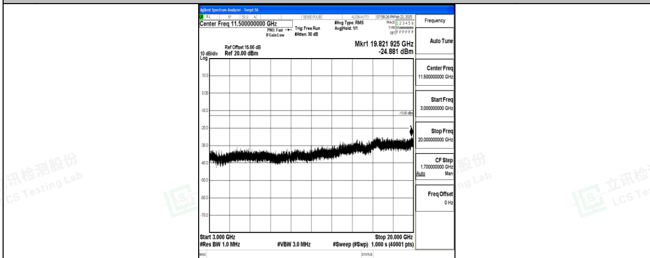
Band2_10MHz_QPSK_18900_1RB#0_3000~20000_3000~20000
