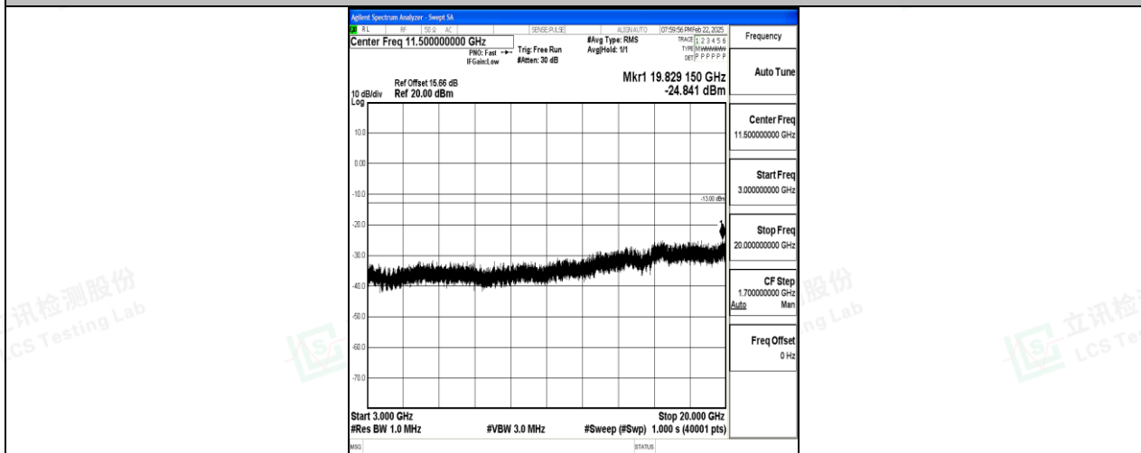
Band2_10MHz_16QAM_19150_1RB#0_3000~20000_3000~20000
