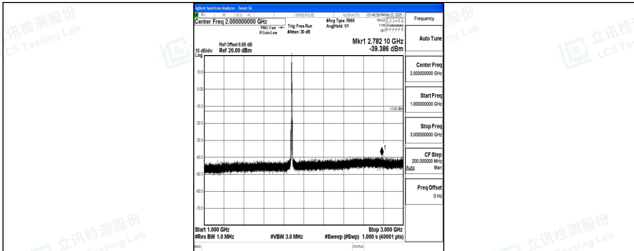
Band2_5MHz_QPSK_18900_1RB#0_1000~3000_1000~3000
