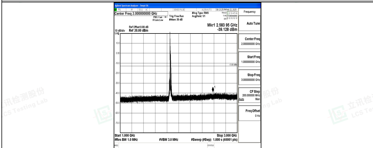
Band2_15MHz_16QAM_18675_1RB#0_1000~3000_1000~3000
