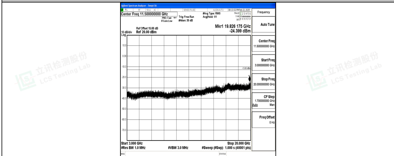
Band2_15MHz_16QAM_18675_1RB#0_3000~20000_3000~20000
