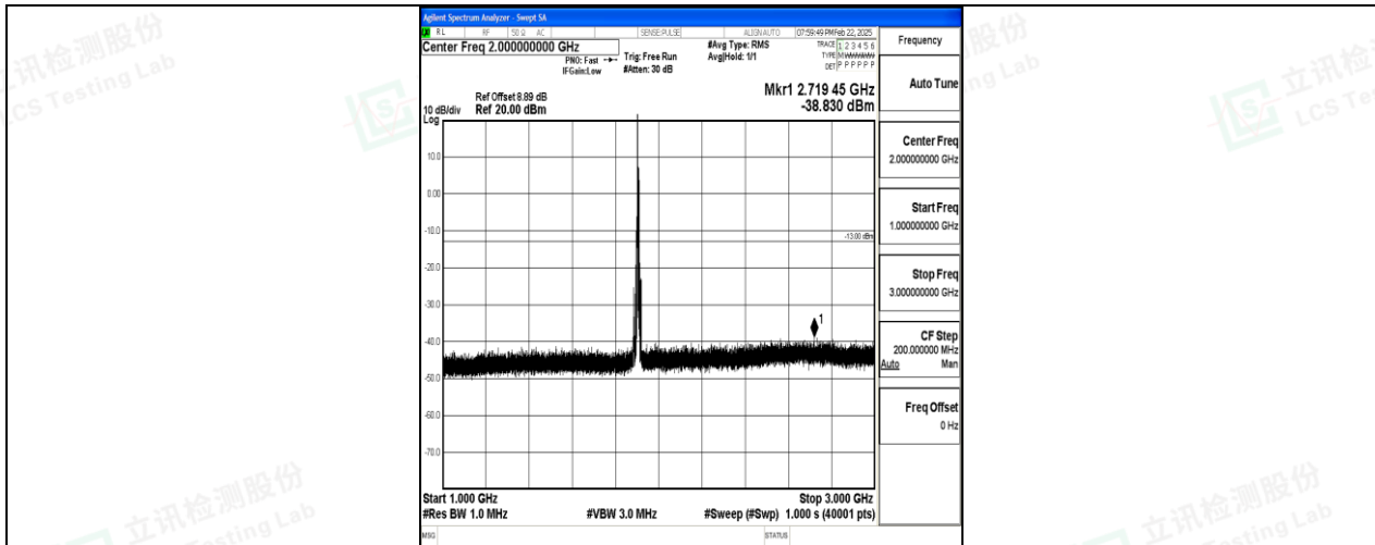
Band2_10MHz_16QAM_19150_1RB#0_1000~3000_1000~3000
