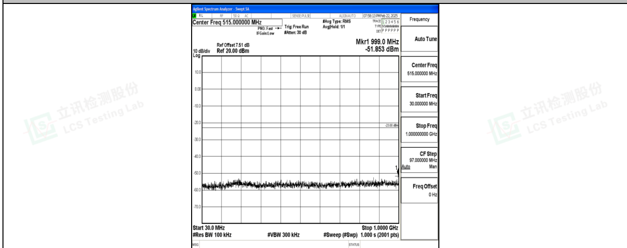
Band2_10MHz_QPSK_18900_1RB#0_30~1000_30~1000
