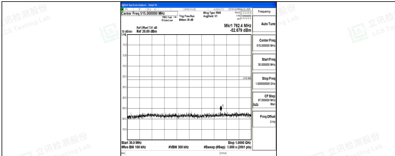
Band2_10MHz_16QAM_18650_1RB#0_30~1000_30~1000
