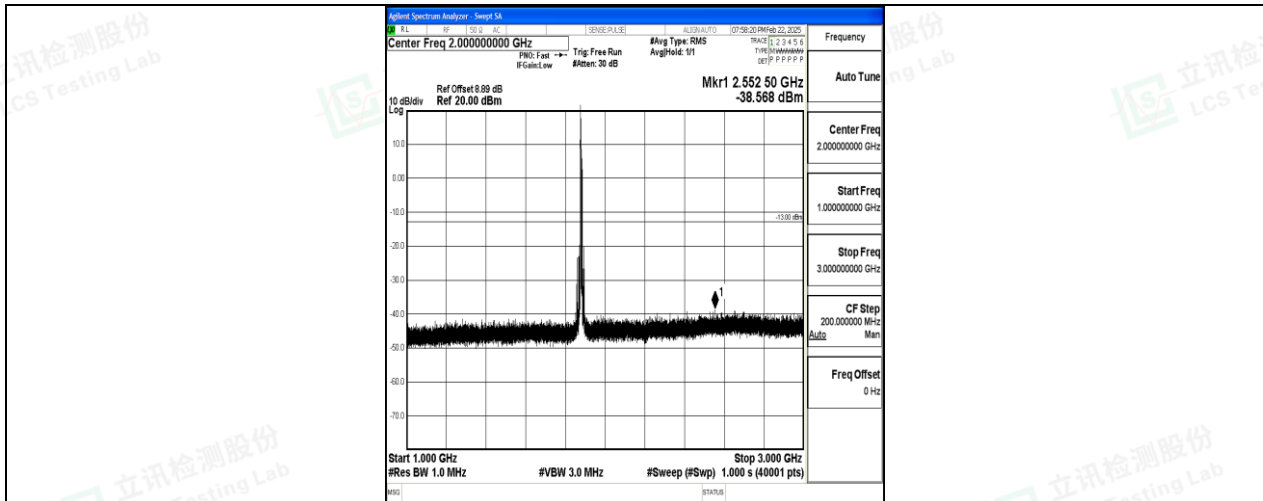
Band2_10MHz_QPSK_18900_1RB#0_1000~3000_1000~3000
