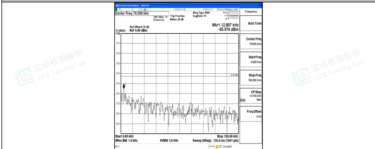
Band2_5MHz_16QAM_18900_1RB#0_0.009~0.15_0.009~0.15
