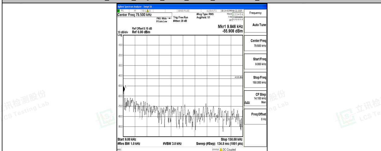
Band2_15MHz_QPSK_19125_1RB#0_0.009~0.15_0.009~0.15
