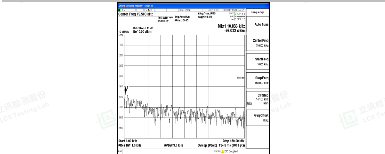
Band2_15MHz_16QAM_18675_1RB#0_0.009~0.15_0.009~0.15
