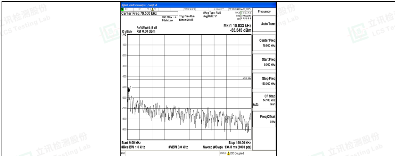
Band2_10MHz_QPSK_18900_1RB#0_0.009~0.15_0.009~0.15
