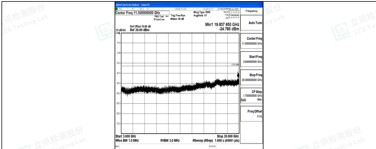
Band2_5MHz_QPSK_18625_1RB#0_3000~20000_3000~20000
