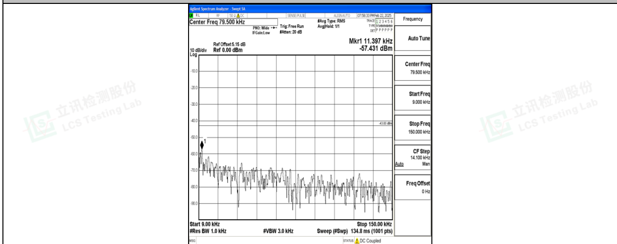
Band2_10MHz_16QAM_18900_1RB#0_0.009~0.15_0.009~0.15
