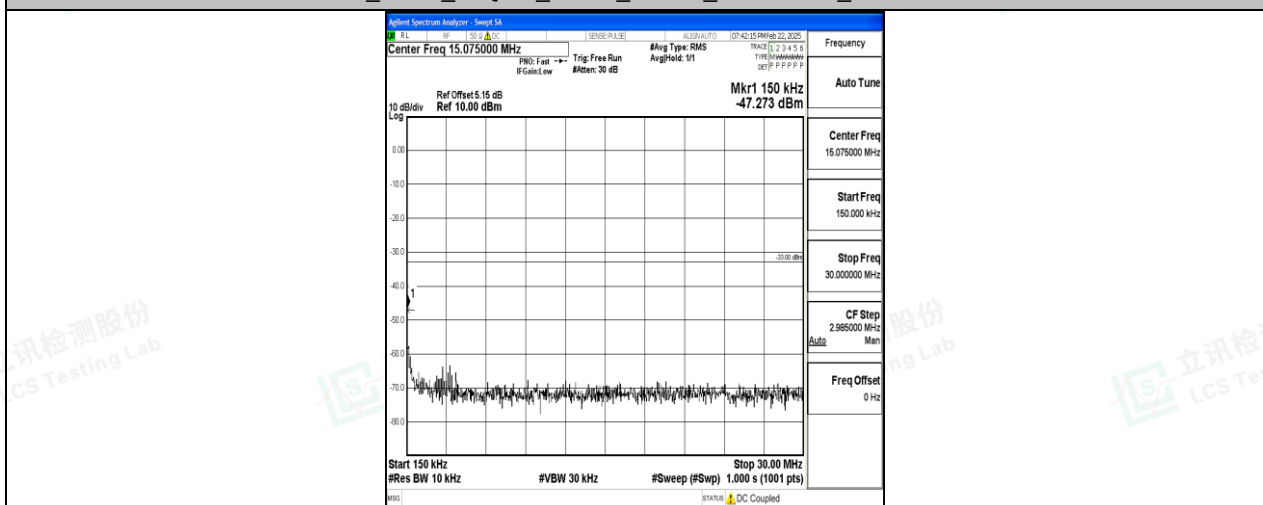
Band2_5MHz_16QAM_19175_1RB#0_0.15~30_0.15~30
