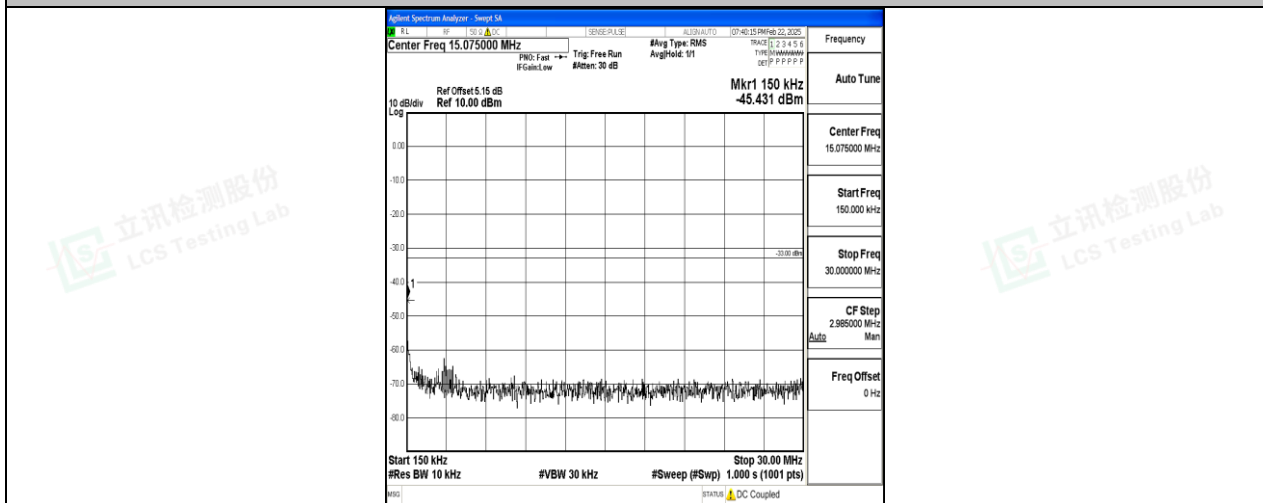
Band2_5MHz_16QAM_18625_1RB#0_0.15~30_0.15~30
