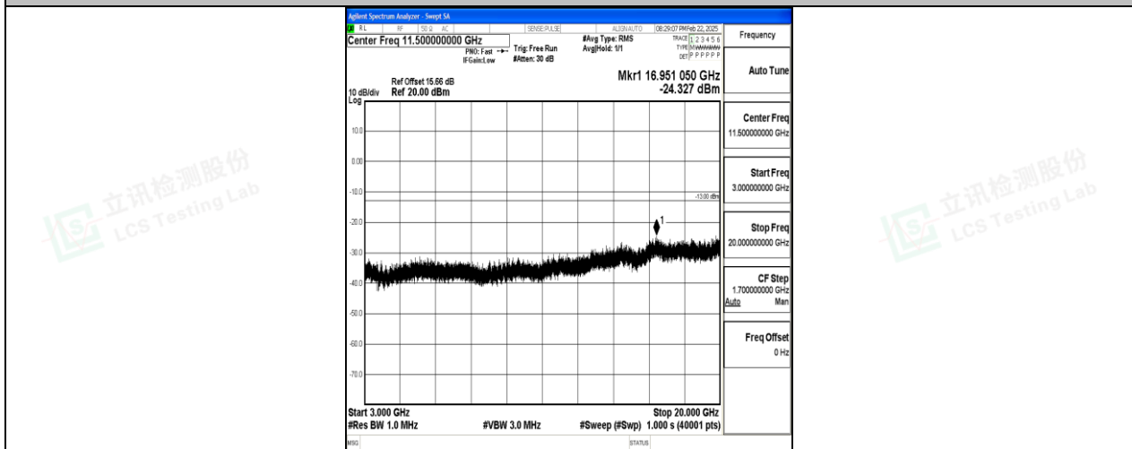
Band2_20MHz_16QAM_18700_1RB#0_3000~20000_3000~20000
