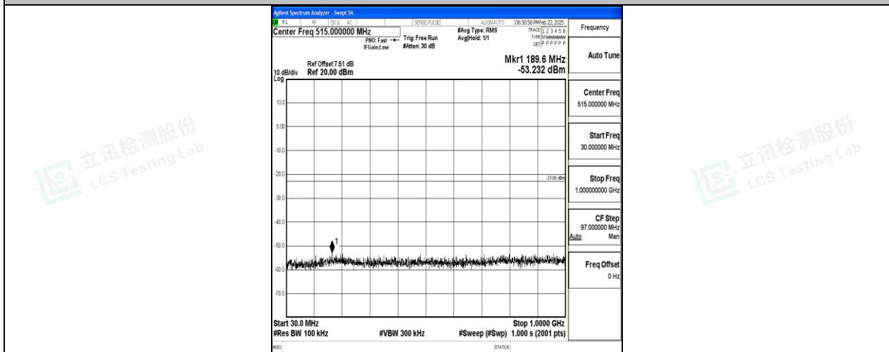
Band2_20MHz_16QAM_19100_1RB#0_30~1000_30~1000
