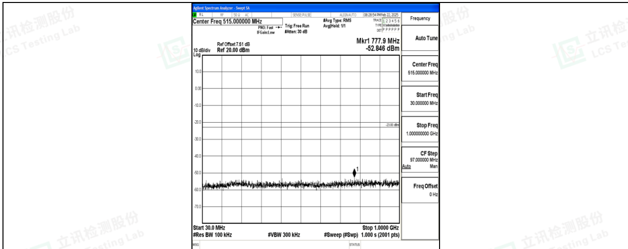
Band2_20MHz_16QAM_18700_1RB#0_30~1000_30~1000
