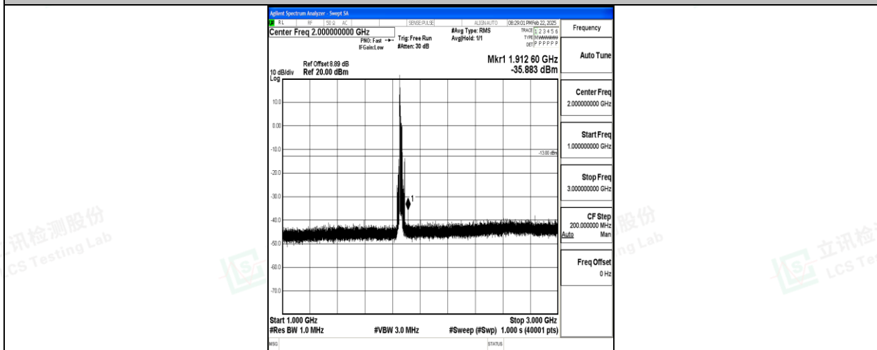
Band2_20MHz_16QAM_18700_1RB#0_1000~3000_1000~3000
