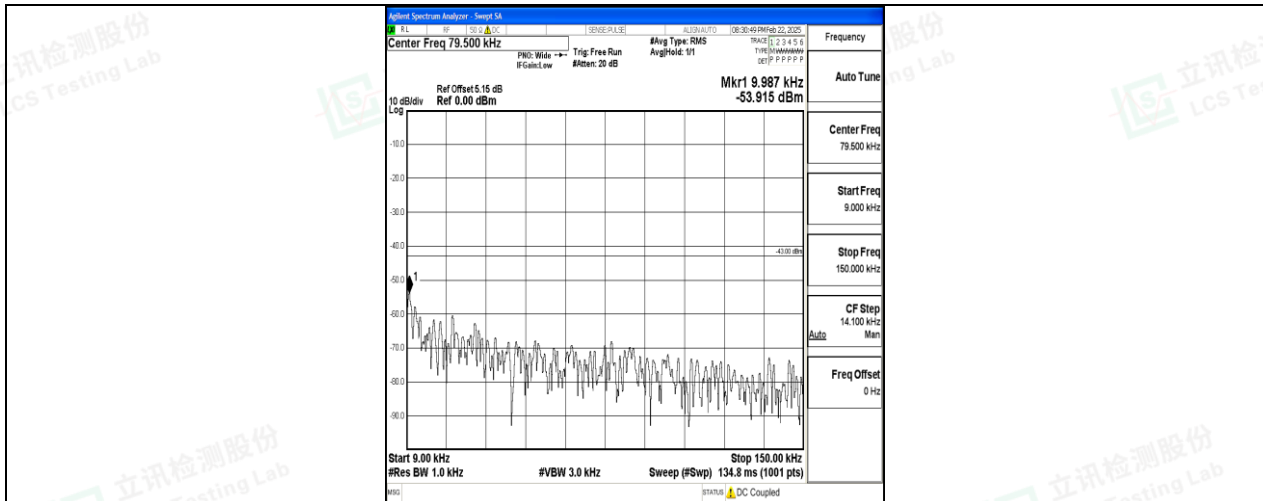
Band2_20MHz_16QAM_19100_1RB#0_0.009~0.15_0.009~0.15
